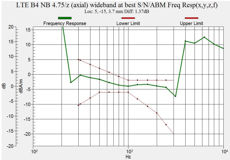
Frequency Response of Ant.2 LTE Band 4
