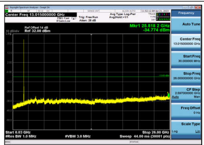
FDD04_LowRange_20MHz_30MHz~26GHz
