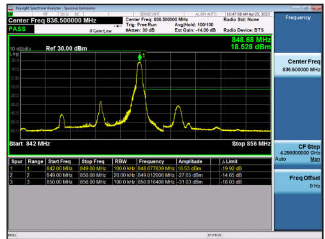
FDD5-5MHz-16QAM-HCH-25RB#0
