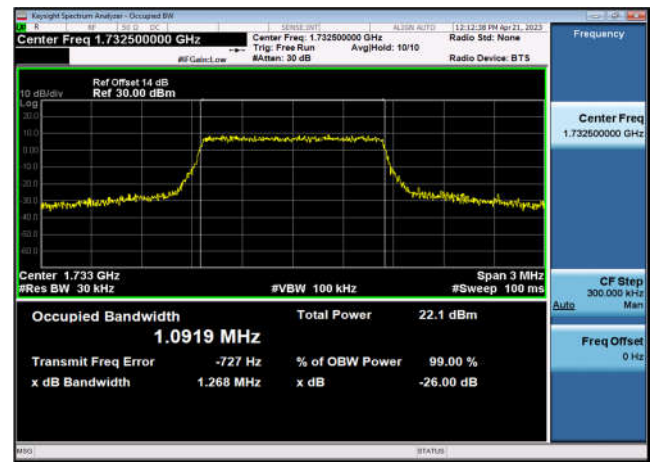
FDD04_MidRange_3_1732.5_Q16
