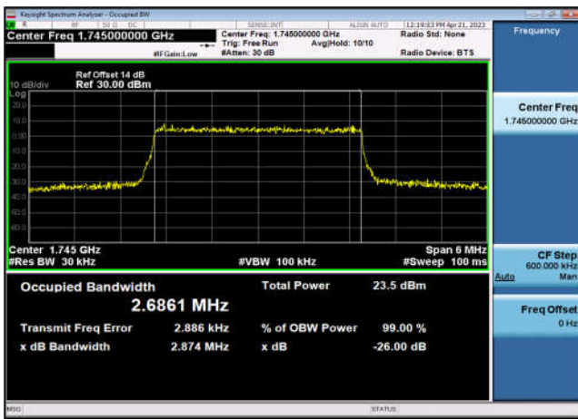
FDD66_MidRange_5_1745_QPSK
