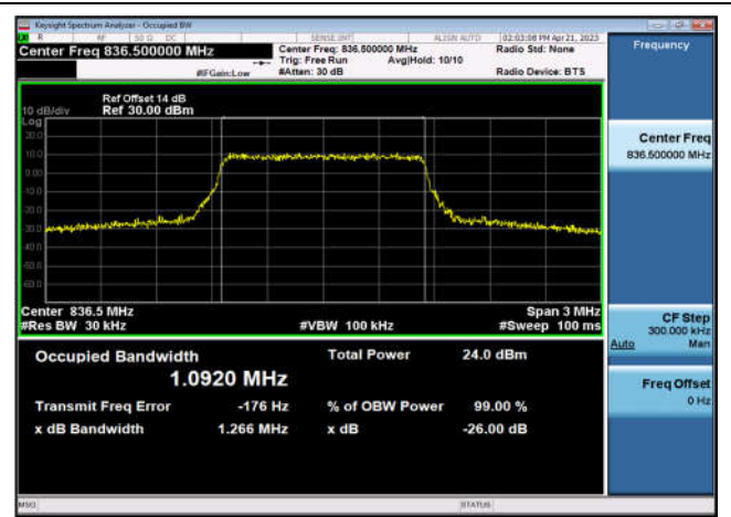
FDD05_MidRange_3_836.5_Q16
