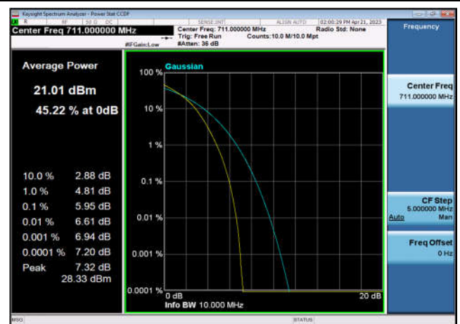
FDD12_HighRange_10MHz_711_fullRB_Q16
