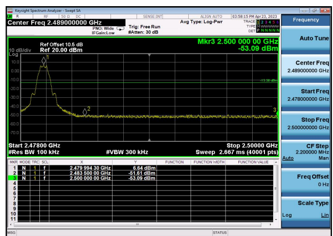
,Plot ,3Transmitter Spurious Emission
