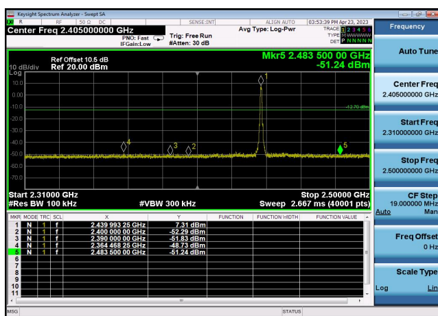
,Plot ,3Transmitter Spurious Emission
