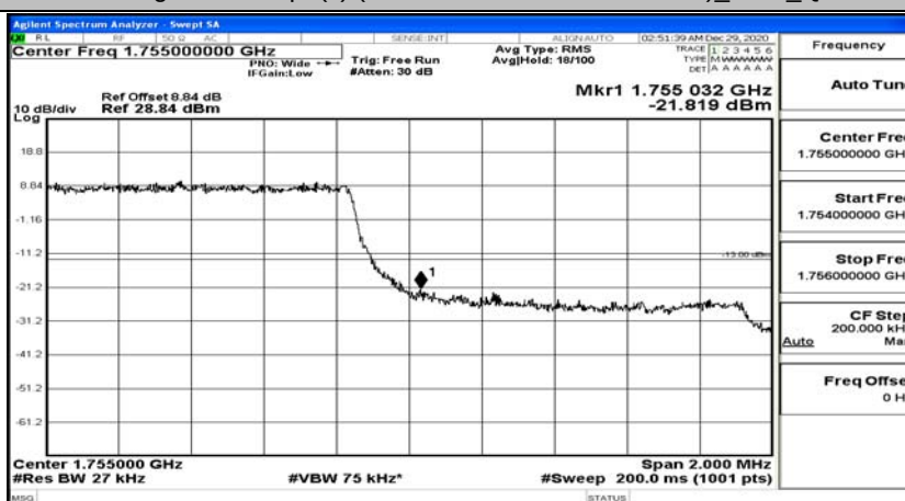
Band Edge Test Graph(s) (Channel Bandwidth: 1.4 MHz) HCH QPSK
