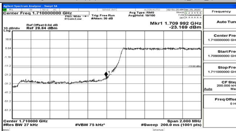
Band Edge Test Graph(s) (Channel Bandwidth: 1.4 MHz) LCH QPSK
