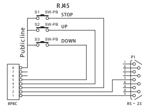
Connection diagram
