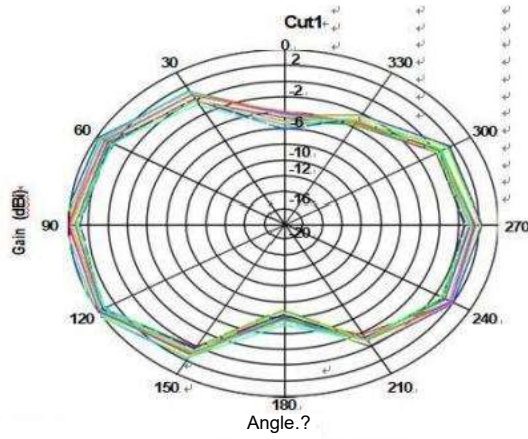
Horizontal X-Y
