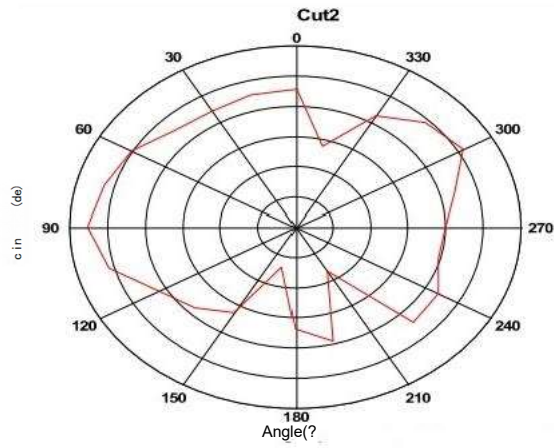
Horizontal X-Z
