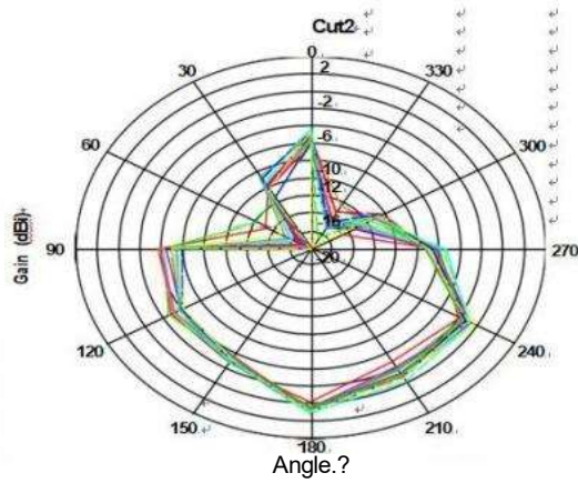
Horizontal X-Z
