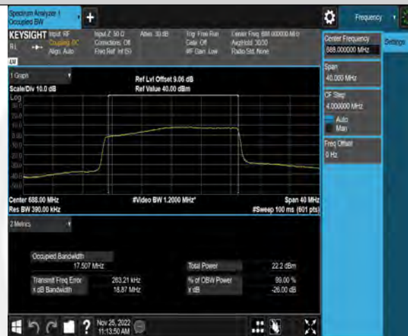
Band71-20MHz-16QAM-133222-100RB#0
