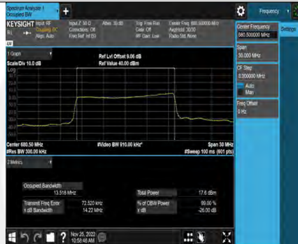
Band71-15MHz-16QAM-133397-75RB#0
