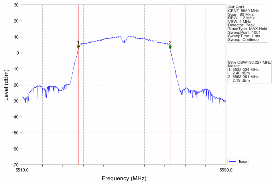
802.11n(HT40)_MCH_5550MHz_Ant1_NTN
