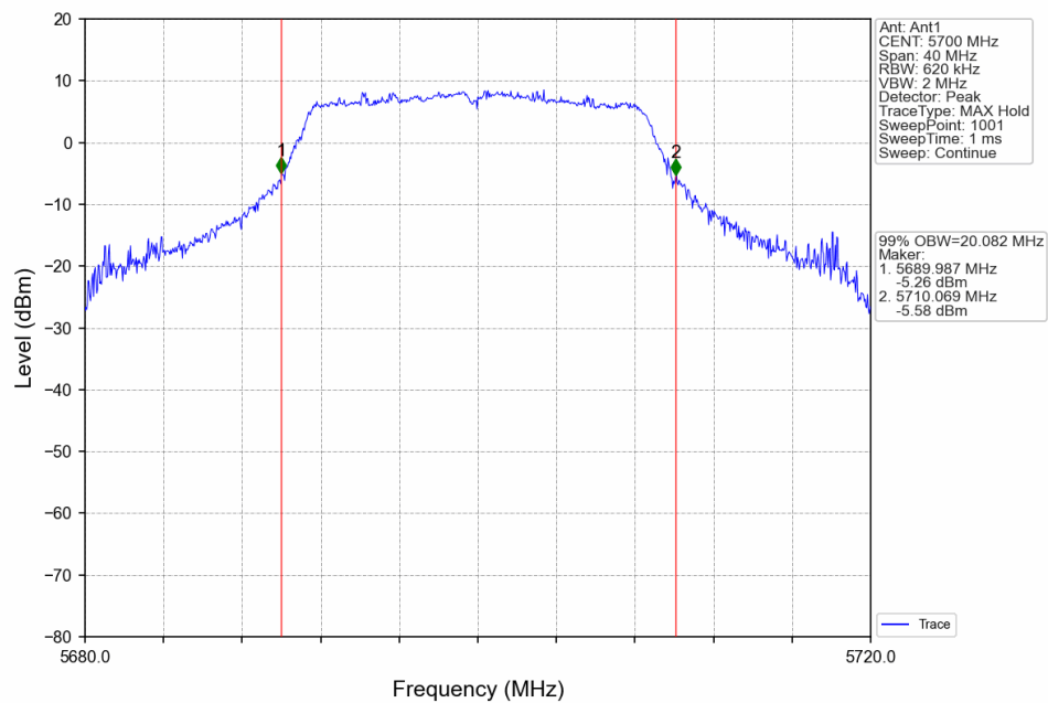
802.11n(HT20)_HCH_5700MHz_Ant1_NTN
