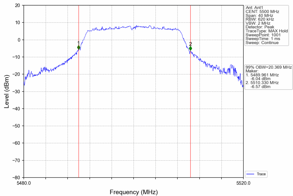
802.11ac(VHT20)_LCH_5500MHz_Ant1_NTN
