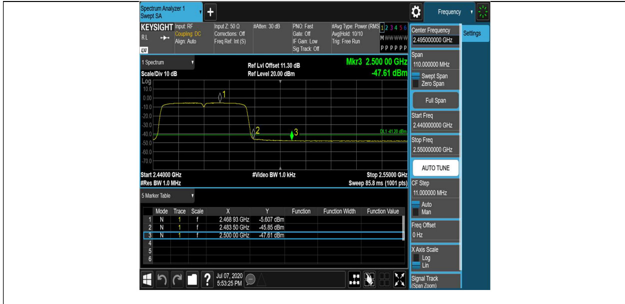
11N40SISO_Ant1_High_2452_Peak
