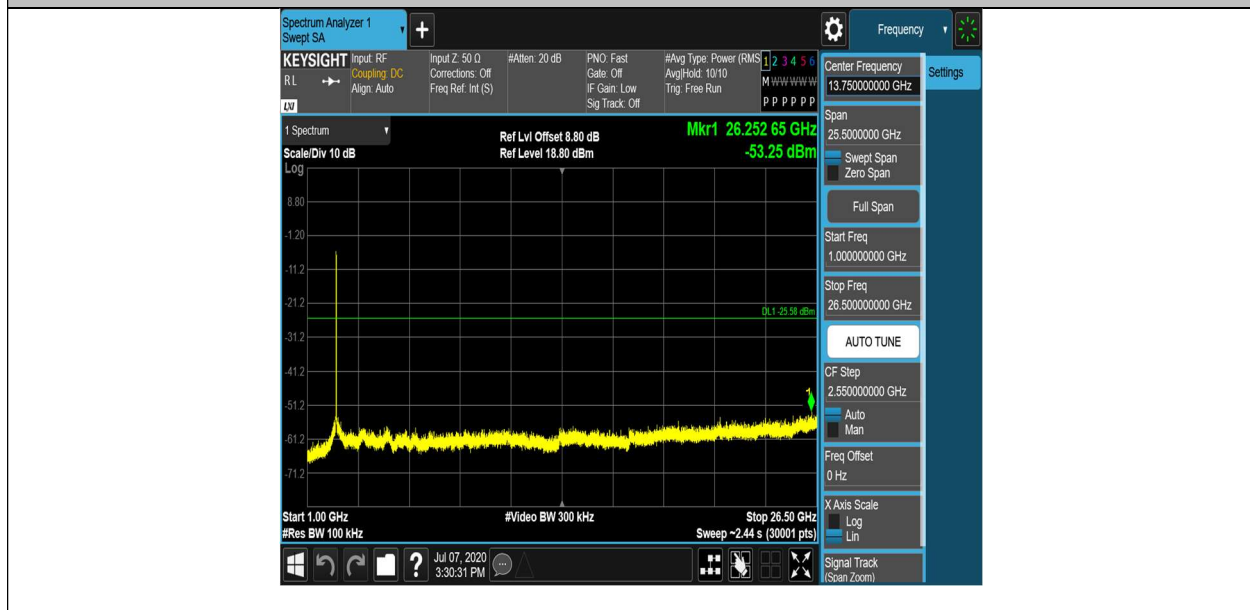
11G_Ant1_2462_0~Reference
