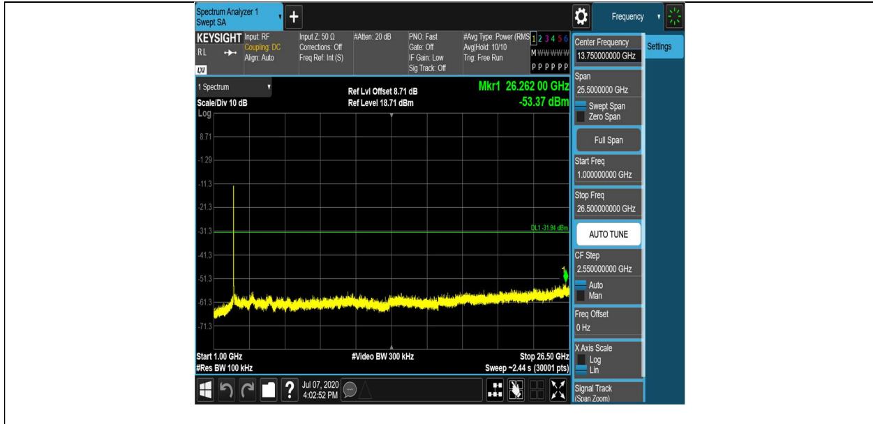
11N40SISO_Ant1_2437_0~Reference
