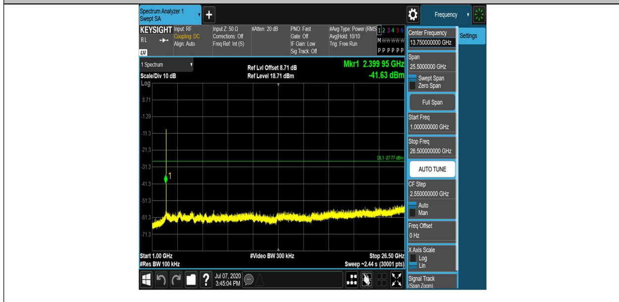
11N20SISO_Ant1_2437_0~Reference
