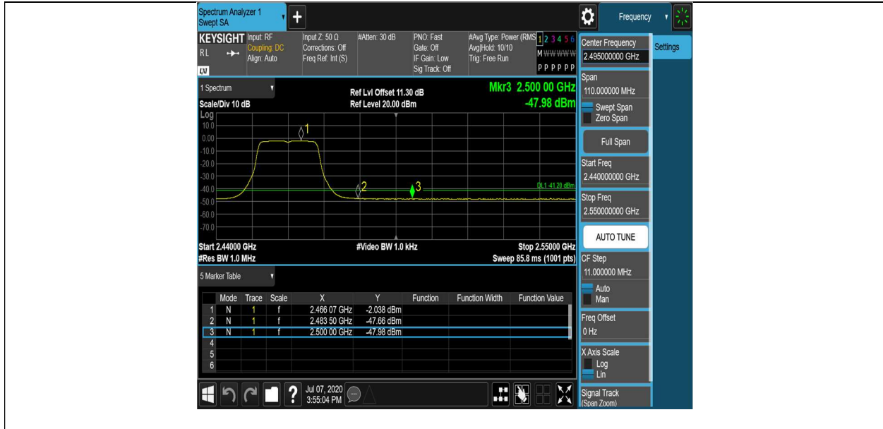
11N20SISO_Ant1_High_2462_Peak
