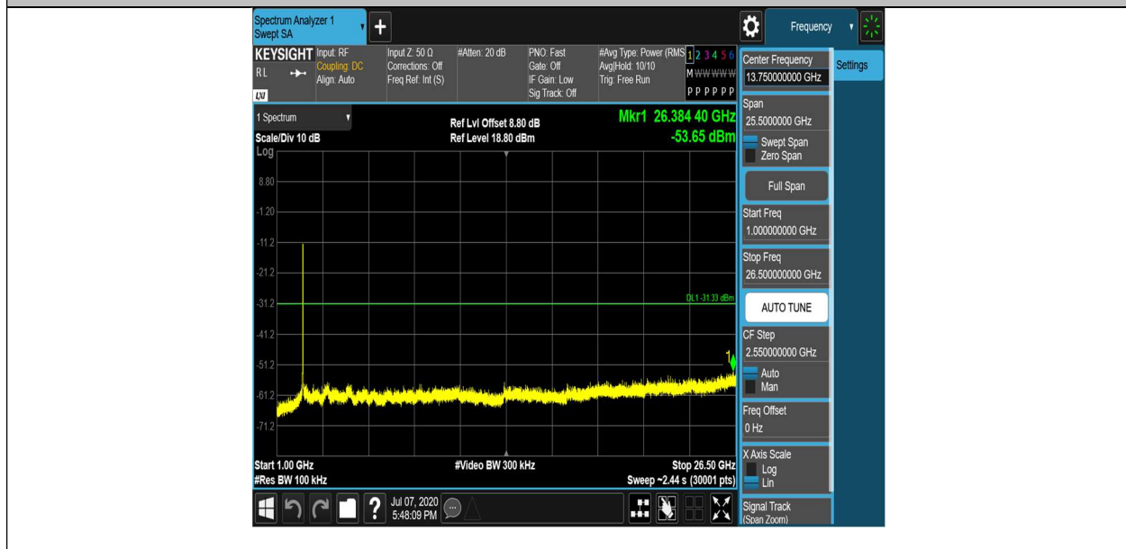
11N40SISO_Ant1_2452_0~Reference
