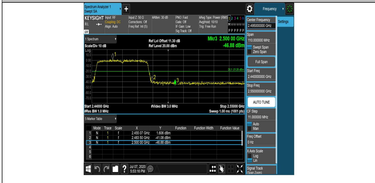
11N40SISO_Ant1_High_2452_Peak
