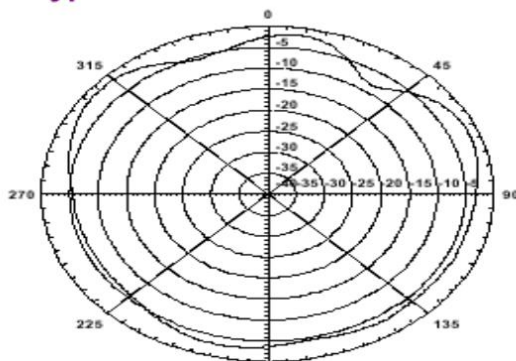
Typical H-Plane Antenna Pattern
