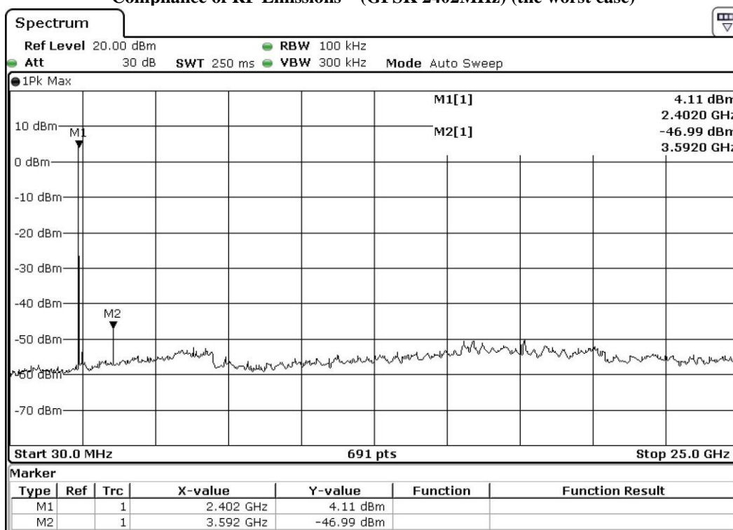
Compliance of RF Emissions – (GFSK 2402MHz) (the worst case)
