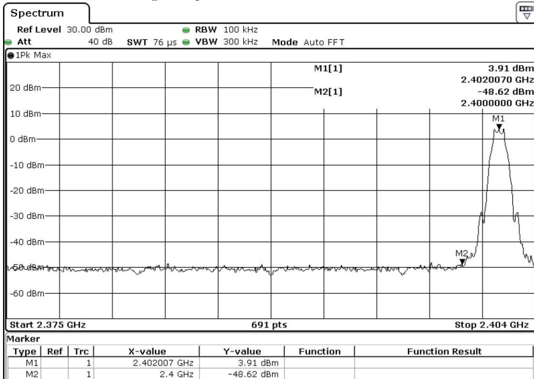
Band-edge Compliance of RF Emissions – Lowest (GFSK)
