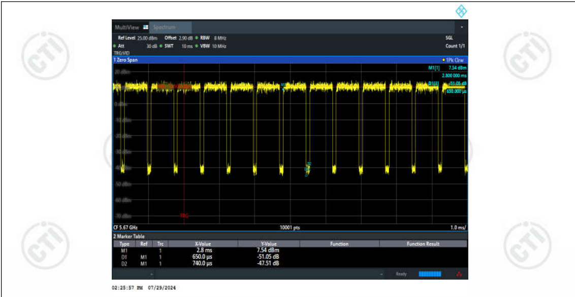
11N40SISO_Ant2_5670
