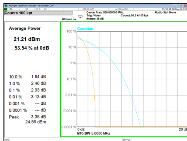
WCDMA B5_Middle
