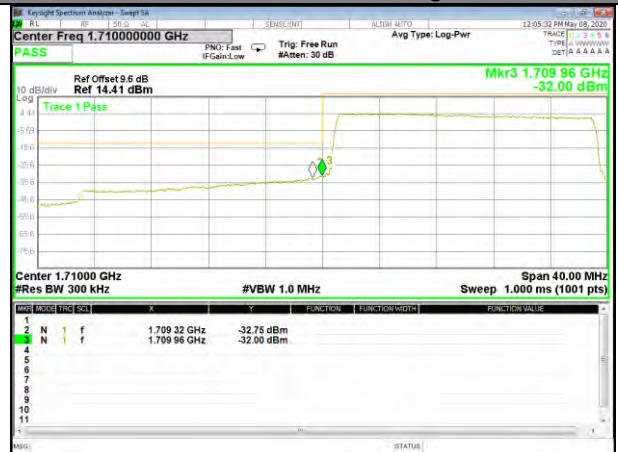
QPSK_20M_Lower_Band edge_Full-RB
