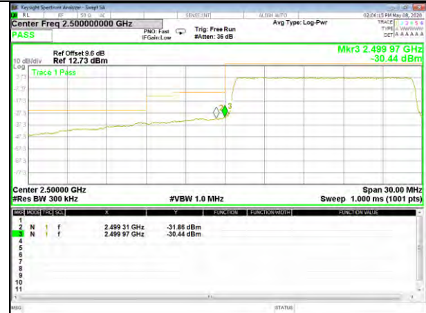
B7_Q16_15M_Low_Full-RB_Bedge
