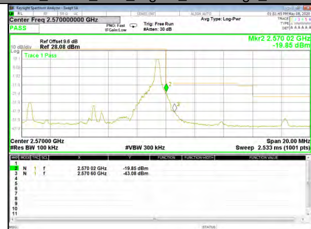
B7_QPSK_10M_Higher_Band edge_1-RB
