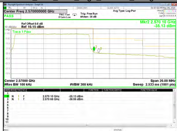
B7_Q16_10M_High_Full-RB_Bedge
