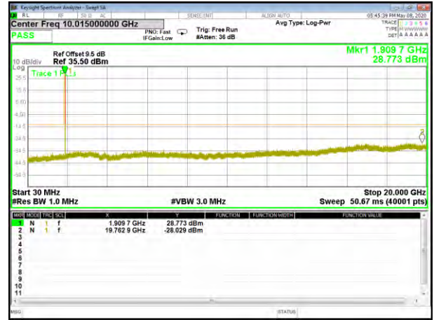
EGPRS_1900_Higher Conducted Spurious
