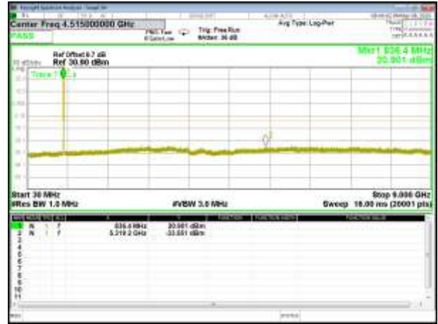
WCDMA B5_Conducted Spurious_Middle
