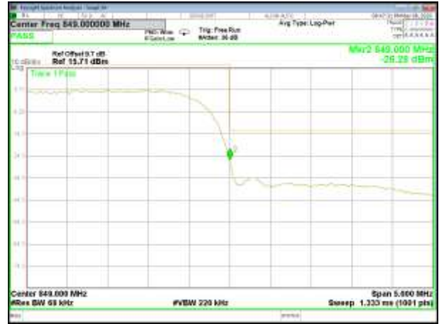
WCDMA B5_Band edge_High
