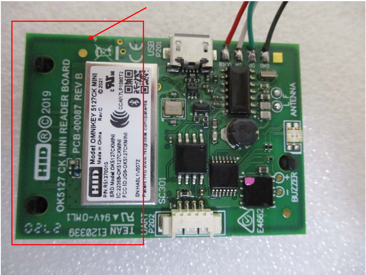
< RFID 2(HID) -13.56 MHz Antenna >
