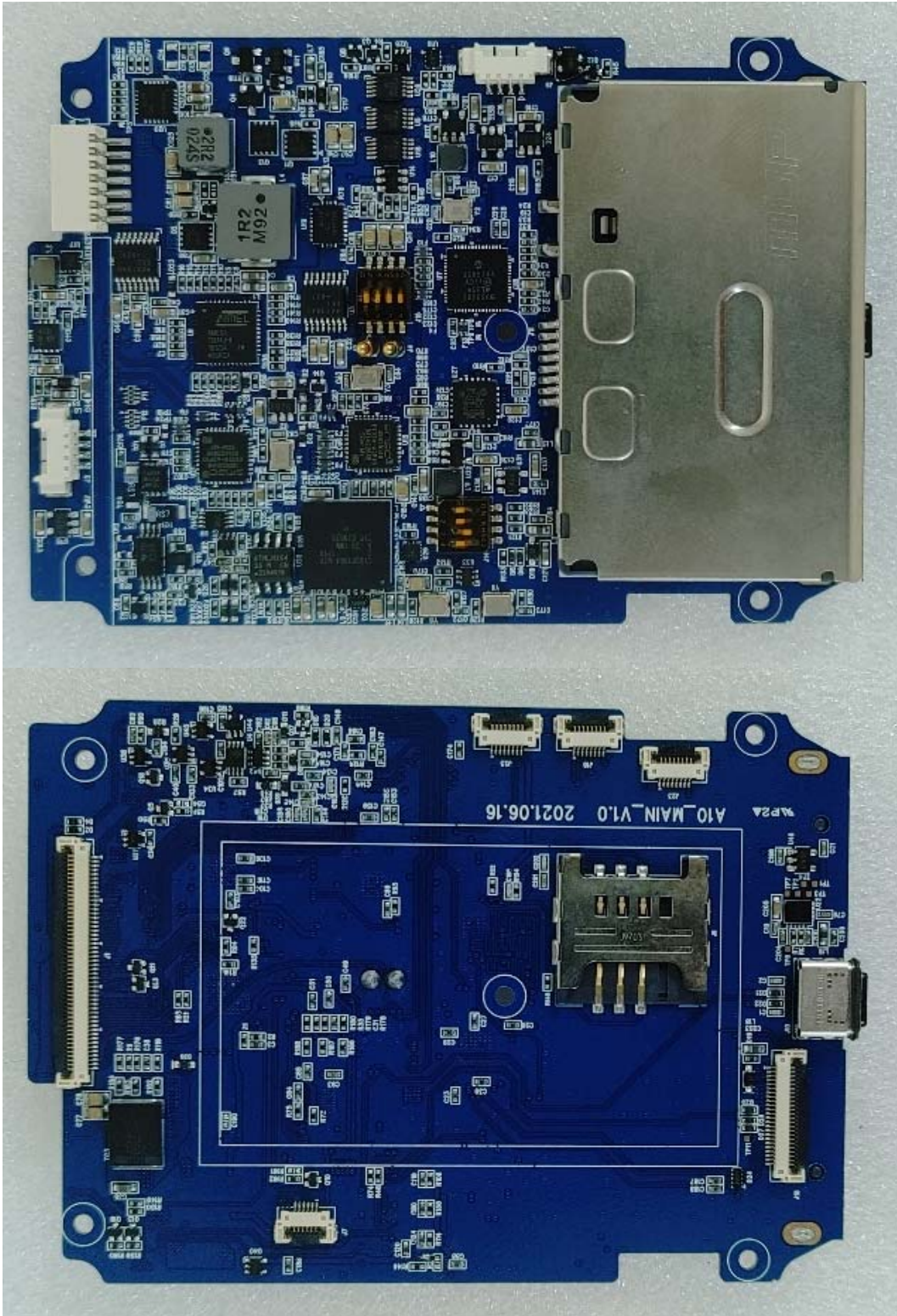
< Main board >
