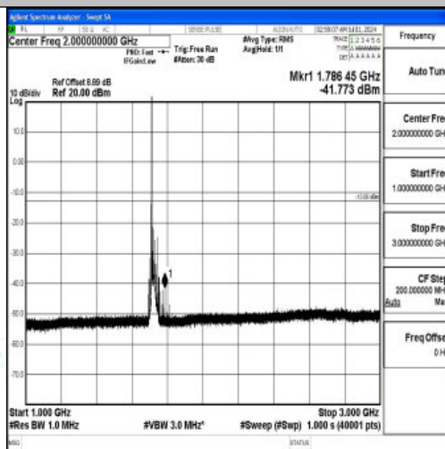
Band66_20MHz_16QAM_132072_1RB#0_1000~3000_1000~3000
