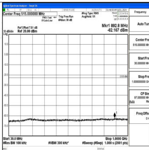
Band66 5MHz 16QAM 131997 1RB#0 30~1000 30~1000
