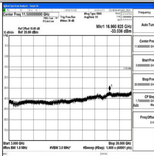
Band66_5MHz_QPSK_132647_1RB#0_3000~20000_3000~20000
