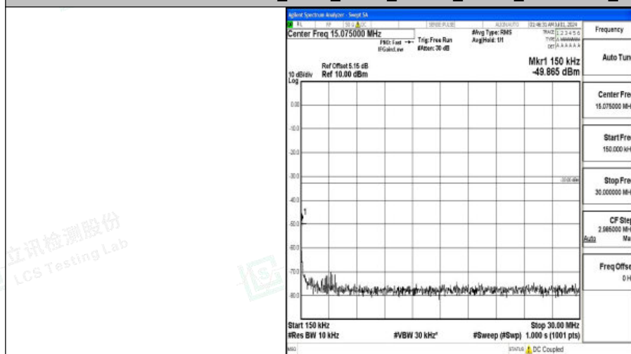
Band66_5MHz_QPSK_132322_1RB#0_0.15~30_0.15~30
