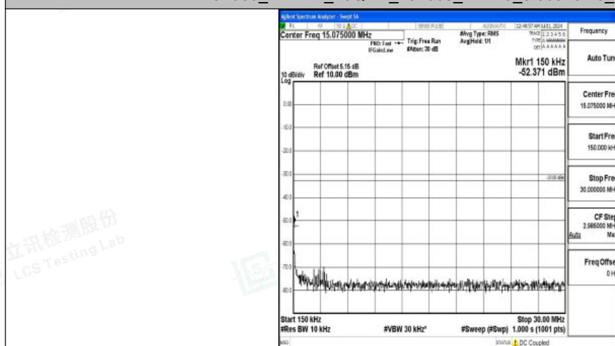
Band66_1.4MHz_16QAM_132665_1RB#0_0.15~30_0.15~30
