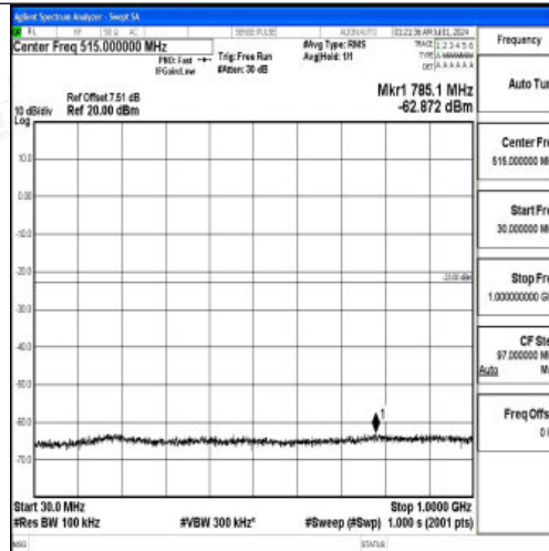
Band66_3MHz_QPSK_132657_1RB#0_30~1000_30~1000
