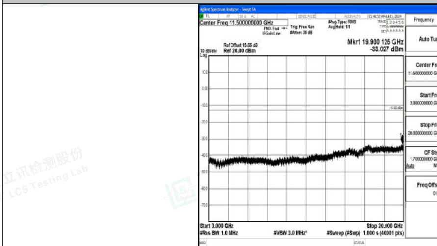
Band66_5MHz_QPSK_132322_1RB#0_3000~20000_3000~20000
