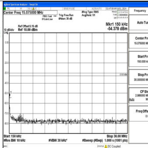
Band66_5MHz_16QAM_132322_1RB#0_0.15~30_0.15~30
