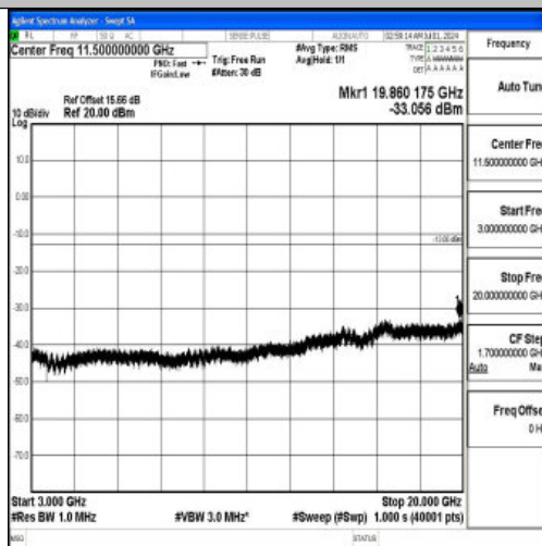
Band66_20MHz_16QAM_132072_1RB#0_3000~20000_3000~20000
