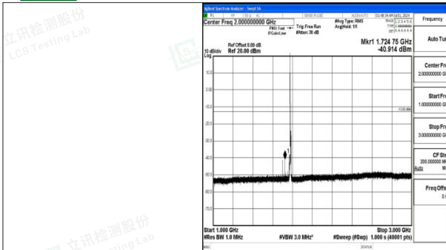
Band66_5MHz_16QAM_132647_1RB#0_1000~3000_1000~3000
