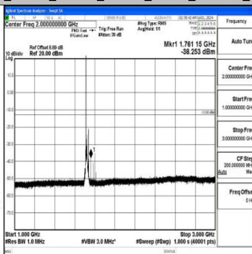
Band66_15MHz_16QAM_132047_1RB#0_1000~3000_1000~3000
