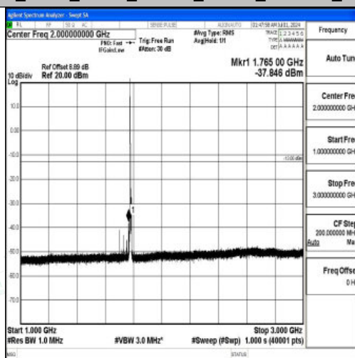
Band66_5MHz_QPSK_132647_1RB#0_1000~3000_1000~3000
