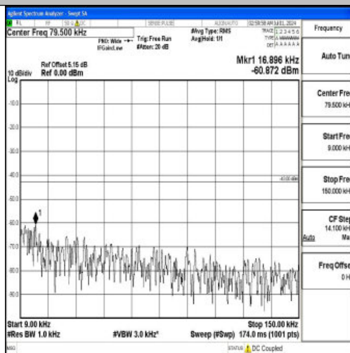
Band66_20MHz_16QAM_132322_1RB#0_0.009~0.15_0.009~0.15
