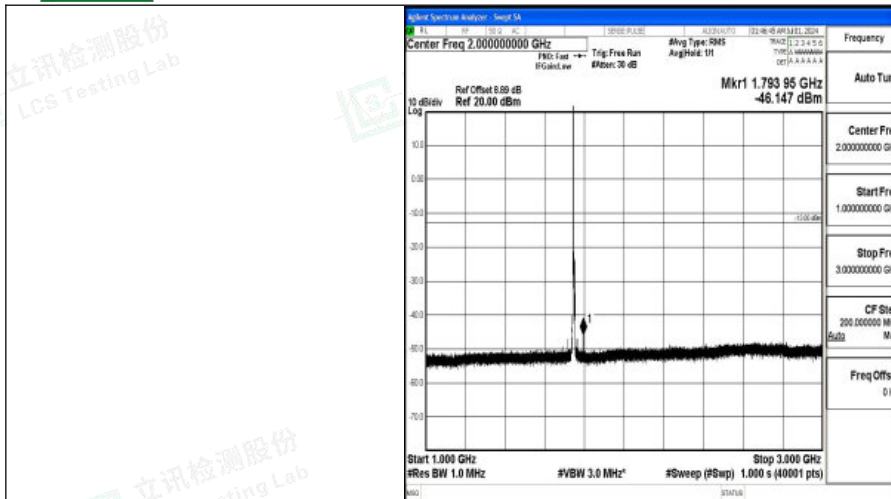
Band66_5MHz_QPSK_132322_1RB#0_1000~3000_1000~3000
