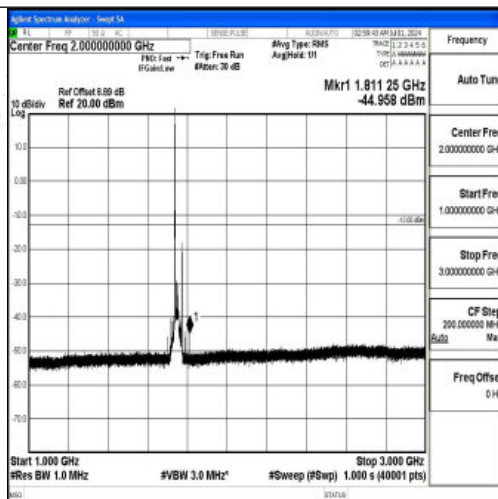
Band66_20MHz_QPSK_132322_1RB#0_1000~3000_1000~3000
