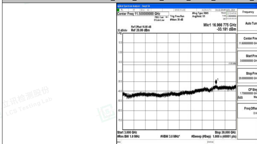
Band66_3MHz_16QAM_132657_1RB#0_3000~20000_3000~20000
