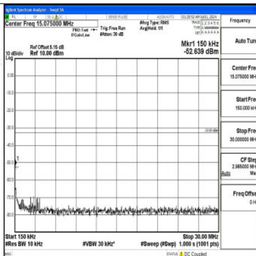
Band66_3MHz_16QAM_132322_1RB#0_0.15~30_0.15~30
