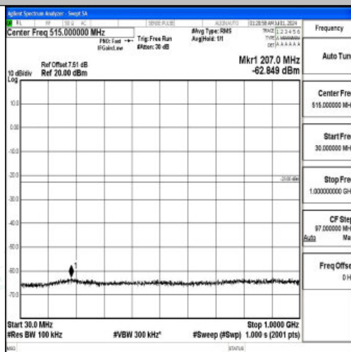
Band66_3MHz_16QAM_132322_1RB#0_30~1000_30~1000
