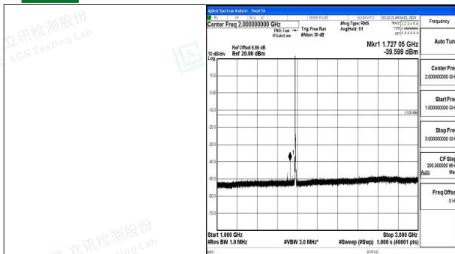
Band66_3MHz_16QAM_132657_1RB#0_1000~3000_1000~3000
