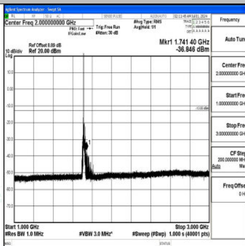
Band66_10MHz_16QAM_132022_1RB#0_1000~3000_1000~3000
