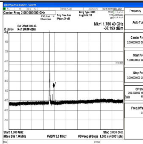
Band66_5MHz_QPSK_131997_1RB#0_1000~3000_1000~3000
