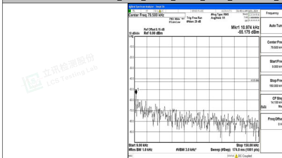
Band66_5MHz_QPSK_131997_1RB#0_0.009~0.15_0.009~0.15
