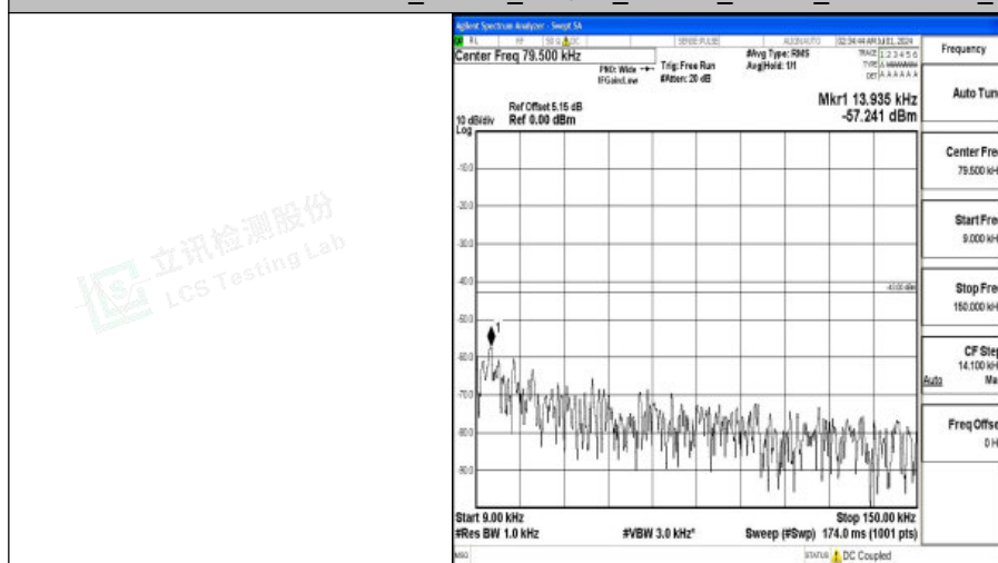
Band66_15MHz_QPSK_132047_1RB#0_0.009~0.15_0.009~0.15
