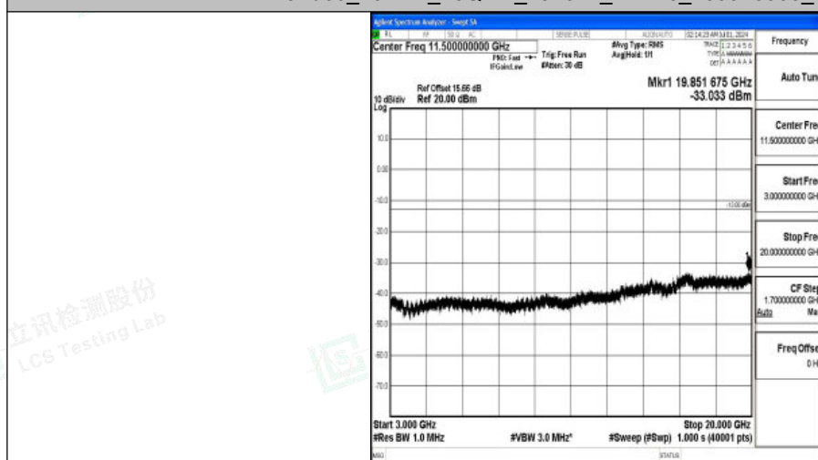
Band66_10MHz_16QAM_132622_1RB#0_3000~20000_3000~20000
