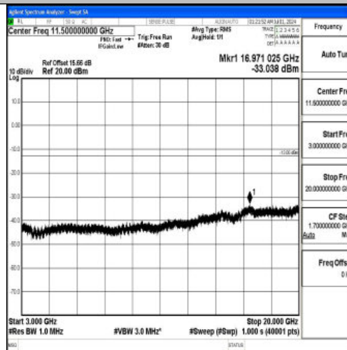
Band66_3MHz_QPSK_132657_1RB#0_3000~20000_3000~20000
