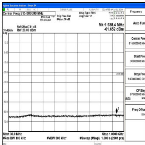
Band66_5MHz_QPSK_132647_1RB#0_30~1000_30~1000
