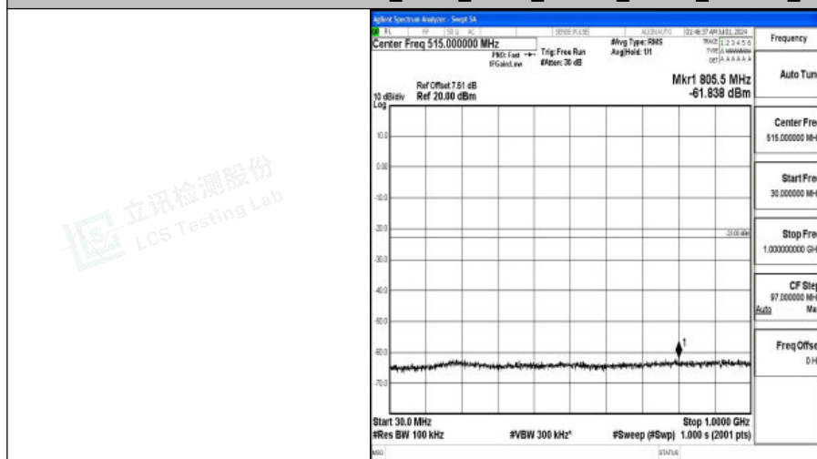
Band66_5MHz_QPSK_132322_1RB#0_30~1000_30~1000
