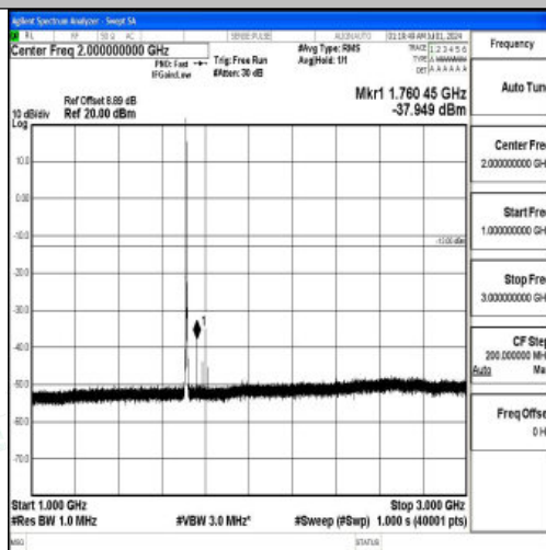
Band66_3MHz_16QAM_131987_1RB#0_1000~3000_1000~3000
