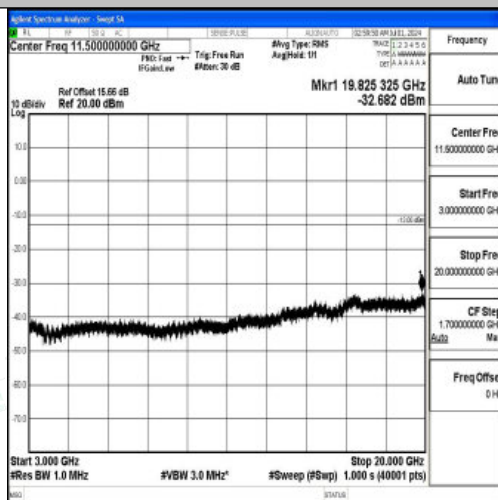
Band66_20MHz_QPSK_132322_1RB#0_3000~20000_3000~20000
