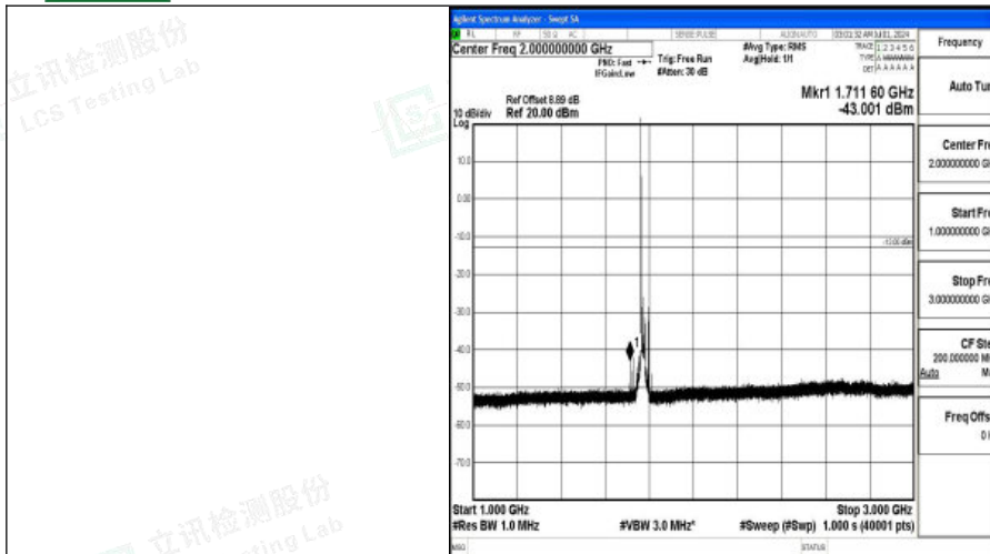
Band66_20MHz_16QAM_132572_1RB#0_1000~3000_1000~3000
