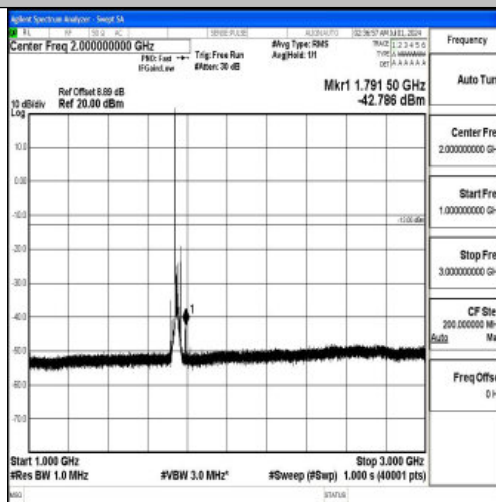
Band66_15MHz_16QAM_132322_1RB#0_1000~3000_1000~3000
