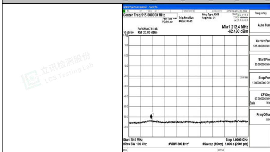
Band66_1.4MHz_16QAM_132665_1RB#0_30~1000_30~1000
