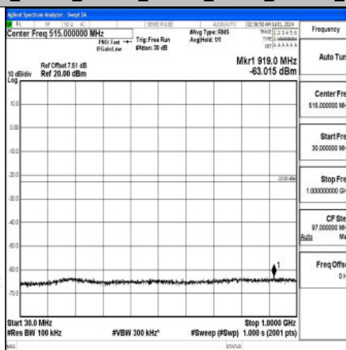
Band66_15MHz_16QAM_132322_1RB#0_30~1000_30~1000
