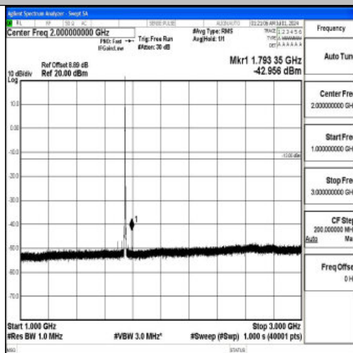
Band66_3MHz_16QAM_132322_1RB#0_1000~3000_1000~3000
