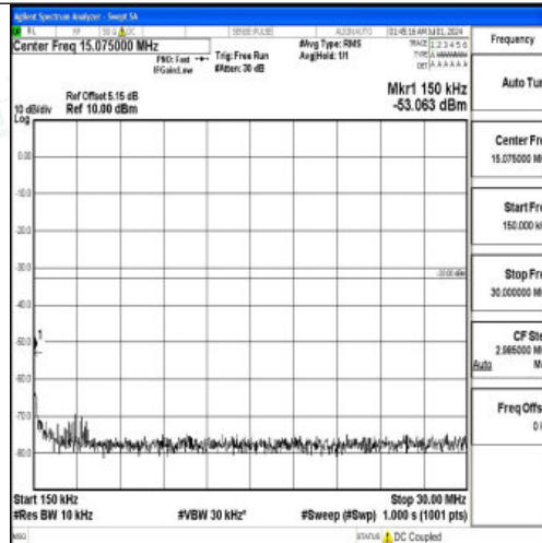
Band66_5MHz_QPSK_131997_1RB#0_0.15~30_0.15~30
