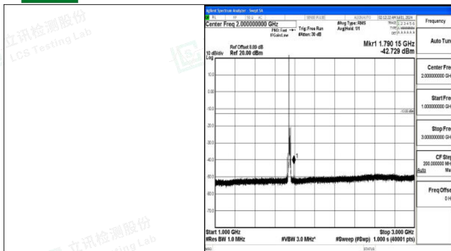
Band66_10MHz_QPSK_132322_1RB#0_1000~3000_1000~3000
