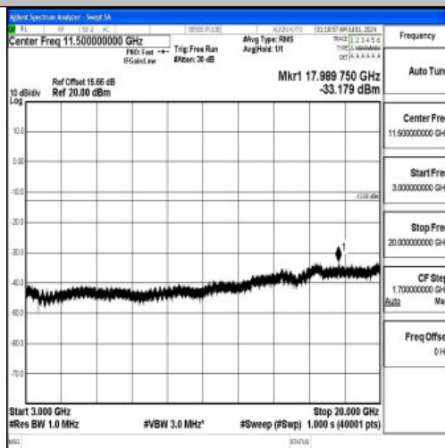
Band66_3MHz_16QAM_131987_1RB#0_3000~20000_3000~20000
