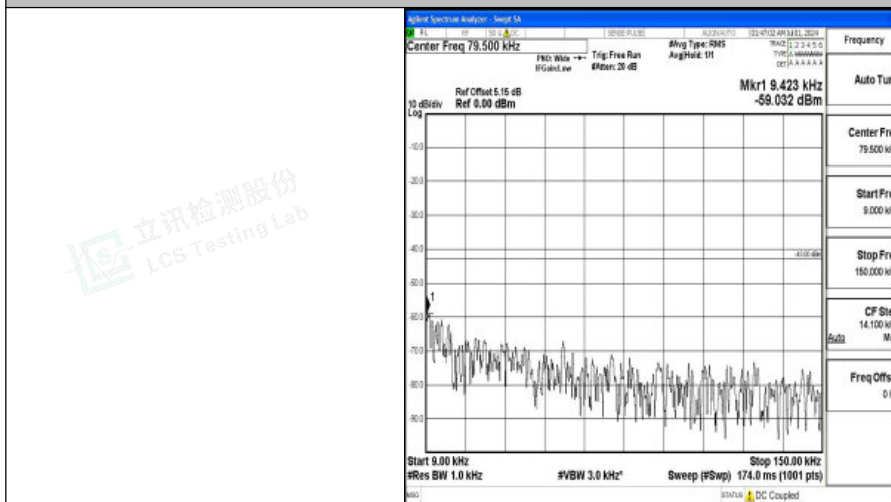
Band66_5MHz_16QAM_132322_1RB#0_0.009~0.15_0.009~0.15
