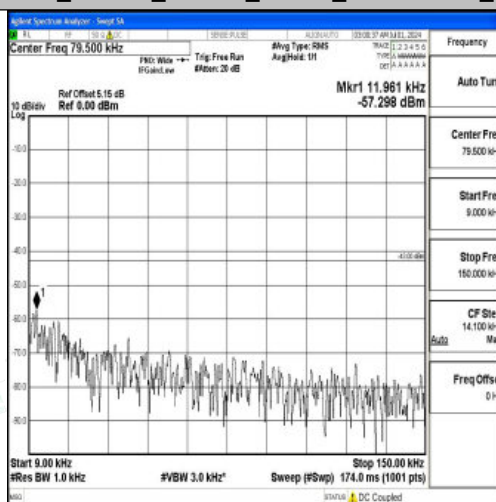
Band66 20MHz QPSK 132572 1RB#0 0.009~0.15 0.009~0.15
