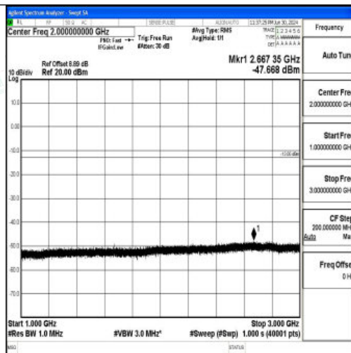
Band26_5MHz_16QAM_26915_1RB#0_1000~3000_1000~3000
