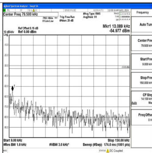
Band26_10MHz_QPSK_26840_1RB#0_0.009~0.15_0.009~0.15
