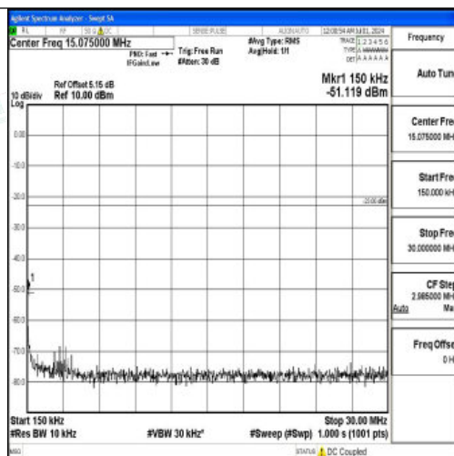
Band26_10MHz_16QAM_26840_1RB#0_0.15~30_0.15~30
