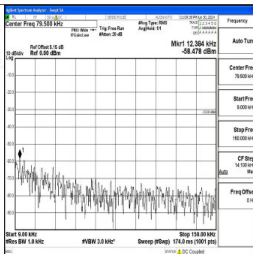
Band26_3MHz_16QAM_26915_1RB#0_0.009~0.15_0.009~0.15
