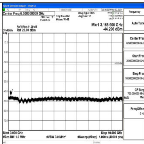
Band26_1.4MHz_QPSK_27033_1RB#0_3000~10000_3000~10000
