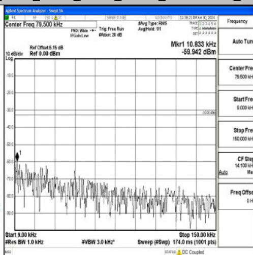
Band26_5MHz_16QAM_27015_1RB#0_0.009~0.15_0.009~0.15
