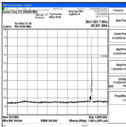
Band26_5MHz_16QAM_27015_1RB#0_30~1000_30~1000
