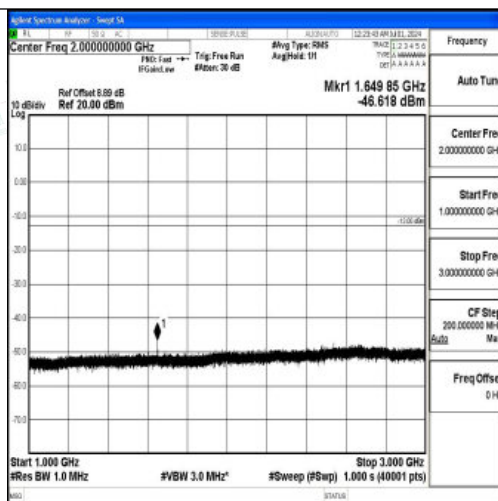
Band26_15MHz_QPSK_26865_1RB#0_1000~3000_1000~3000
