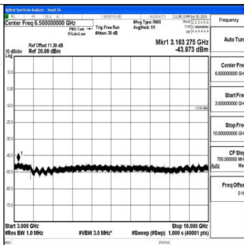
Band26_5MHz_QPSK_27015_1RB#0_3000~10000_3000~10000
