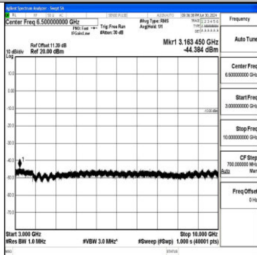
Band26_3MHz_QPSK_26740_1RB#0_3000~10000_3000~10000
