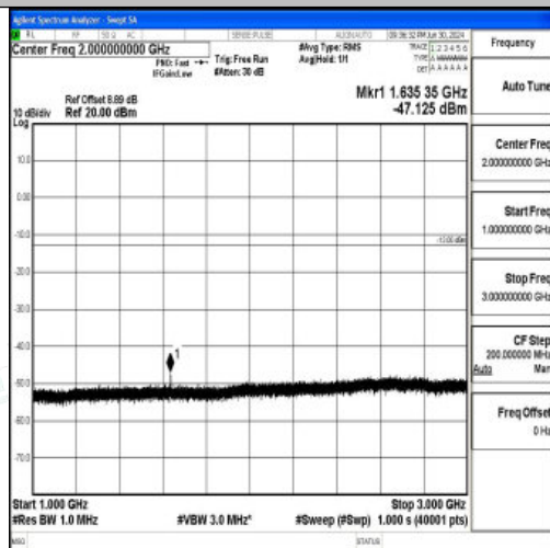
Band26_3MHz_QPSK_26740_1RB#0_1000~3000_1000~3000
