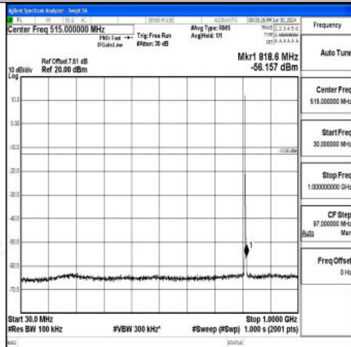
Band26_1.4MHz_16QAM_26697_1RB#0_30~1000_30~1000
