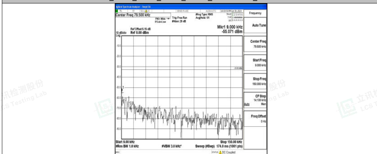
Band26_5MHz_16QAM_26765_1RB#0_0.009~0.15_0.009~0.15
