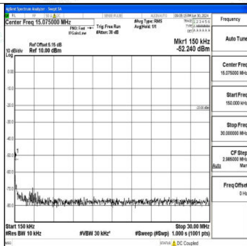
Band26_1.4MHz_QPSK_26783_1RB#0_0.15~30_0.15~30
