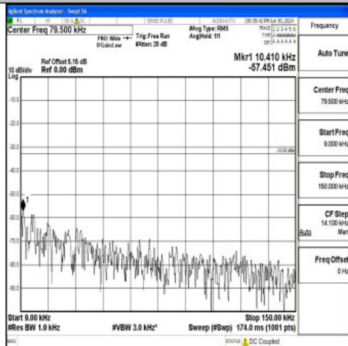
Band26_3MHz_16QAM_26705_1RB#0_0.009~0.15_0.009~0.15
