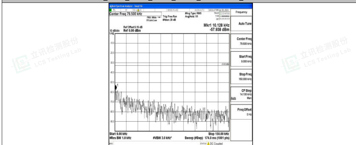
Band26_5MHz_16QAM_26715_1RB#0_0.009~0.15_0.009~0.15
