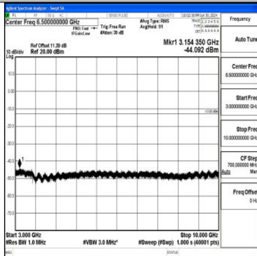
Band26_5MHz_QPSK_26740_1RB#0_3000~10000_3000~10000
