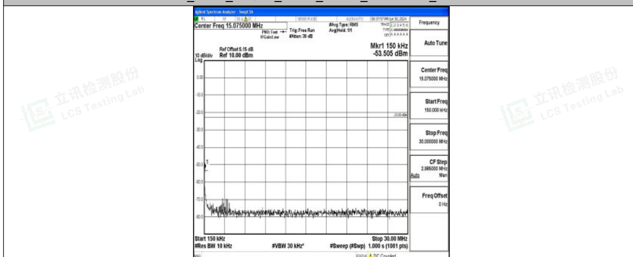
Band26_3MHz_16QAM_26775_1RB#0_0.15~30_0.15~30
