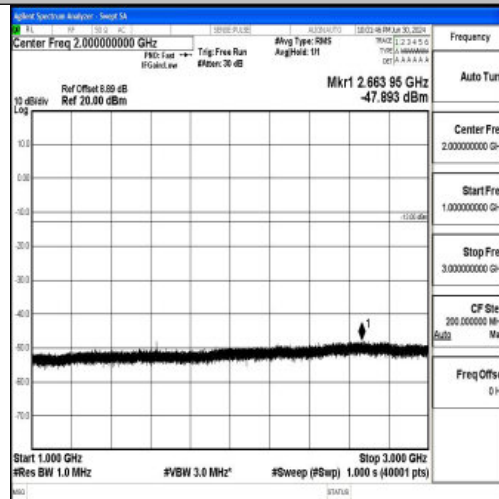
Band26_5MHz_16QAM_26715_1RB#0_1000~3000_1000~3000
