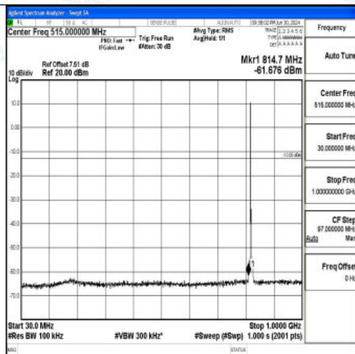
Band26_3MHz_16QAM_26775_1RB#0_30~1000_30~1000
