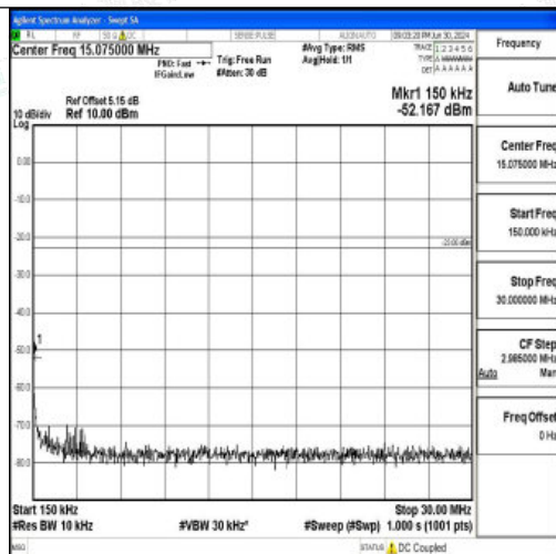
Band26_1.4MHz_16QAM_26697_1RB#0_0.15~30_0.15~30
