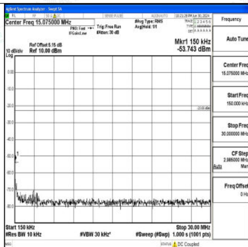
Band26_10MHz_16QAM_26740_1RB#0_0.15~30_0.15~30
