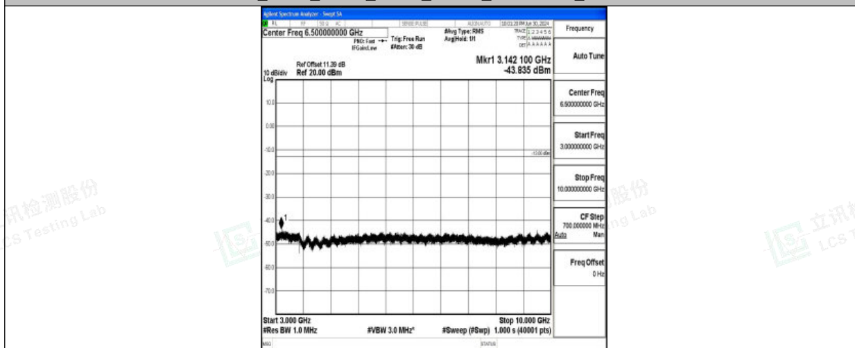
Band26_5MHz_QPSK_26715_1RB#0_3000~10000_3000~10000
