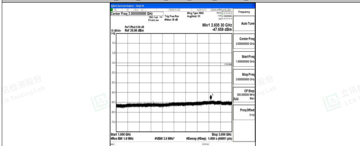
Band26_5MHz_16QAM_26765_1RB#0_1000~3000_1000~3000
