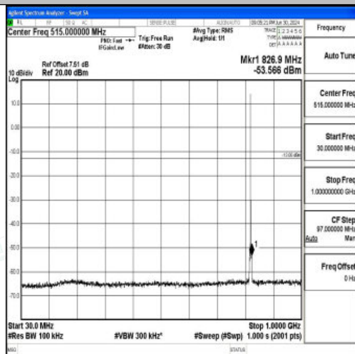
Band26_1.4MHz_QPSK_26783_1RB#0_30~1000_30~1000
