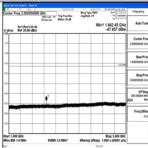
Band26_3MHz_16QAM_26775_1RB#0_1000~3000_1000~3000
