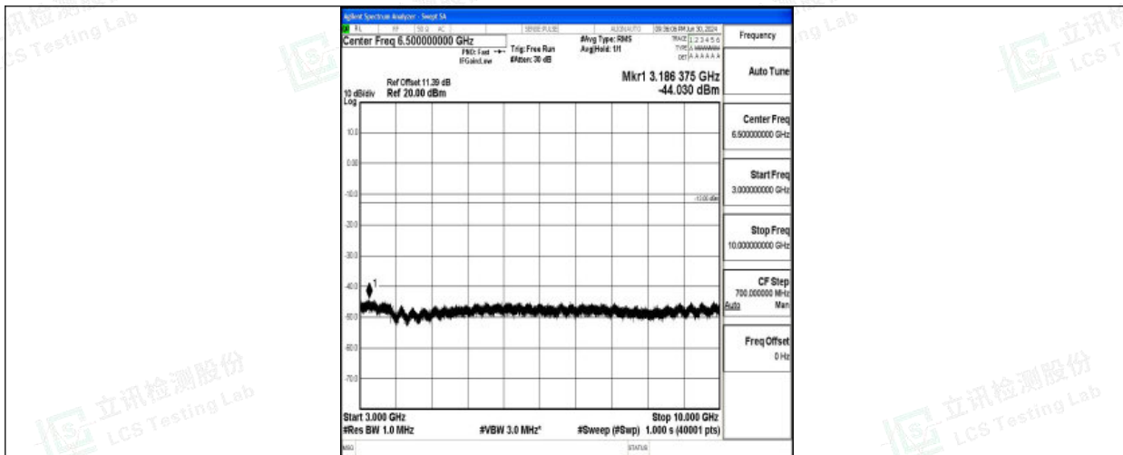
Band26_3MHz_16QAM_26705_1RB#0_3000~10000_3000~10000
