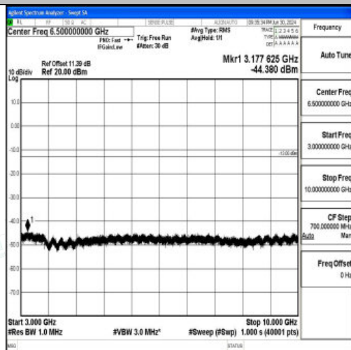
Band26_3MHz_QPSK_26705_1RB#0_3000~10000_3000~10000
