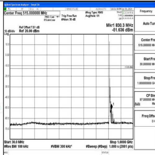
Band26_5MHz_16QAM_26715_1RB#0_30~1000_30~1000
