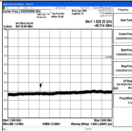
Band26_10MHz_16QAM_26740_1RB#0_1000~3000_1000~3000
