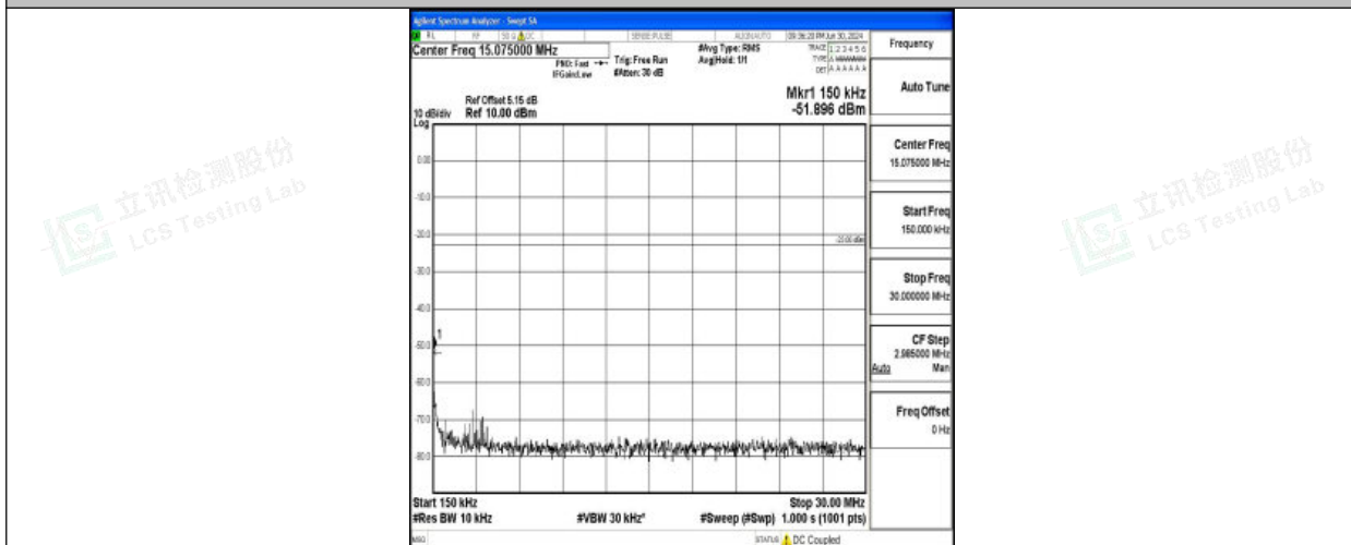
Band26_3MHz_QPSK_26740_1RB#0_0.15~30_0.15~30
