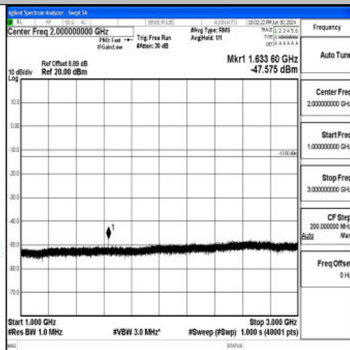
Band26_5MHz_QPSK_26740_1RB#0_1000~3000_1000~3000
