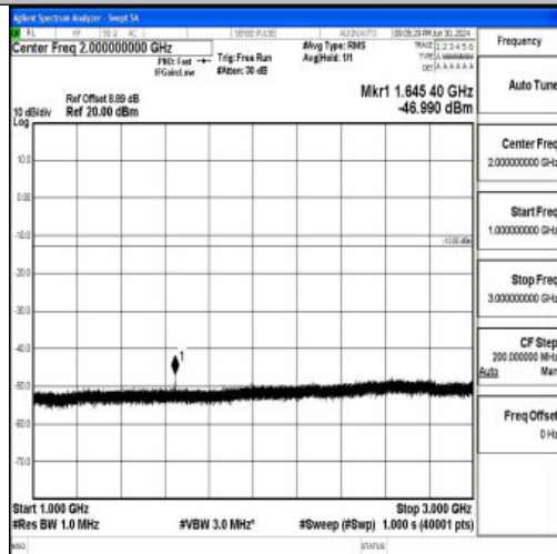
Band26_1.4MHz_QPSK_26783_1RB#0_1000~3000_1000~3000
