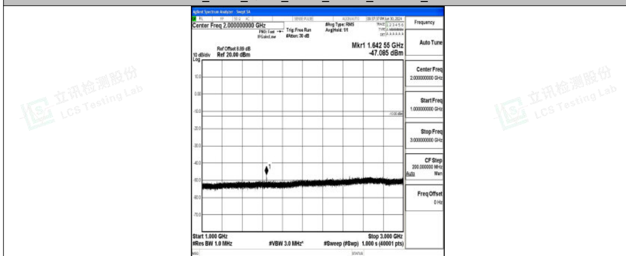
Band26_3MHz_QPSK_26775_1RB#0_1000~3000_1000~3000
