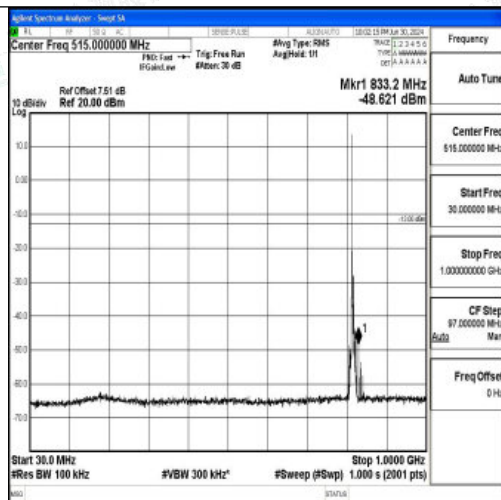
Band26_5MHz_QPSK_26740_1RB#0_30~1000_30~1000
