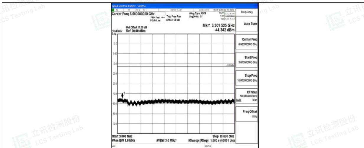
Band26_1.4MHz_QPSK_26783_1RB#0_3000~10000_3000~10000
