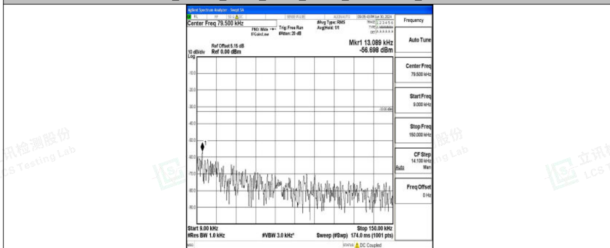
Band26_1.4MHz_16QAM_26783_1RB#0_0.009~0.15_0.009~0.15
