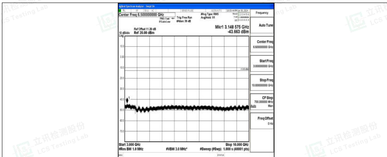
Band26_5MHz_QPSK_26765_1RB#0_3000~10000_3000~10000
