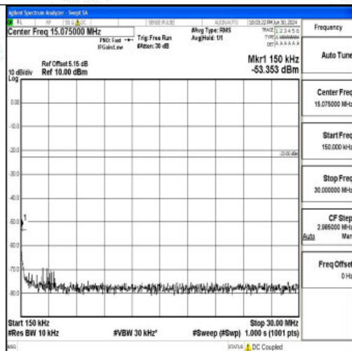
Band26_5MHz_QPSK_26765_1RB#0_0.15~30_0.15~30
