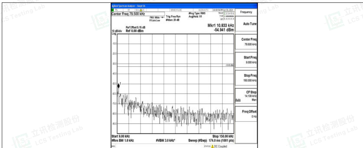
Band26_5MHz_QPSK_26715_1RB#0_0.009~0.15_0.009~0.15
