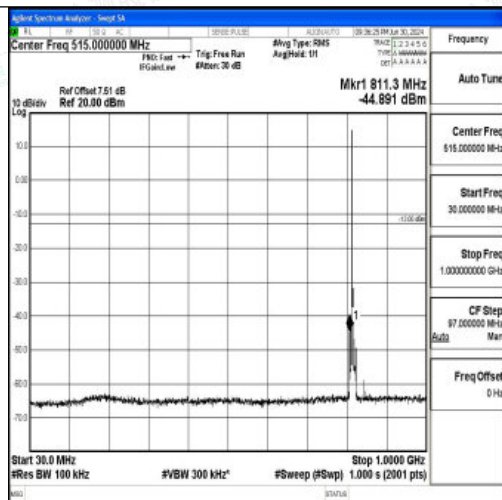
Band26_3MHz_QPSK_26740_1RB#0_30~1000_30~1000
