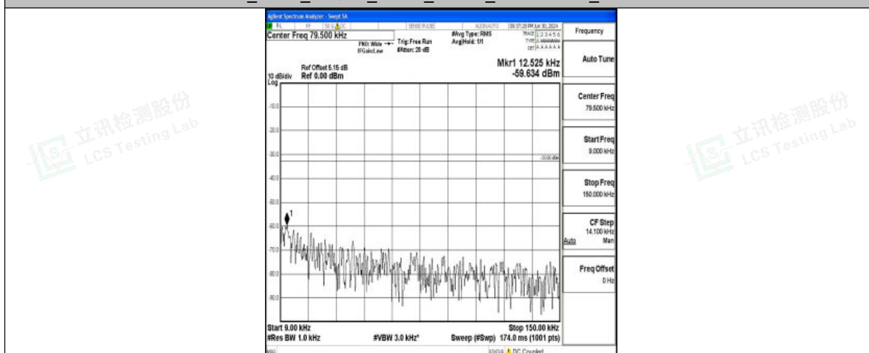
Band26_3MHz_QPSK_26775_1RB#0_0.009~0.15_0.009~0.15
