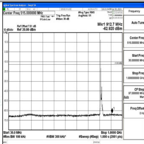
Band26_10MHz_16QAM_26740_1RB#0_30~1000_30~1000
