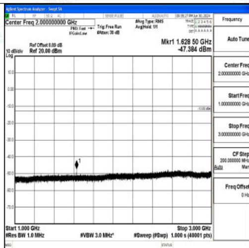
Band26_3MHz_QPSK_26705_1RB#0_1000~3000_1000~3000
