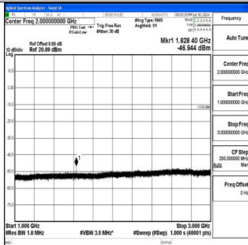
Band26_1.4MHz_16QAM_26697_1RB#0_1000~3000_1000~3000
