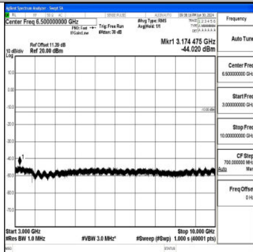
Band26_3MHz_16QAM_26775_1RB#0_3000~10000_3000~10000
