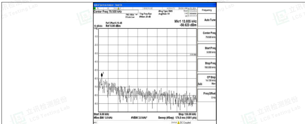
Band26_3MHz_QPSK_26705_1RB#0_0.009~0.15_0.009~0.15
