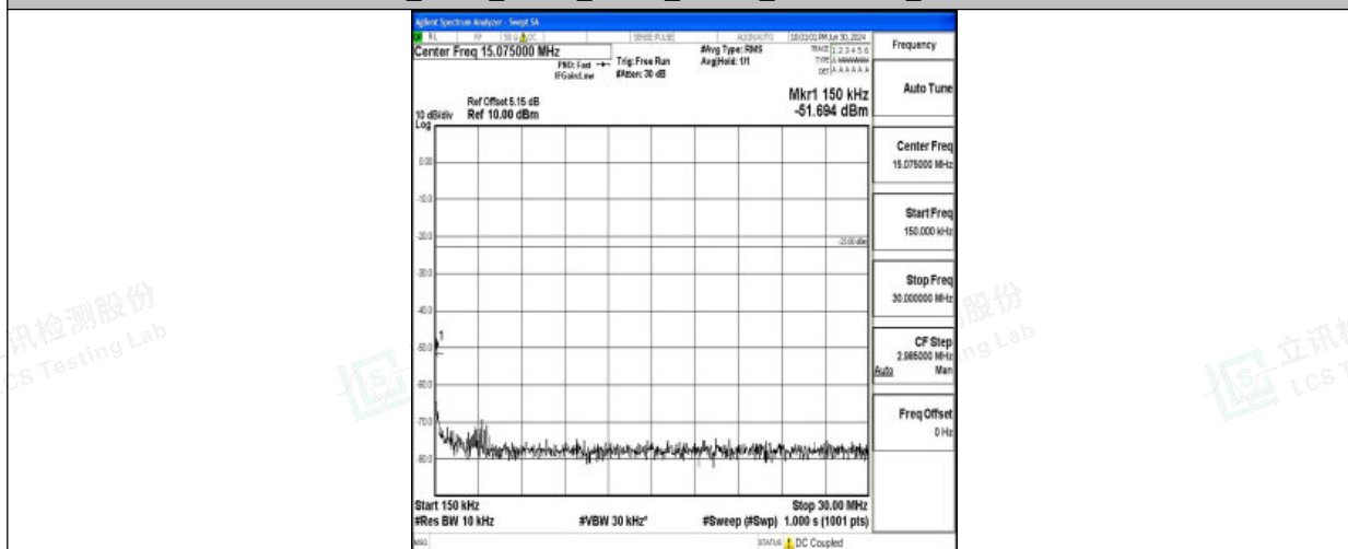
Band26_5MHz_QPSK_26715_1RB#0_0.15~30_0.15~30
