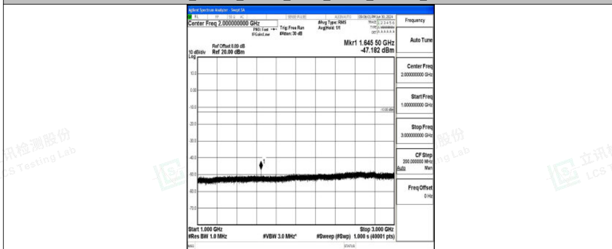
Band26_1.4MHz_16QAM_26783_1RB#0_1000~3000_1000~3000
