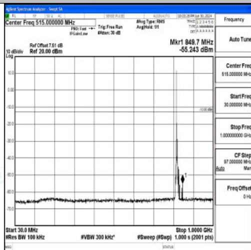
Band26_5MHz_QPSK_26765_1RB#0_30~1000_30~1000
