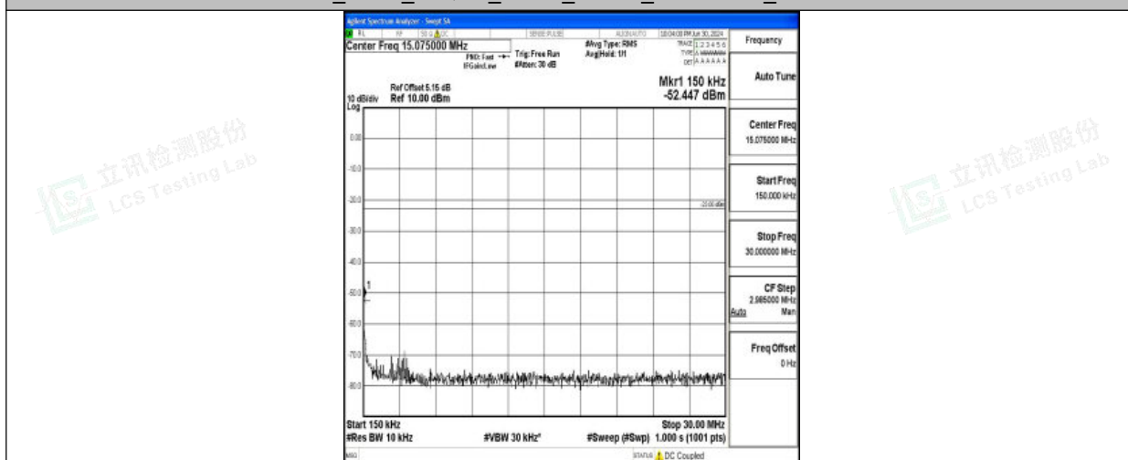
Band26_5MHz_16QAM_26765_1RB#0_0.15~30_0.15~30
