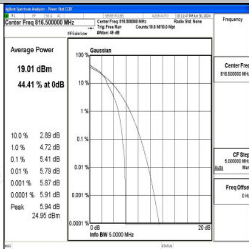
26(814-824)-5MHz-16QAM-26715-1RB#0-PASS
