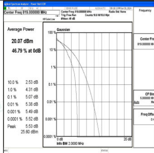
26(814-824)-1.4MHz-QPSK-26740-1RB#0-PASS
