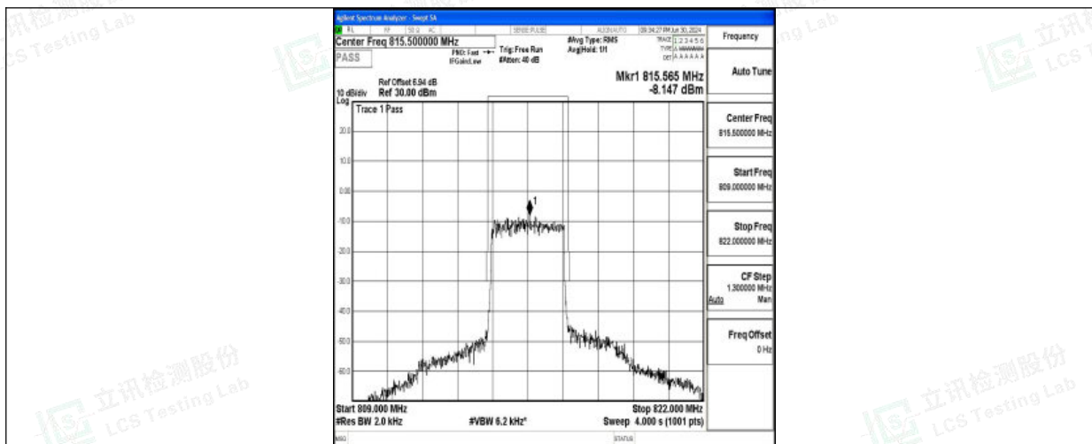
Band26_3MHz_QPSK_26705_15RB#0
