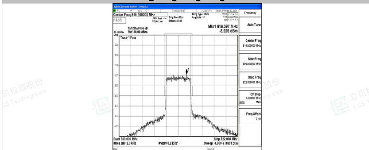
Band26_3MHz_16QAM_26705_15RB#0
