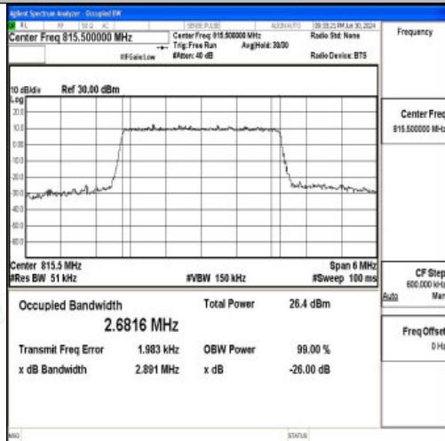
26(814-824)-3MHz-16QAM-26705-15RB#0-PASS
