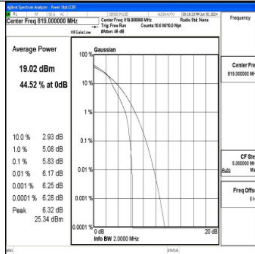
26(814-824)-1.4MHz-16QAM-26740-1RB#0-PASS
