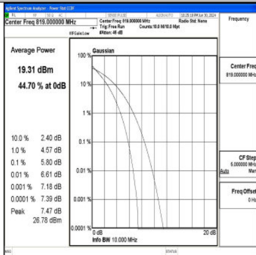
26(814-824)-10MHz-QPSK-26740-50RB#0-PASS
