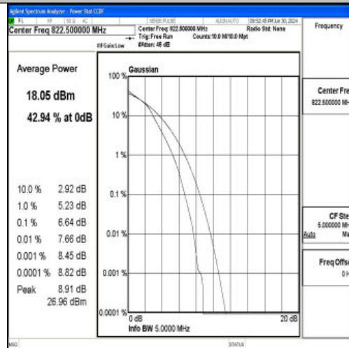
26(814-824)-3MHz-16QAM-26775-15RB#0-PASS
