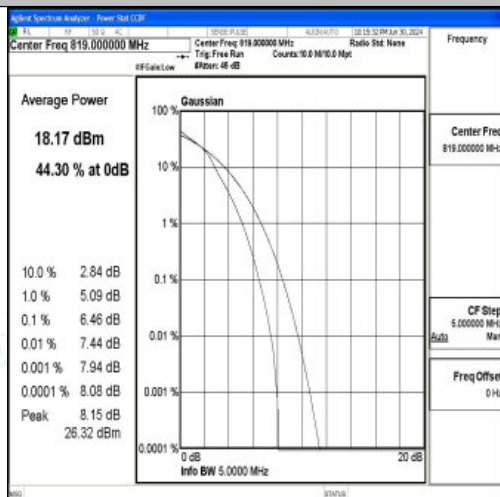
26(814-824)-5MHz-16QAM-26740-25RB#0-PASS
