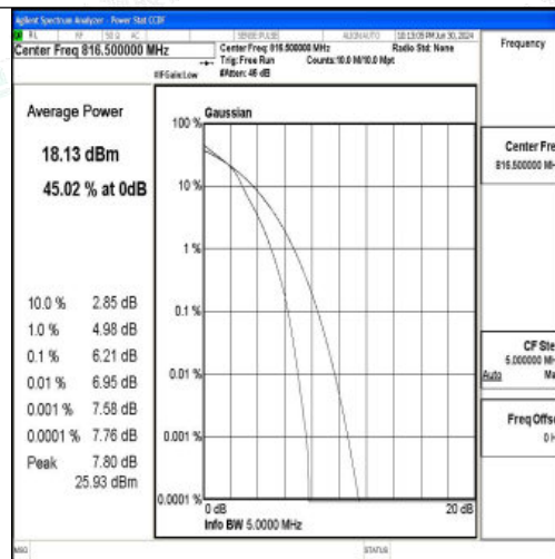
26(814-824)-5MHz-16QAM-26715-25RB#0-PASS
