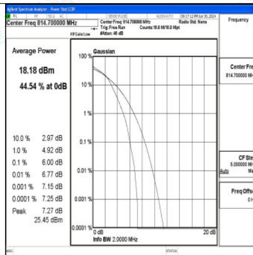
26(814-824)-1.4MHz-16QAM-26697-6RB#0-PASS
