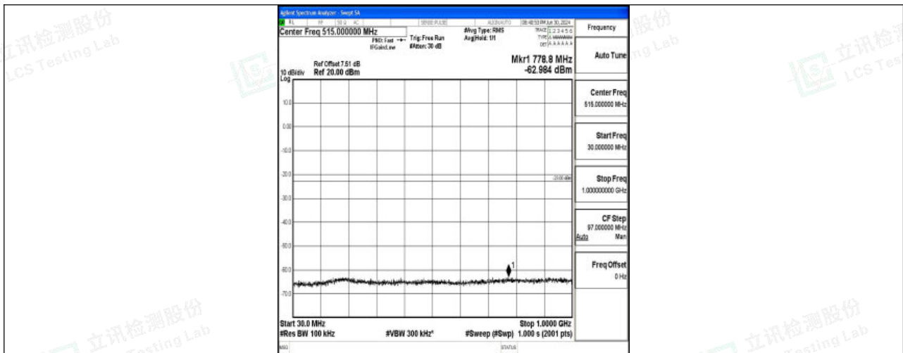
Band25_20MHz_16QAM_26140_1RB#0_30~1000_30~1000
