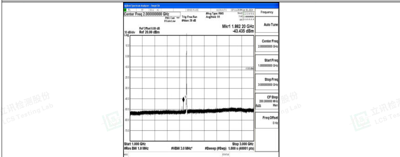
Band25_3MHz_QPSK_26675_1RB#0_1000~3000_1000~3000
