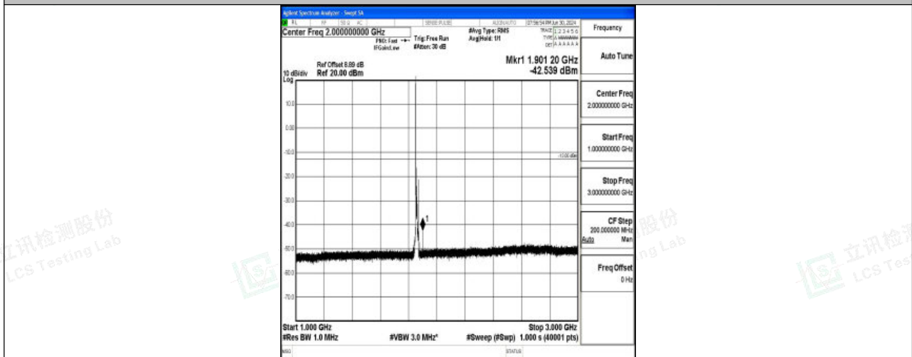
Band25_10MHz_16QAM_26090_1RB#0_1000~3000_1000~3000
