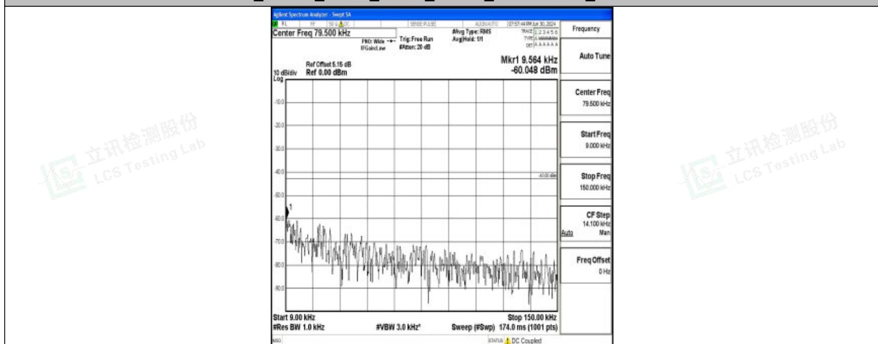
Band25_10MHz_16QAM_26365_1RB#0_0.009~0.15_0.009~0.15
