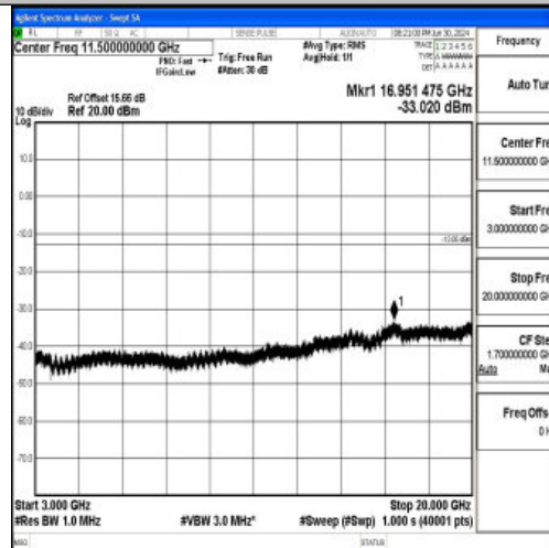
Band25_15MHz_QPSK_26615_1RB#0_3000~20000_3000~20000
