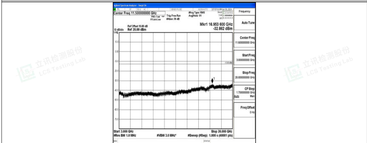
Band25_10MHz_16QAM_26090_1RB#0_3000~20000_3000~20000
