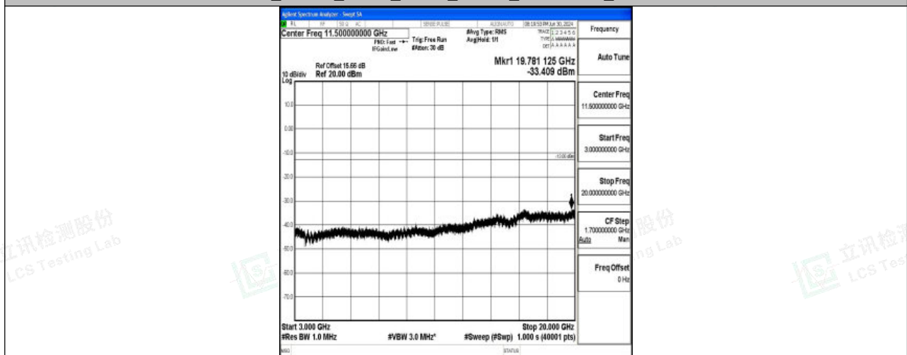
Band25_15MHz_QPSK_26365_1RB#0_3000~20000_3000~20000
