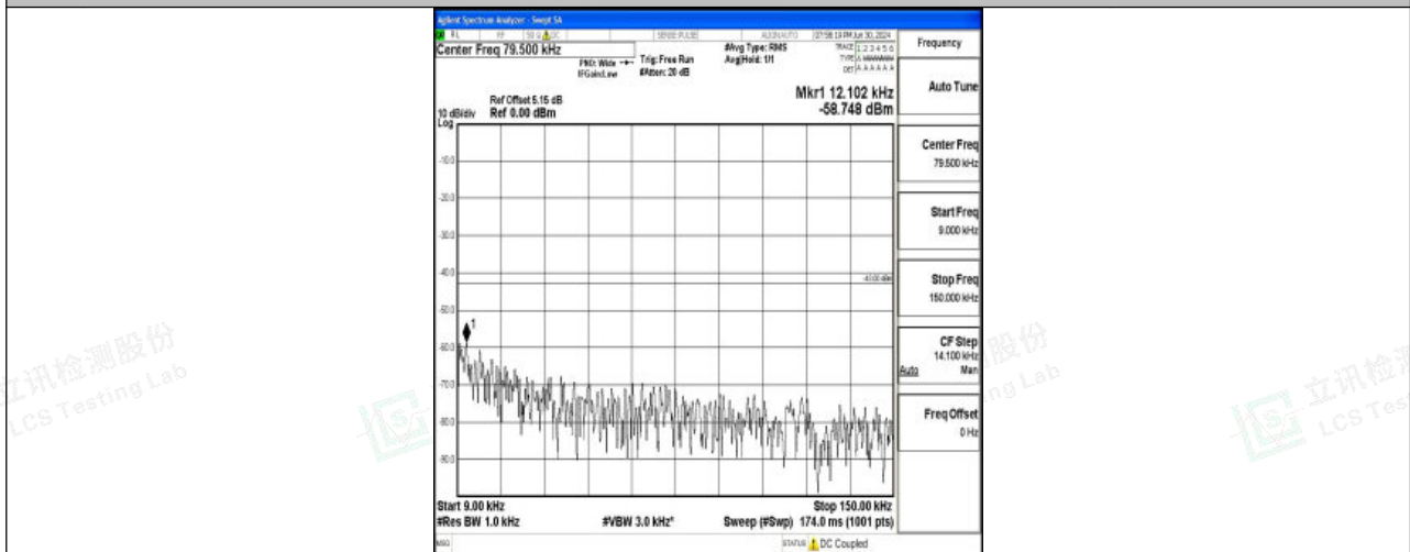
Band25_10MHz_QPSK_26640_1RB#0_0.009~0.15_0.009~0.15
