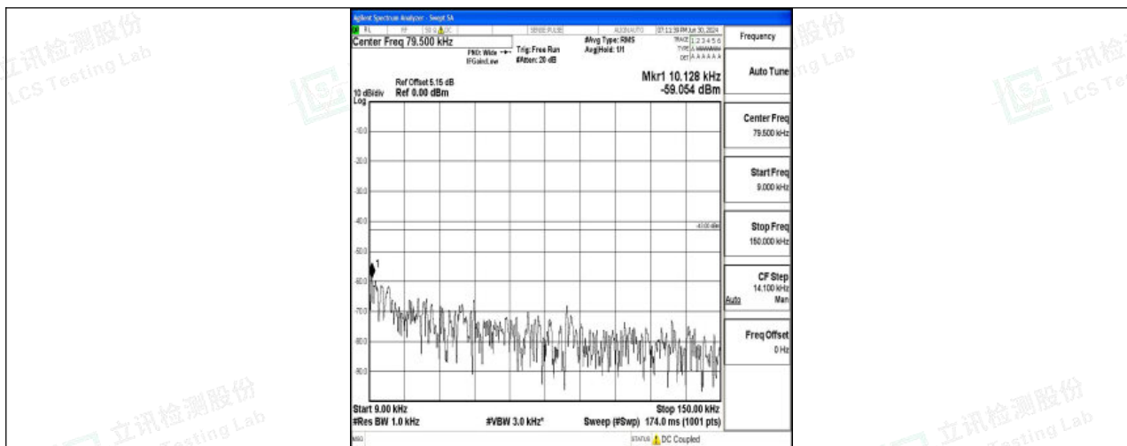
Band25_3MHz_16QAM_26675_1RB#0_0.009~0.15_0.009~0.15
