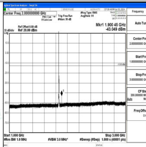
Band25_3MHz_16QAM_26055_1RB#0_1000~3000_1000~3000
