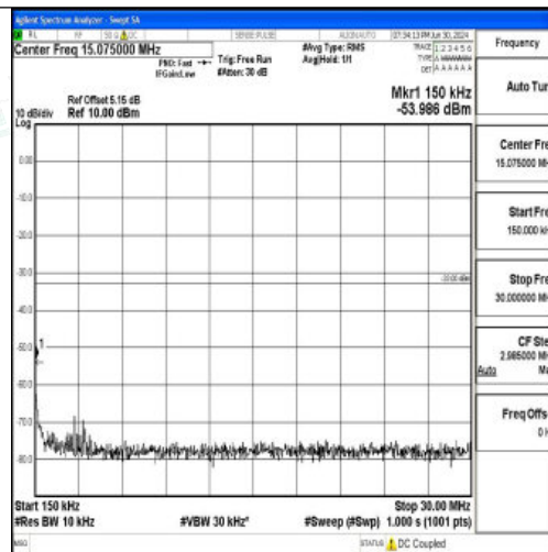
Band25_5MHz_16QAM_26365_1RB#0_0.15~30_0.15~30
