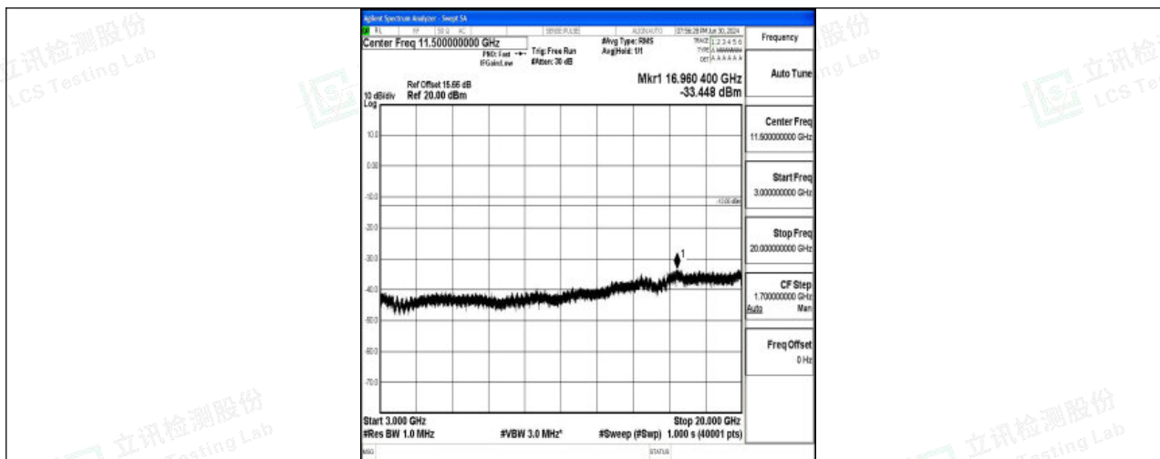
Band25_10MHz_QPSK_26090_1RB#0_3000~20000_3000~20000
