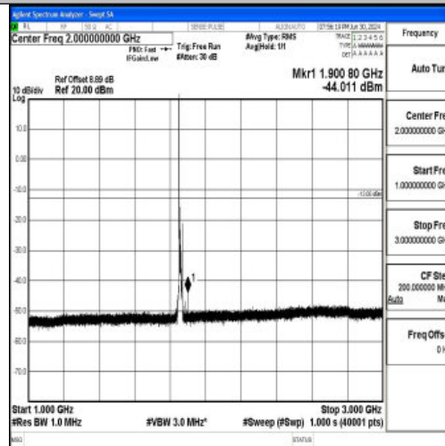
Band25_10MHz_QPSK_26090_1RB#0_1000~3000_1000~3000
