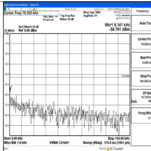
Band25_10MHz_QPSK_26365_1RB#0_0.009~0.15_0.009~0.15
