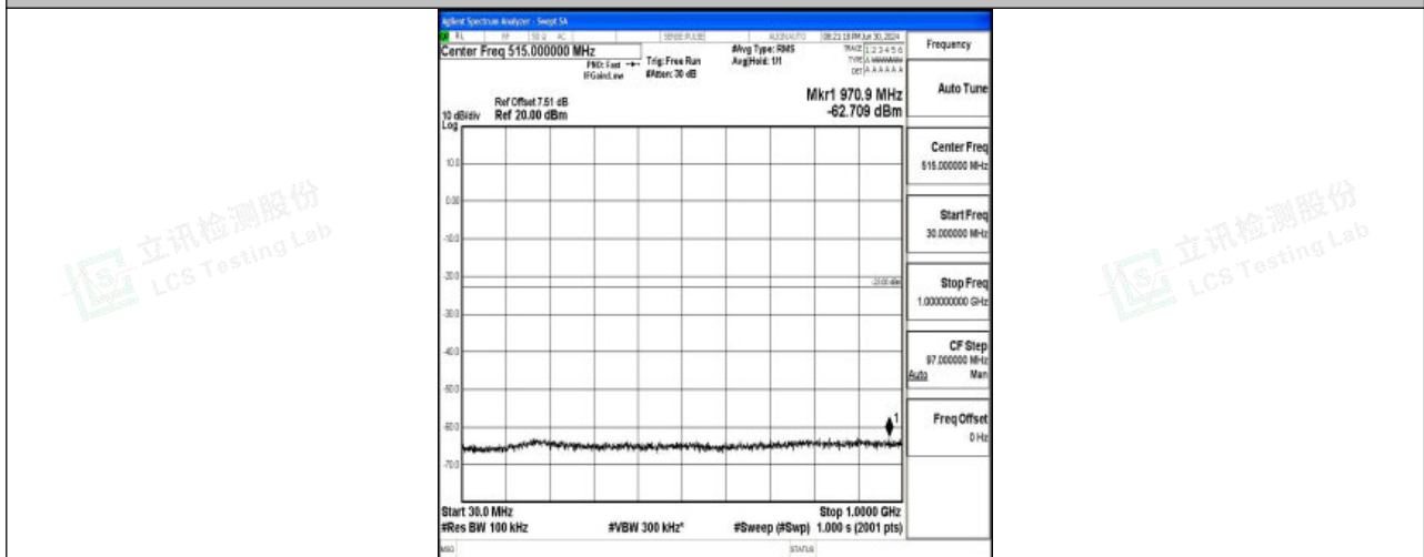
Band25_15MHz_16QAM_26615_1RB#0_30~1000_30~1000
