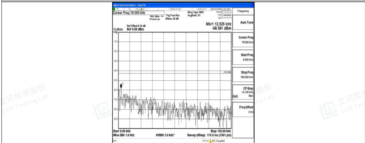
Band25_15MHz_QPSK_26615_1RB#0_0.009~0.15_0.009~0.15
