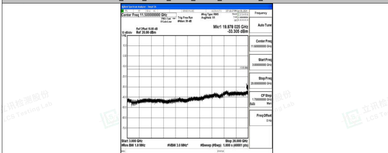
Band25_3MHz_QPSK_26365_1RB#0_3000~20000_3000~20000
