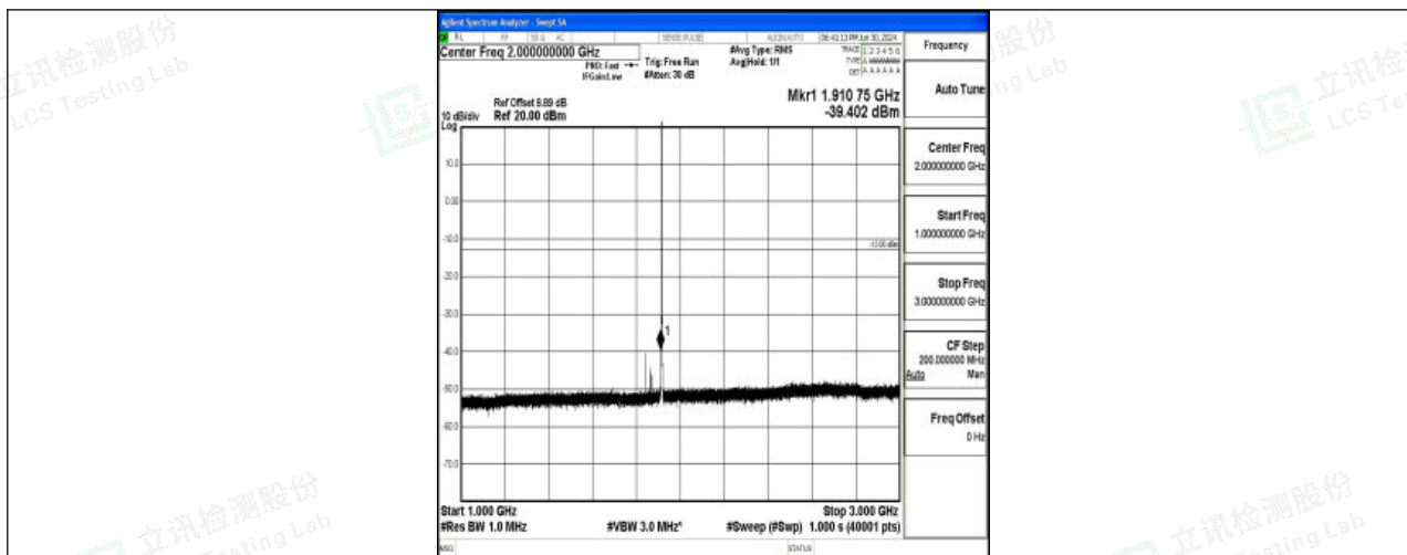
Band25_1.4MHz_16QAM_26683_1RB#0_1000~3000_1000~3000
