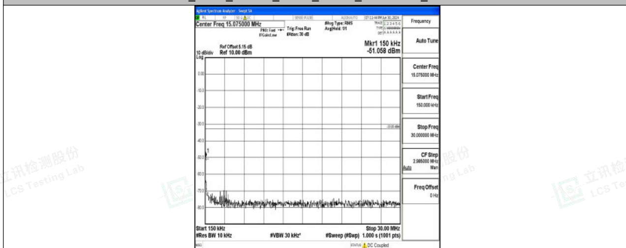
Band25_3MHz_16QAM_26675_1RB#0_0.15~30_0.15~30
