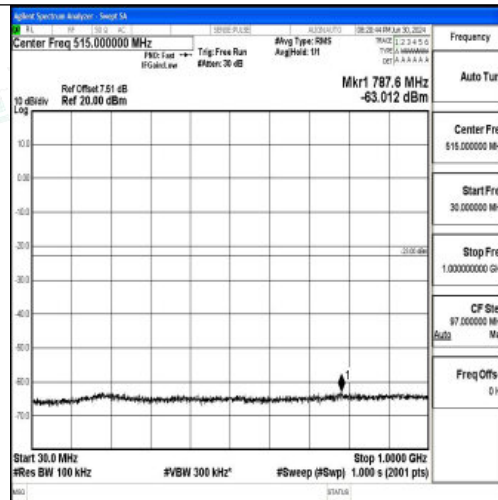
Band25_15MHz_QPSK_26615_1RB#0_30~1000_30~1000
