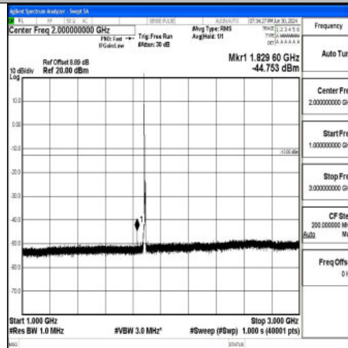
Band25_5MHz_16QAM_26365_1RB#0_1000~3000_1000~3000
