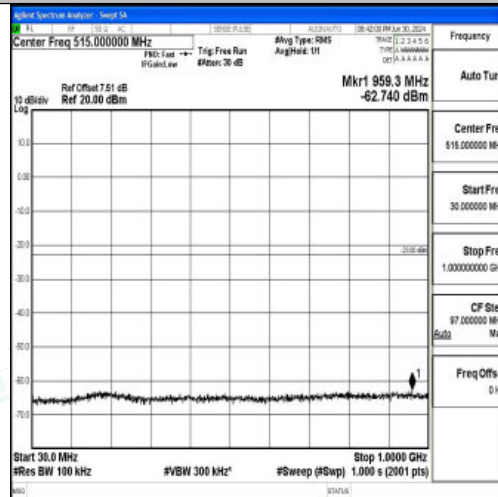
Band25_20MHz_16QAM_26365_1RB#0_30~1000_30~1000
