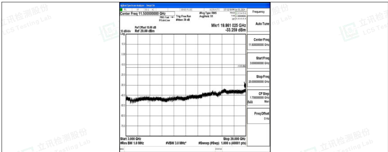
Band25_5MHz_QPSK_26065_1RB#0_3000~20000_3000~20000
