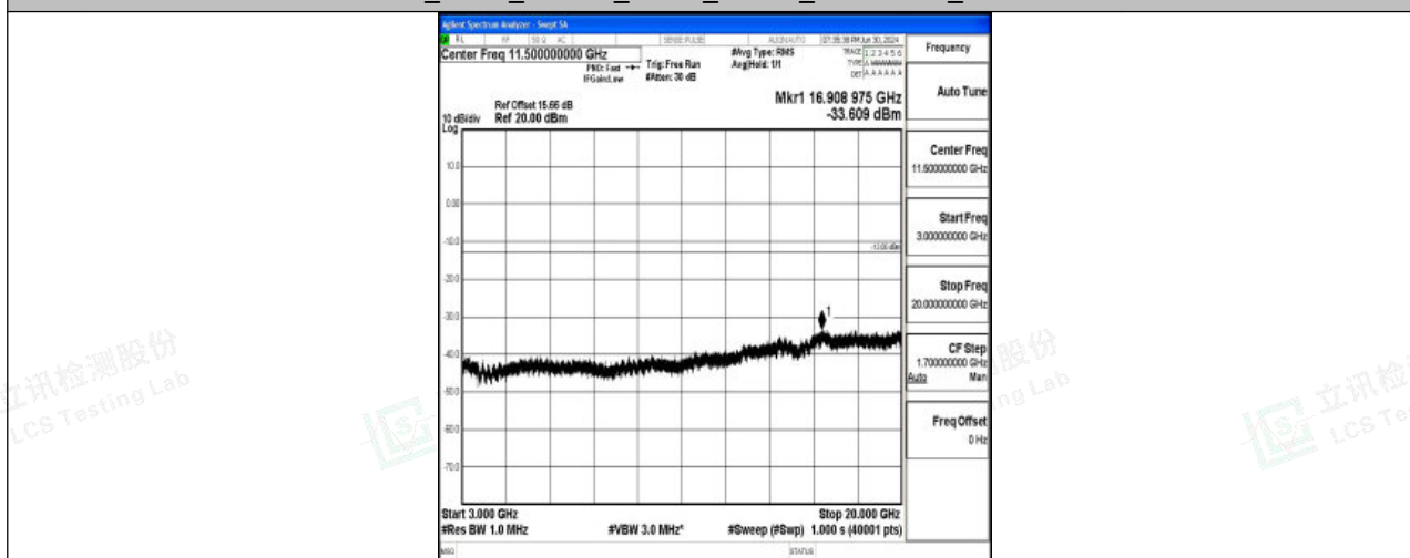
Band25_5MHz_16QAM_26665_1RB#0_3000~20000_3000~20000
