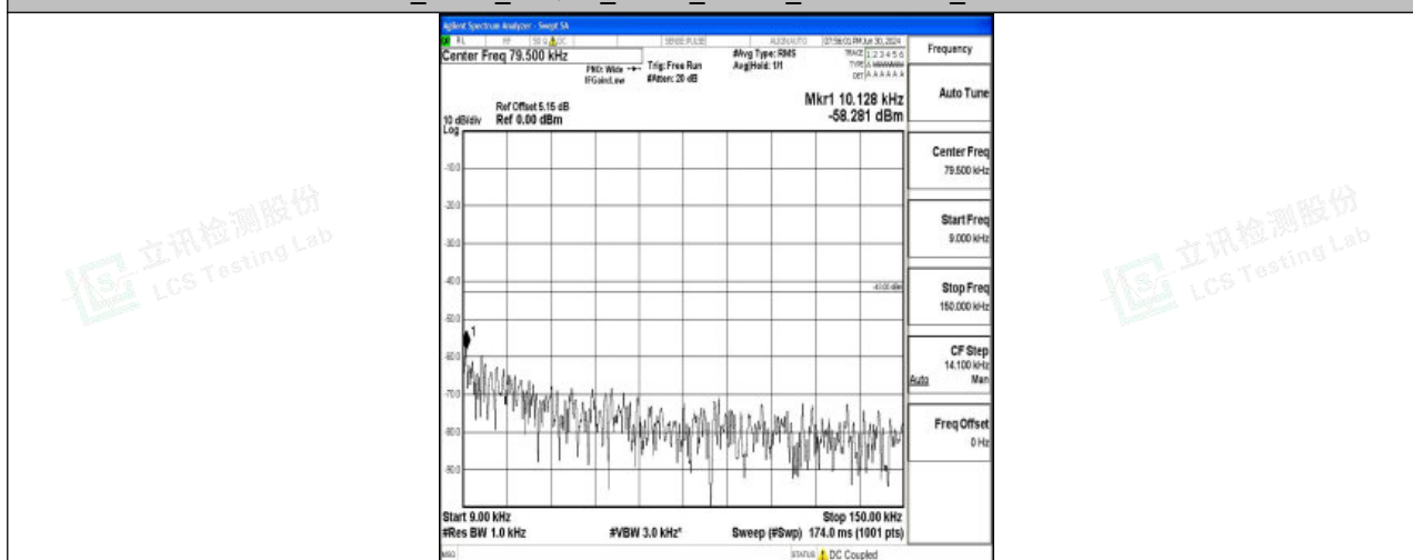
Band25_10MHz_QPSK_26090_1RB#0_0.009~0.15_0.009~0.15
