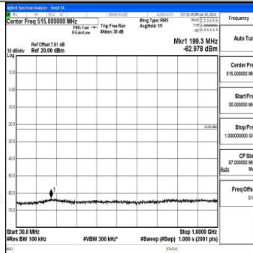
Band25_5MHz_QPSK_26065_1RB#0_30~1000_30~1000
