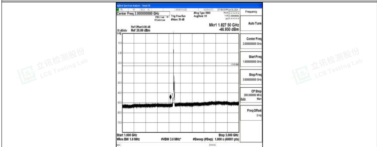
Band25_10MHz_16QAM_26365_1RB#0_1000~3000_1000~3000
