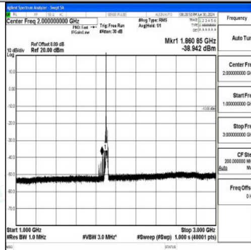
Band25_15MHz_QPSK_26615_1RB#0_1000~3000_1000~3000
