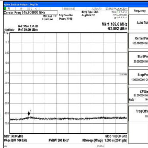
Band25_5MHz_16QAM_26365_1RB#0_30~1000_30~1000
