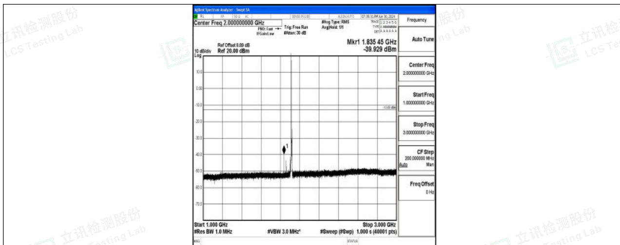
Band25_5MHz_16QAM_26665_1RB#0_1000~3000_1000~3000
