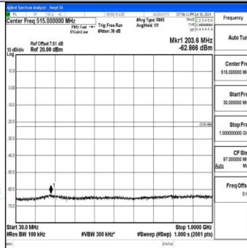
Band25_10MHz_QPSK_26090_1RB#0_30~1000_30~1000
