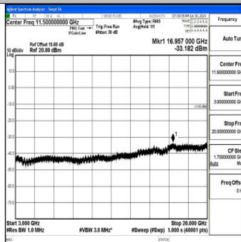
Band25_3MHz_16QAM_26055_1RB#0_3000~20000_3000~20000
