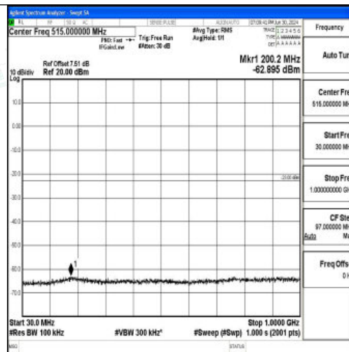
Band25_3MHz_16QAM_26055_1RB#0_30~1000_30~1000
