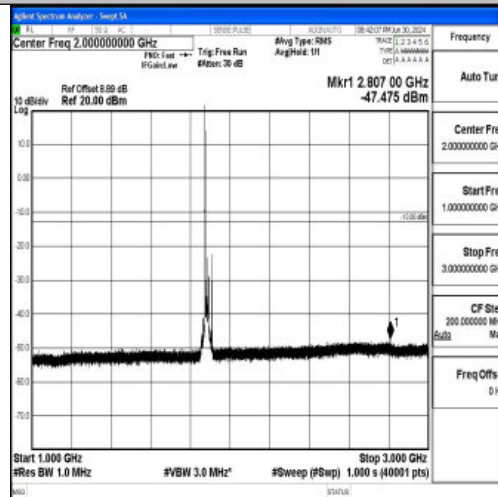
Band25_20MHz_16QAM_26365_1RB#0_1000~3000_1000~3000
