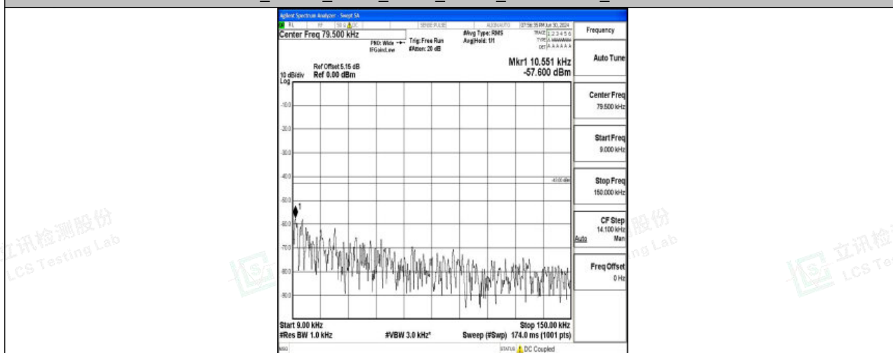
Band25_10MHz_16QAM_26090_1RB#0_0.009~0.15_0.009~0.15
