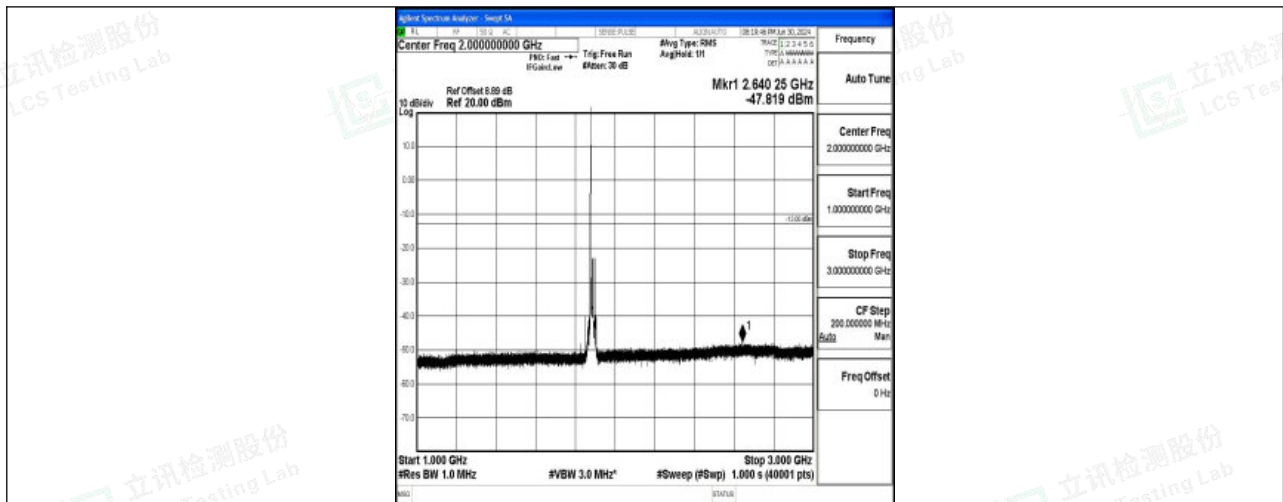
Band25_15MHz_QPSK_26365_1RB#0_1000~3000_1000~3000
