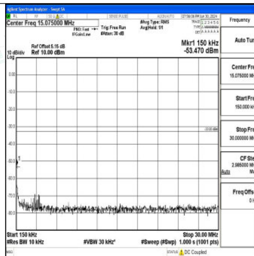
Band25_10MHz_QPSK_26090_1RB#0_0.15~30_0.15~30
