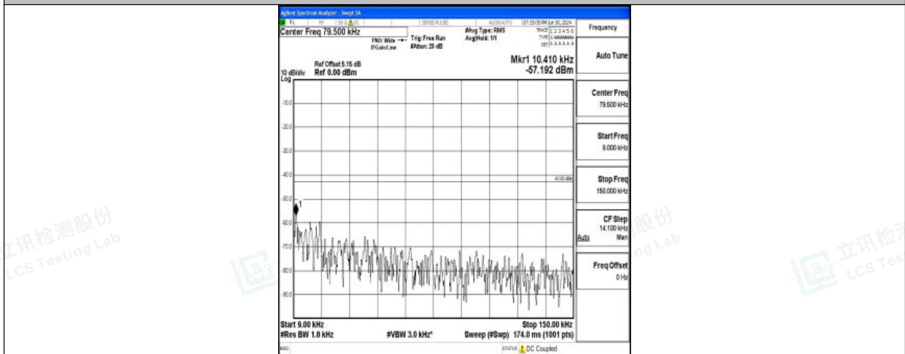
Band25_5MHz_16QAM_26065_1RB#0_0.009~0.15_0.009~0.15
