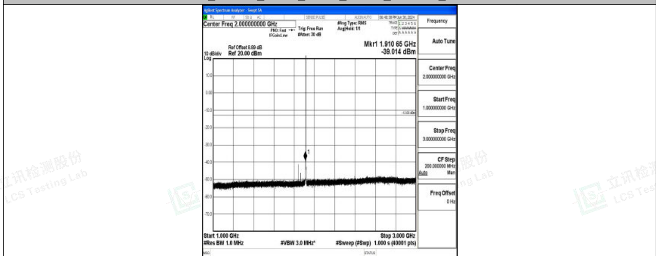
Band25_1.4MHz_QPSK_26683_1RB#0_1000~3000_1000~3000
