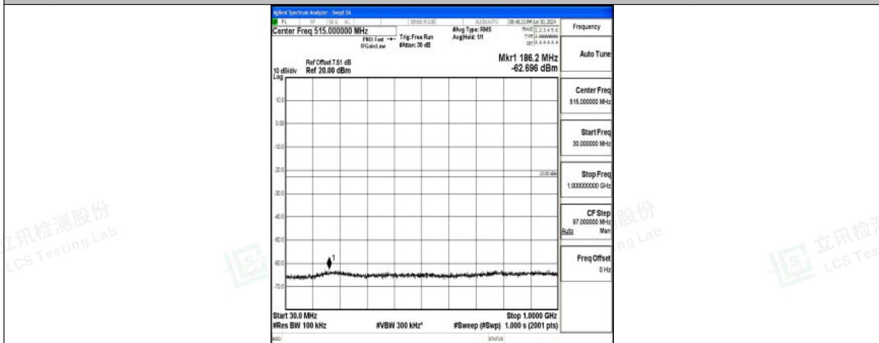
Band25_20MHz_QPSK_26140_1RB#0_30~1000_30~1000
