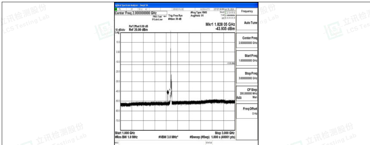
Band25_10MHz_QPSK_26365_1RB#0_1000~3000_1000~3000
