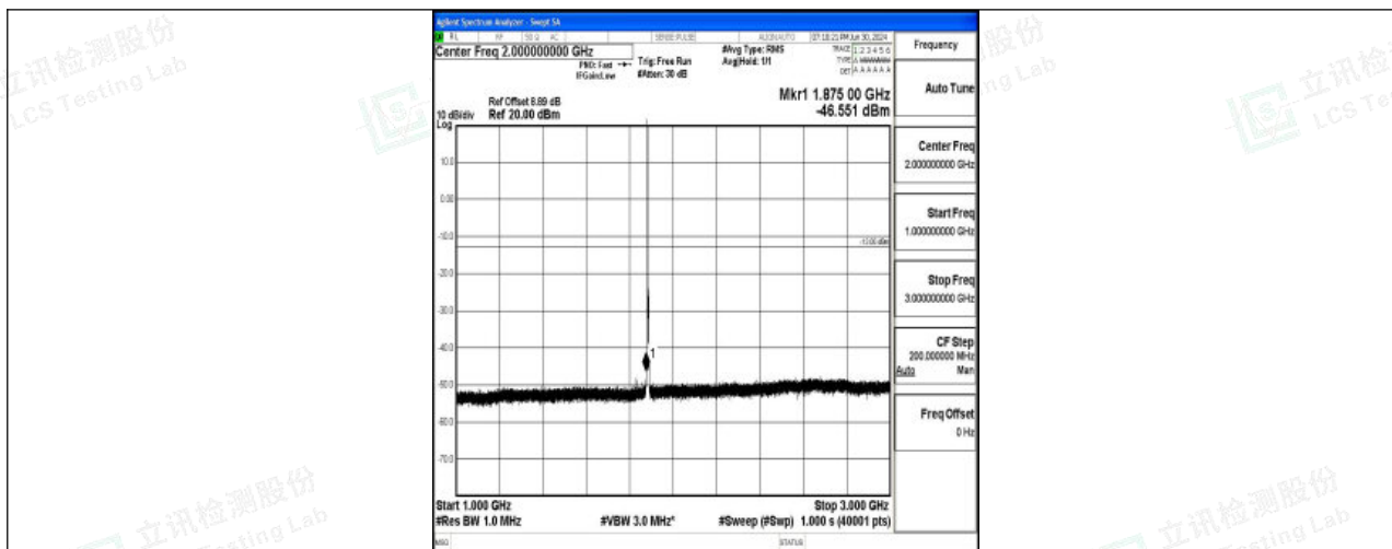
Band25_3MHz_QPSK_26365_1RB#0_1000~3000_1000~3000
