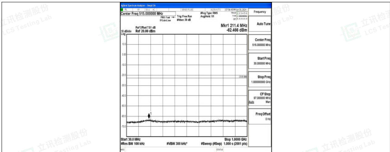
Band25_10MHz_16QAM_26090_1RB#0_30~1000_30~1000
