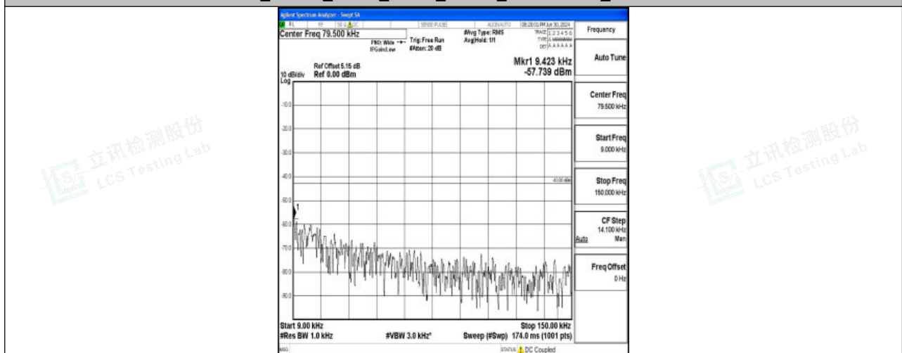
Band25_15MHz_16QAM_26365_1RB#0_0.009~0.15_0.009~0.15
