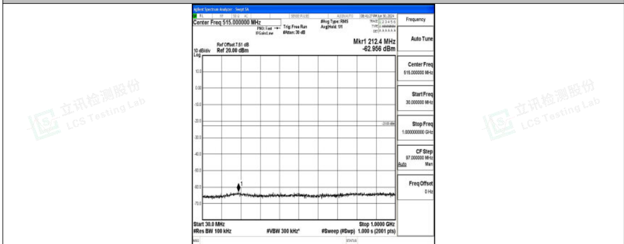
Band25_20MHz_QPSK_26365_1RB#0_30~1000_30~1000
