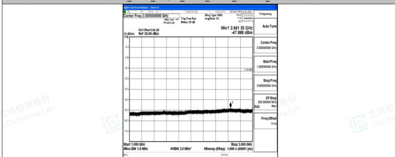
Band13_5MHz_16QAM_23230_1RB#0_1000~3000_1000~3000
