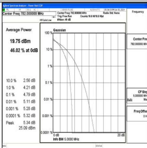
Band13-5MHz-QPSK-23230-1RB#0-PASS
