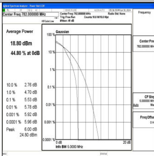
Band13-5MHz-16QAM-23230-1RB#0-PASS
