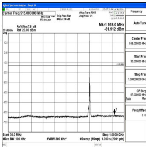
Band12_10MHz_16QAM_23130_1RB#0_30~1000_30~1000
