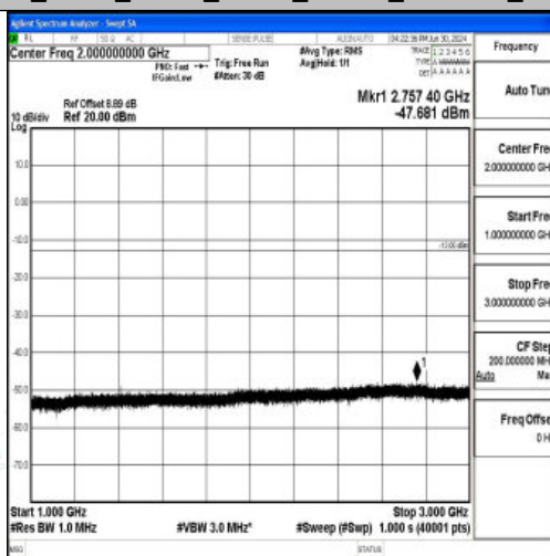
Band12_3MHz_QPSK_23095_1RB#0_1000~3000_1000~3000
