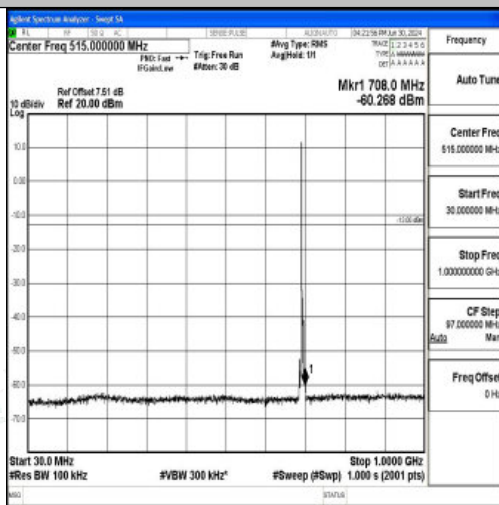
Band12_3MHz_16QAM_23025_1RB#0_30~1000_30~1000
