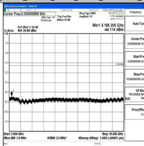
Band12_10MHz_16QAM_23095_1RB#0_3000~10000_3000~10000
