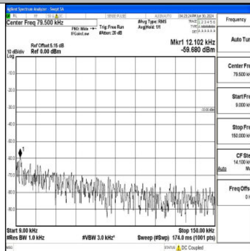
Band12_3MHz_QPSK_23165_1RB#0_0.009~0.15_0.009~0.15
