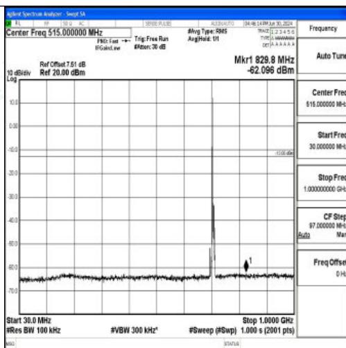
Band12_5MHz_16QAM_23155_1RB#0_30~1000_30~1000
