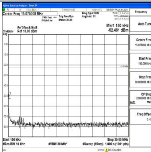
Band12_10MHz_QPSK_23095_1RB#0_0.15~30_0.15~30
