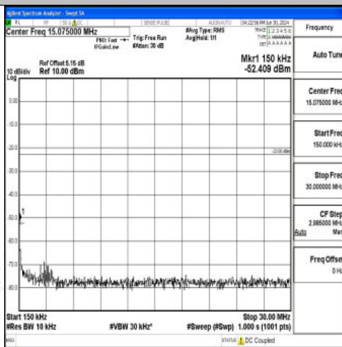
Band12_3MHz_16QAM_23095_1RB#0_0.15~30_0.15~30
