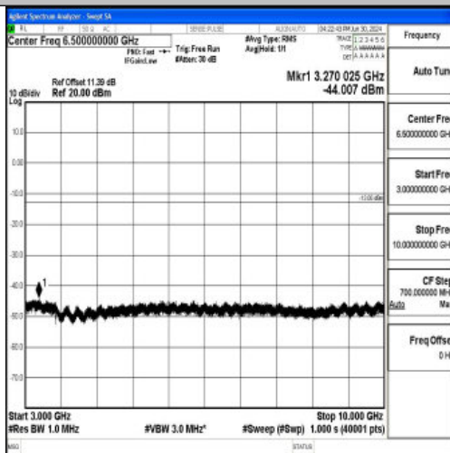
Band12_3MHz_QPSK_23095_1RB#0_3000~10000_3000~10000
