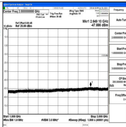
Band12_10MHz_16QAM_23095_1RB#0_1000~3000_1000~3000
