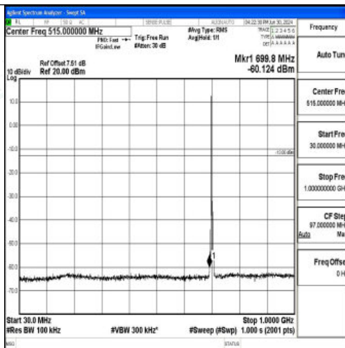
Band12_3MHz_QPSK_23095_1RB#0_30~1000_30~1000
