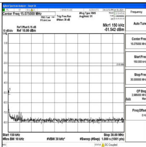
Band12_3MHz_16QAM_23025_1RB#0_0.15~30_0.15~30
