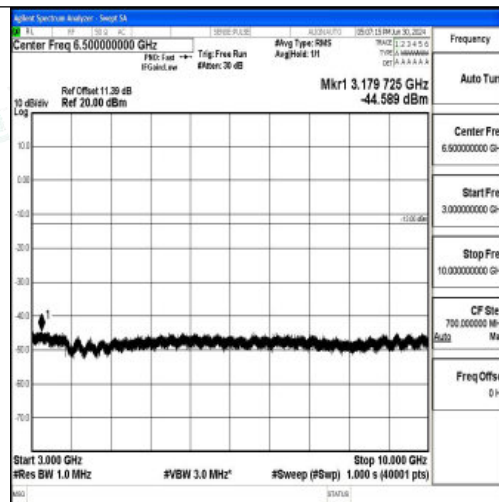
Band12_10MHz_QPSK_23130_1RB#0_3000~10000_3000~10000
