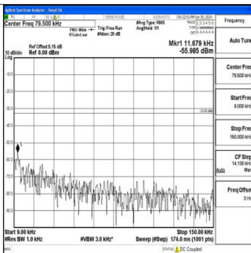
Band12_3MHz_16QAM_23095_1RB#0_0.009~0.15_0.009~0.15
