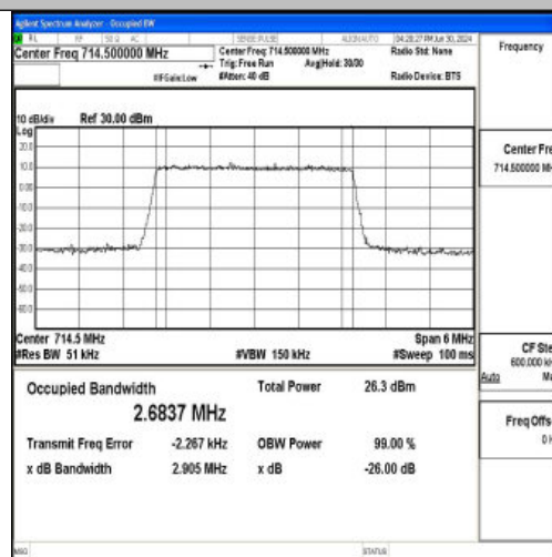
Band12-3MHz-16QAM-23165-15RB#0-PASS
