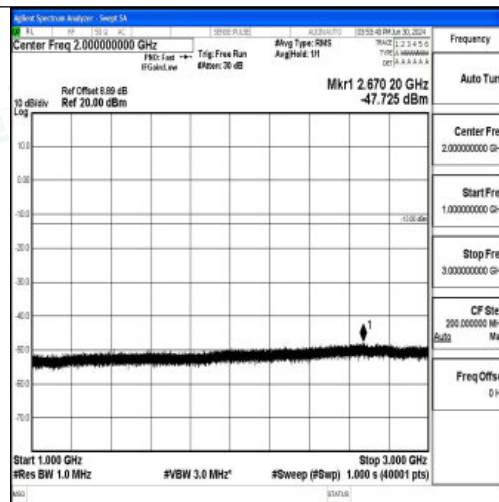
Band12_1.4MHz_16QAM_23095_1RB#0_1000~3000_1000~3000
