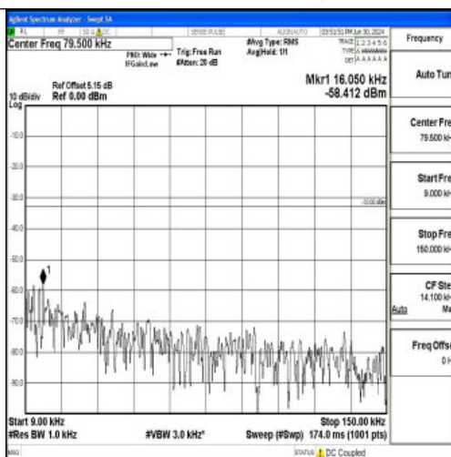
Band12_1.4MHz_QPSK_23017_1RB#0_0.009~0.15_0.009~0.15
