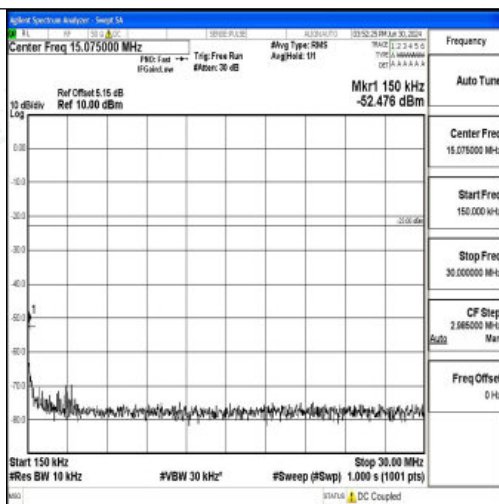
Band12_1.4MHz_16QAM_23017_1RB#0_0.15~30_0.15~30
