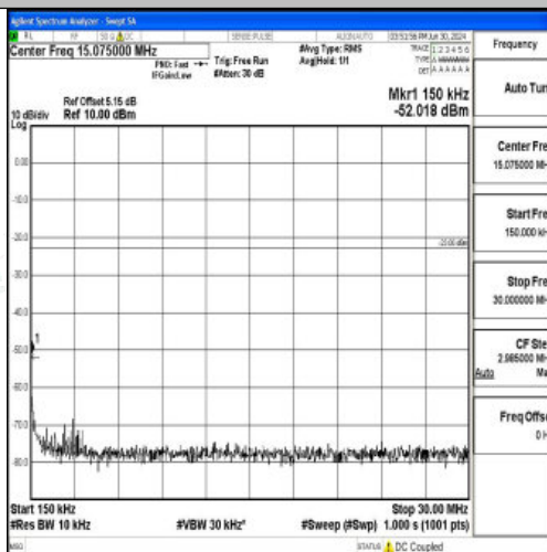
Band12_1.4MHz_QPSK_23017_1RB#0_0.15~30_0.15~30
