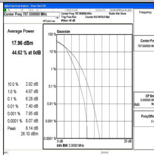
Band12-1.4MHz-16QAM-23095-6RB#0-PASS
