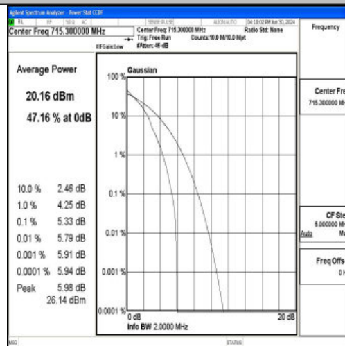
Band12-1.4MHz-QPSK-23173-1RB#0-PASS
