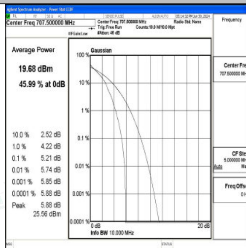
Band12-10MHz-QPSK-23095-1RB#0-PASS
