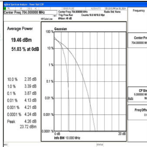
Band12-10MHz-QPSK-23060-1RB#0-PASS
