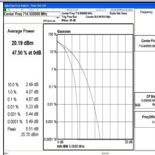
Band12-3MHz-QPSK-23165-1RB#0-PASS
