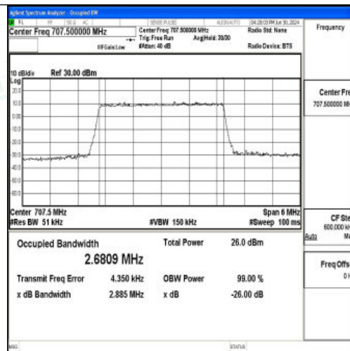
Band12-3MHz-16QAM-23095-15RB#0-PASS
