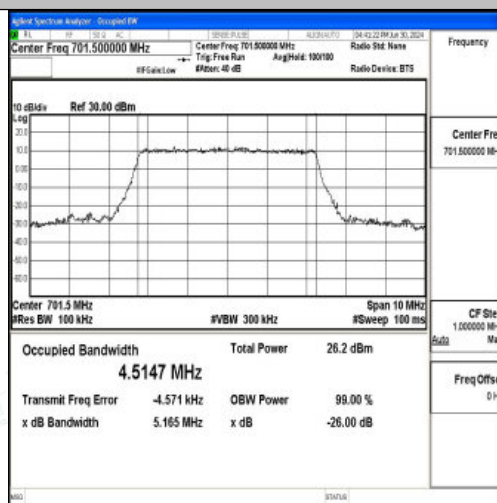
Band12-5MHz-16QAM-23035-25RB#0-PASS
