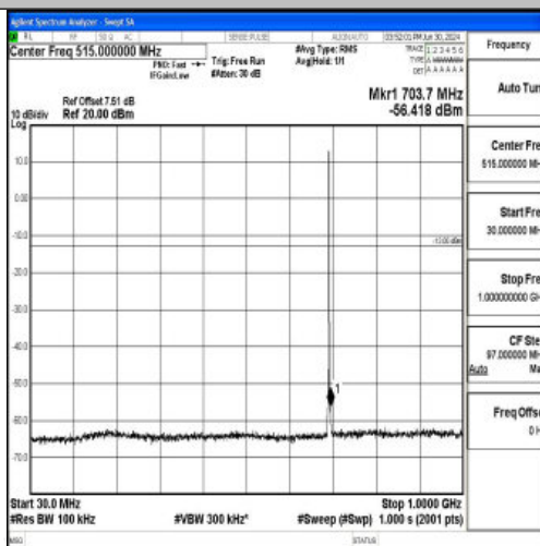
Band12_1.4MHz_QPSK_23017_1RB#0_30~1000_30~1000
