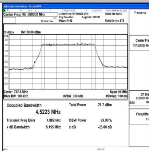
Band12-5MHz-QPSK-23095-25RB#0-PASS
