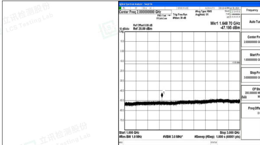
Band5_5MHz_16QAM_20425_1RB#0_1000~3000_1000~3000
