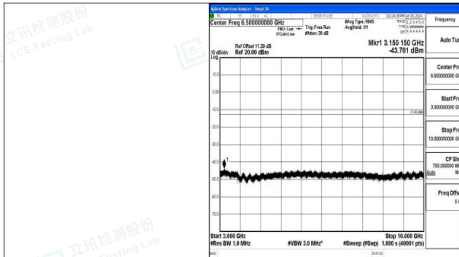
Band5_1.4MHz_16QAM_20643_1RB#0_3000~10000_3000~10000
