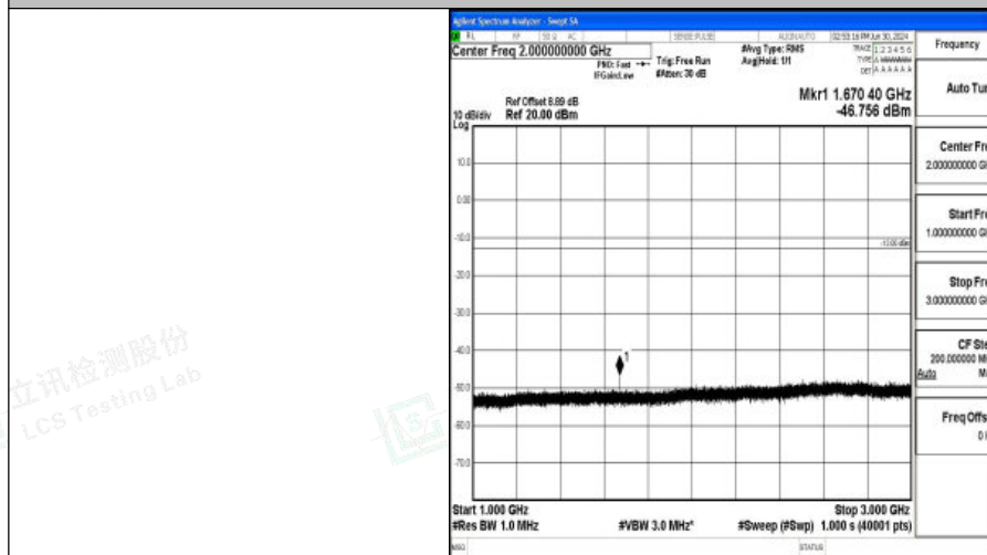
Band5_3MHz_16QAM_20525_1RB#0_1000~3000_1000~3000
