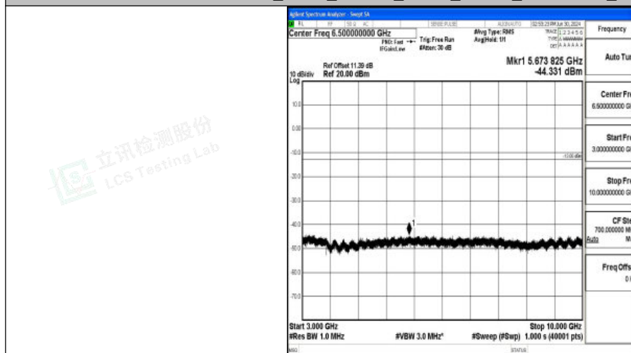
Band5_3MHz_16QAM_20525_1RB#0_3000~10000_3000~10000
