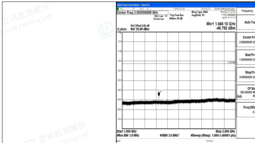
Band5_10MHz_16QAM_20450_1RB#0_1000~3000_1000~3000
