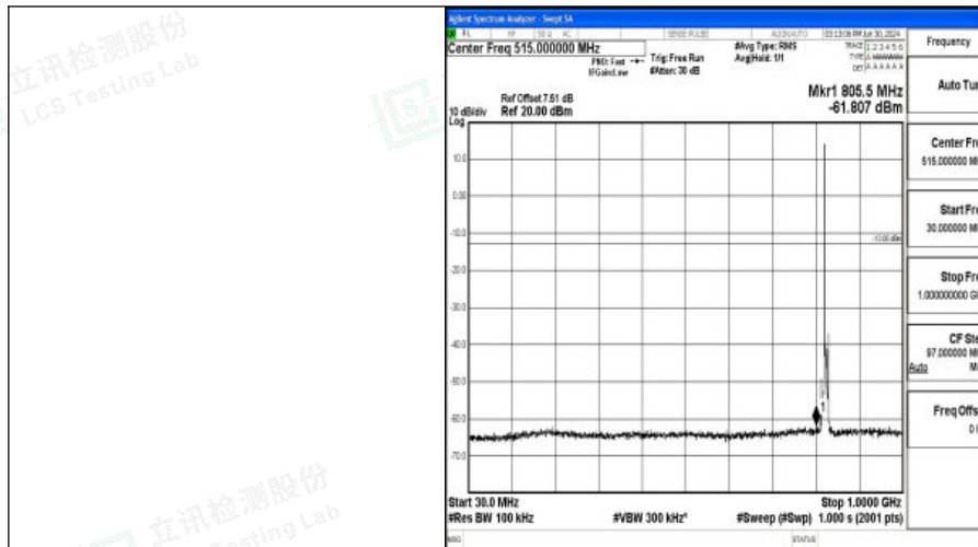
Band5_5MHz_QPSK_20425_1RB#0_30~1000_30~1000
