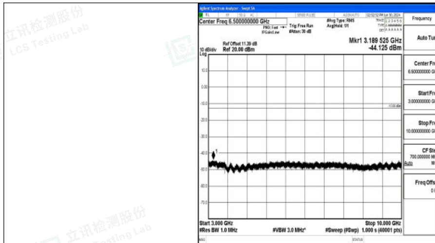
Band5_3MHz_QPSK_20525_1RB#0_3000~10000_3000~10000
