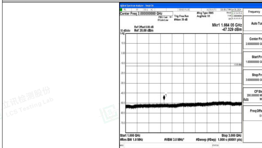
Band5_10MHz_16QAM_20525_1RB#0_1000~3000_1000~3000
