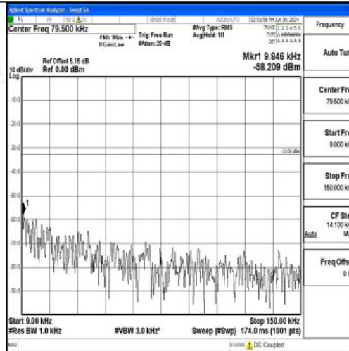
Band5_3MHz_16QAM_20415_1RB#0_0.009~0.15_0.009~0.15
