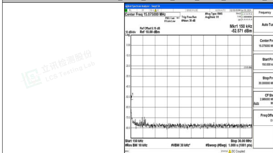
Band5_3MHz_16QAM_20525_1RB#0_0.15~30_0.15~30
