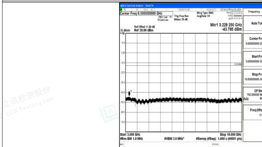
Band5_10MHz_16QAM_20450_1RB#0_3000~10000_3000~10000
