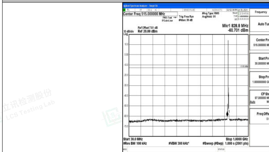
Band5_3MHz_QPSK_20525_1RB#0_30~1000_30~1000
