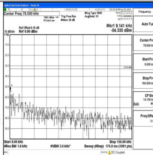
Band5_10MHz_QPSK_20450_1RB#0_0.009~0.15_0.009~0.15
