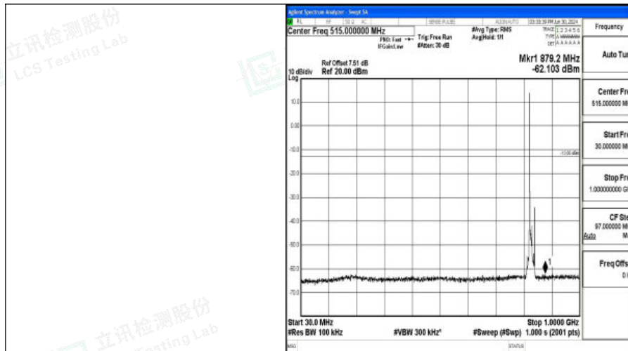
Band5_10MHz_QPSK_20450_1RB#0_30~1000_30~1000
