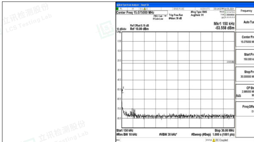
Band5_5MHz_QPSK_20525_1RB#0_0.15~30_0.15~30
