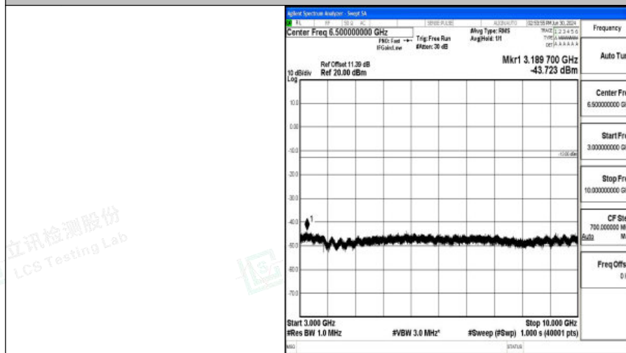
Band5_3MHz_QPSK_20635_1RB#0_3000~10000_3000~10000
