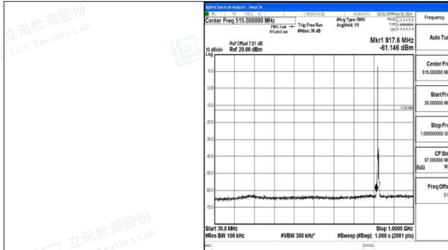
Band5_3MHz_QPSK_20415_1RB#0_30~1000_30~1000
