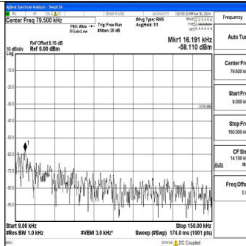
Band5_3MHz_QPSK_20635_1RB#0_0.009~0.15_0.009~0.15
