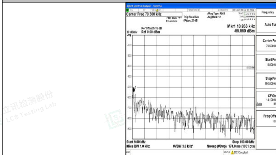
Band5_5MHz_16QAM_20525_1RB#0_0.009~0.15_0.009~0.15
