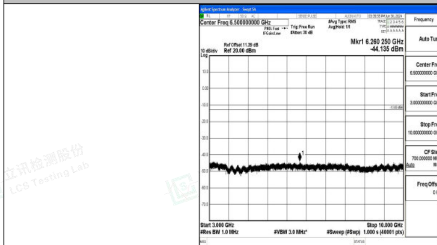
Band5_10MHz_QPSK_20600_1RB#0_3000~10000_3000~10000
