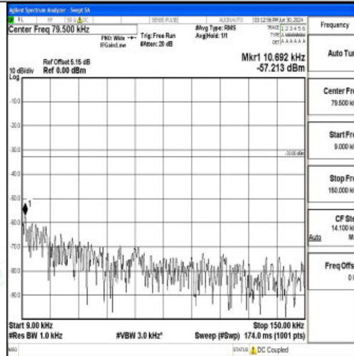
Band5_5MHz_QPSK_20425_1RB#0_0.009~0.15_0.009~0.15
