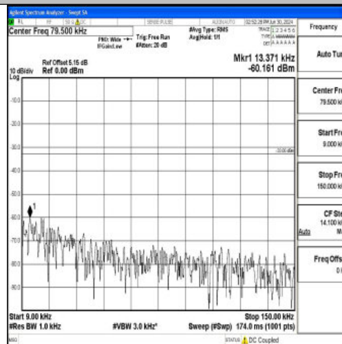
Band5_3MHz_QPSK_20525_1RB#0_0.009~0.15_0.009~0.15
