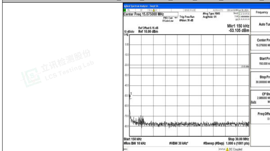
Band5_5MHz_16QAM_20525_1RB#0_0.15~30_0.15~30
