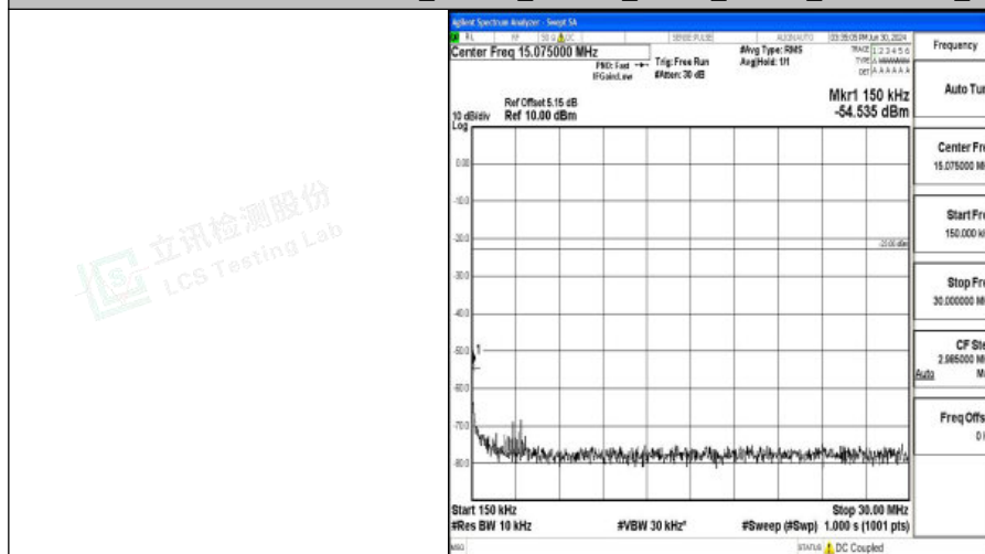
Band5_10MHz_16QAM_20525_1RB#0_0.15~30_0.15~30
