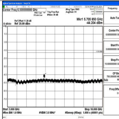
Band5_3MHz_16QAM_20635_1RB#0_3000~10000_3000~10000
