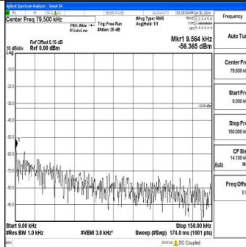
Band5_10MHz_16QAM_20450_1RB#0_0.009~0.15_0.009~0.15
