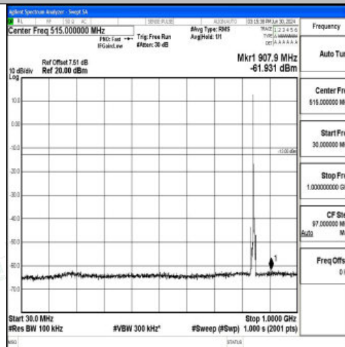
Band5_5MHz_16QAM_20625_1RB#0_30~1000_30~1000
