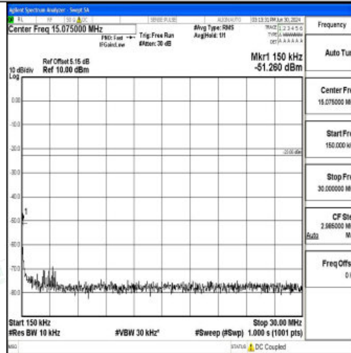
Band5_5MHz_16QAM_20425_1RB#0_0.15~30_0.15~30
