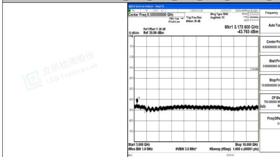
Band5_3MHz_QPSK_20415_1RB#0_3000~10000_3000~10000
