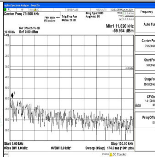
Band5_3MHz_QPSK_20415_1RB#0_0.009~0.15_0.009~0.15
