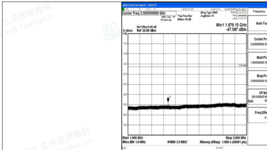
Band5_10MHz_QPSK_20600_1RB#0_1000~3000_1000~3000
