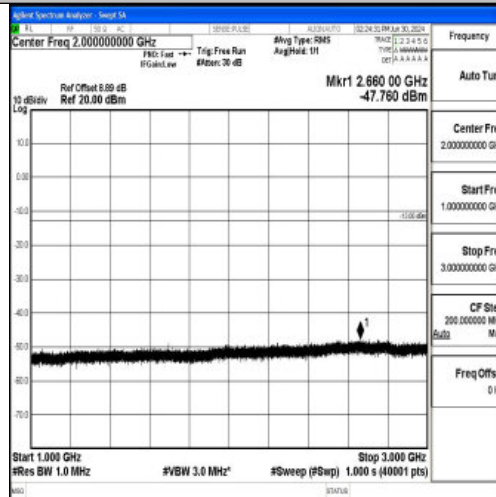
Band5_1.4MHz_16QAM_20643_1RB#0_1000~3000_1000~3000
