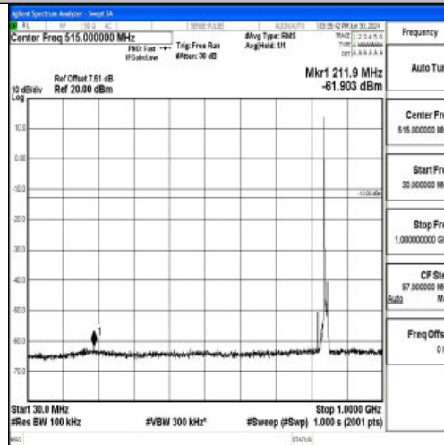
Band5_10MHz_QPSK_20600_1RB#0_30~1000_30~1000
