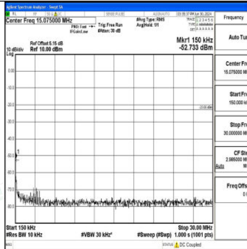
Band5_10MHz_QPSK_20600_1RB#0_0.15~30_0.15~30
