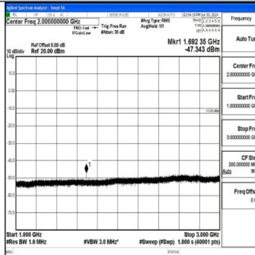
Band5_3MHz_16QAM_20635_1RB#0_1000~3000_1000~3000
