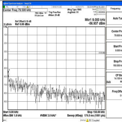
Band5_1.4MHz_QPSK_20643_1RB#0_0.009~0.15_0.009~0.15
