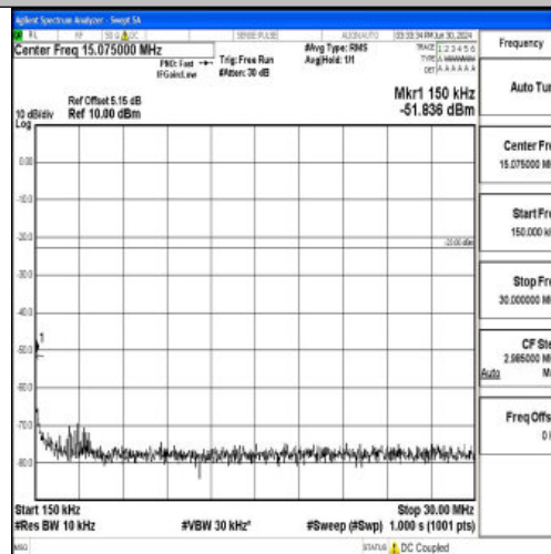
Band5_10MHz_QPSK_20450_1RB#0_0.15~30_0.15~30
