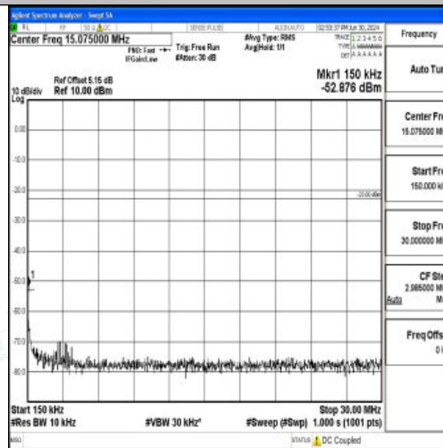
Band5_3MHz_QPSK_20635_1RB#0_0.15~30_0.15~30
