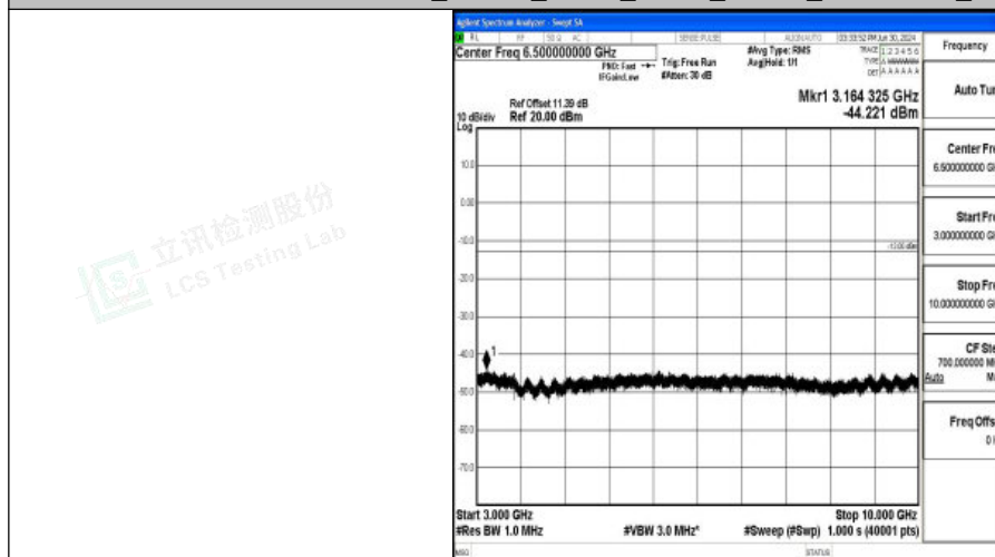
Band5_10MHz_QPSK_20450_1RB#0_3000~10000_3000~10000
