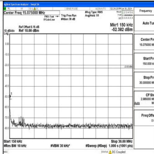
Band5_1.4MHz_16QAM_20643_1RB#0_0.15~30_0.15~30
