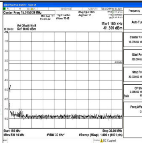
Band5_5MHz_QPSK_20625_1RB#0_0.15~30_0.15~30
