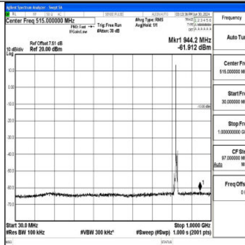
Band5_5MHz_16QAM_20425_1RB#0_30~1000_30~1000
