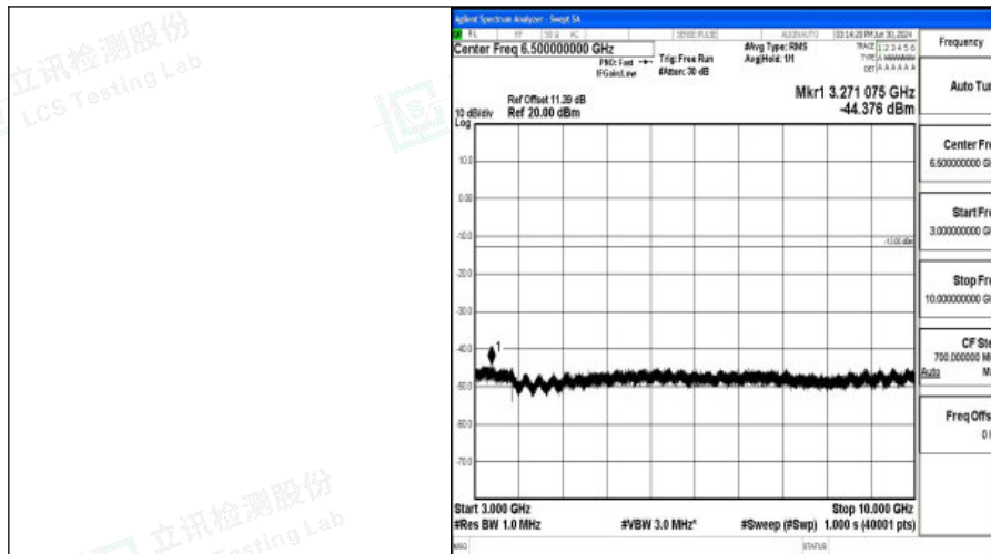
Band5_5MHz_QPSK_20525_1RB#0_3000~10000_3000~10000
