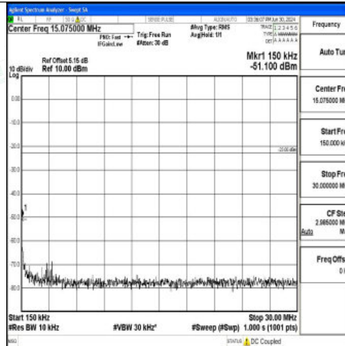
Band5_10MHz_16QAM_20600_1RB#0_0.15~30_0.15~30
