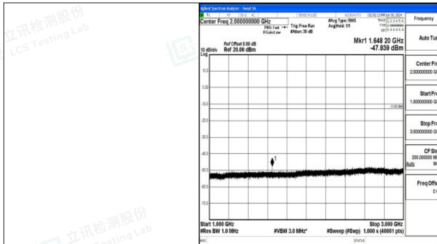
Band5_3MHz_16QAM_20415_1RB#0_1000~3000_1000~3000
