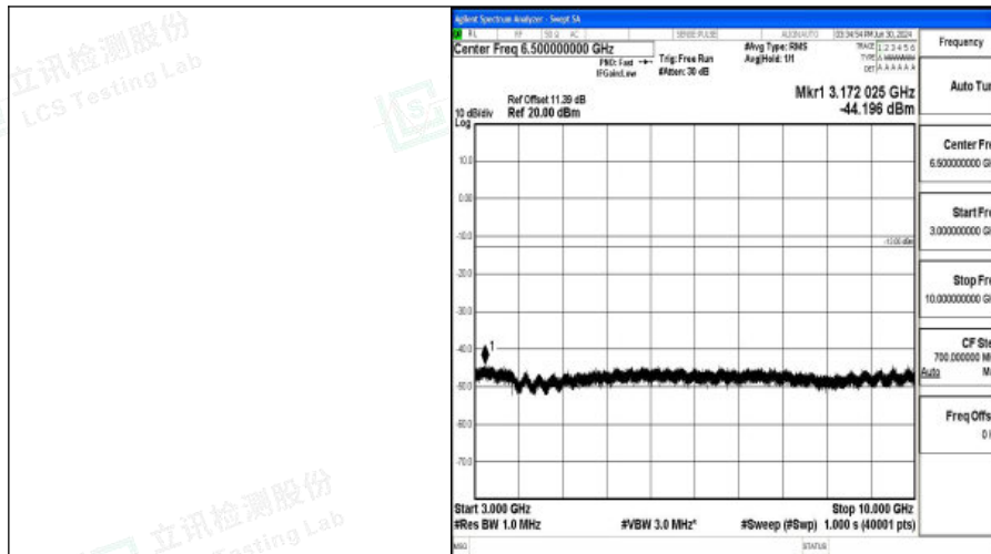
Band5_10MHz_QPSK_20525_1RB#0_3000~10000_3000~10000
