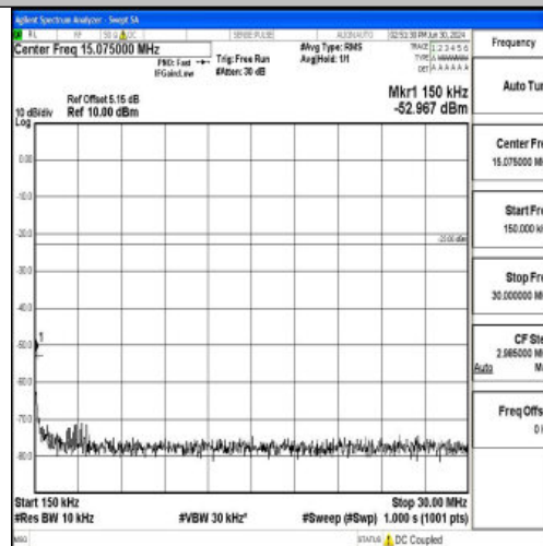
Band5_3MHz_QPSK_20415_1RB#0_0.15~30_0.15~30
