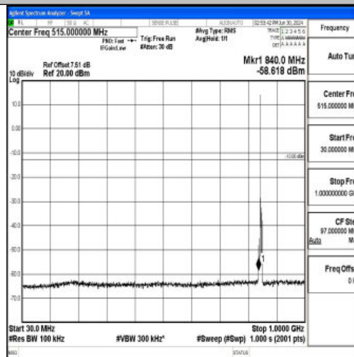
Band5_3MHz_QPSK_20635_1RB#0_30~1000_30~1000
