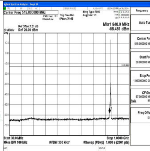
Band5_3MHz_16QAM_20635_1RB#0_30~1000_30~1000
