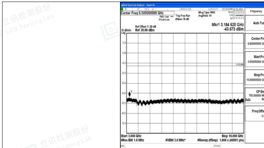
Band5_5MHz_16QAM_20625_1RB#0_3000~10000_3000~10000
