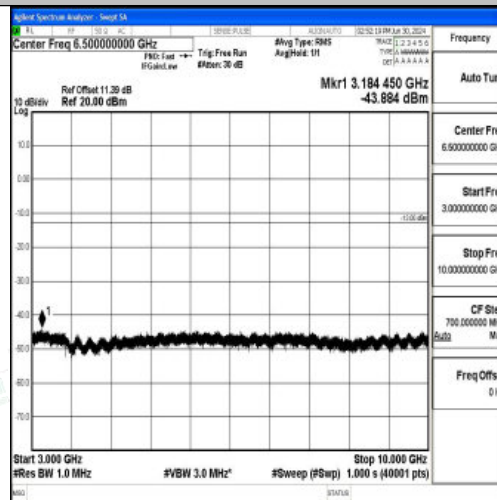
Band5_3MHz_16QAM_20415_1RB#0_3000~10000_3000~10000
