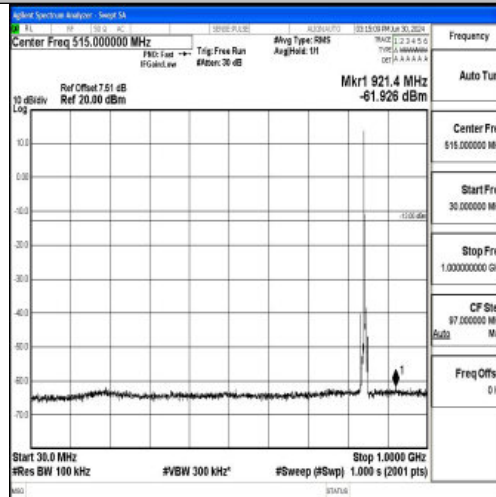
Band5_5MHz_QPSK_20625_1RB#0_30~1000_30~1000
