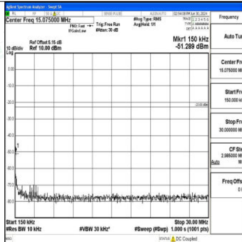
Band5_3MHz_16QAM_20635_1RB#0_0.15~30_0.15~30
