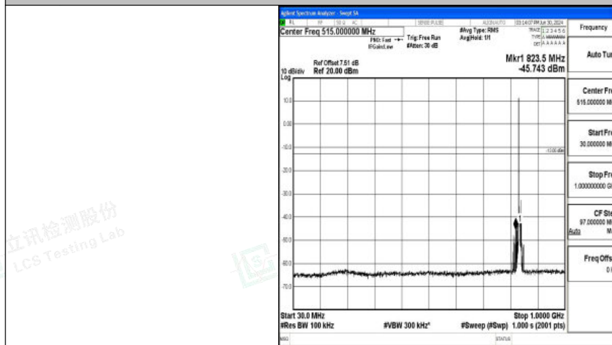
Band5_5MHz_QPSK_20525_1RB#0_30~1000_30~1000
