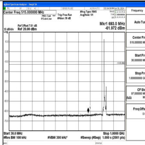
Band5_10MHz_16QAM_20450_1RB#0_30~1000_30~1000
