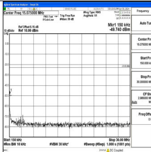
Band5_5MHz_QPSK_20425_1RB#0_0.15~30_0.15~30
