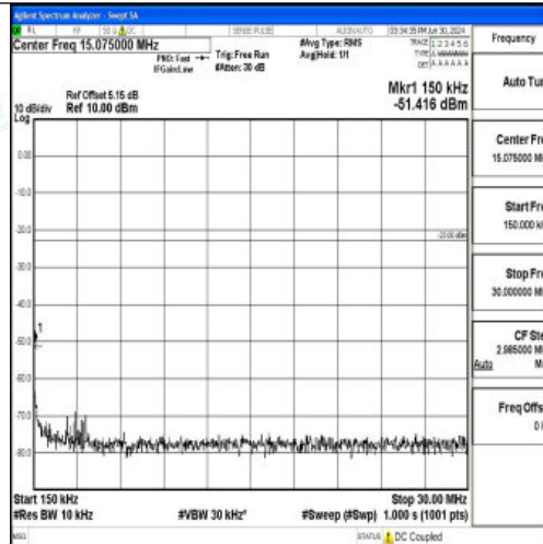
Band5_10MHz_QPSK_20525_1RB#0_0.15~30_0.15~30
