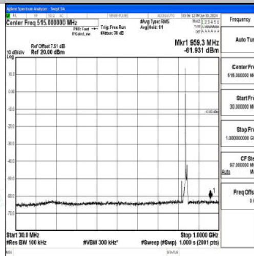
Band5_10MHz_16QAM_20600_1RB#0_30~1000_30~1000
