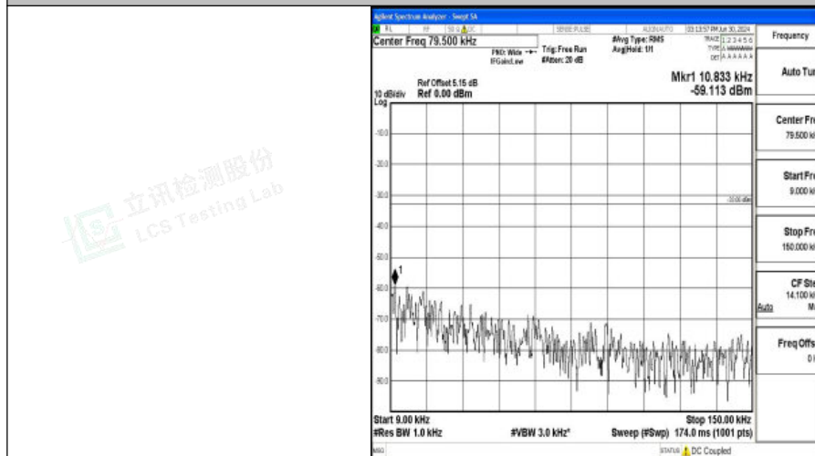
Band5_5MHz_QPSK_20525_1RB#0_0.009~0.15_0.009~0.15
