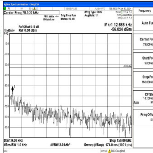
Band5_10MHz_QPSK_20600_1RB#0_0.009~0.15_0.009~0.15
