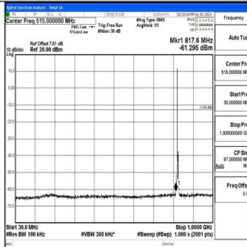
Band5_3MHz_16QAM_20415_1RB#0_30~1000_30~1000
