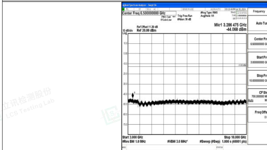
Band5_5MHz_16QAM_20425_1RB#0_3000~10000_3000~10000
