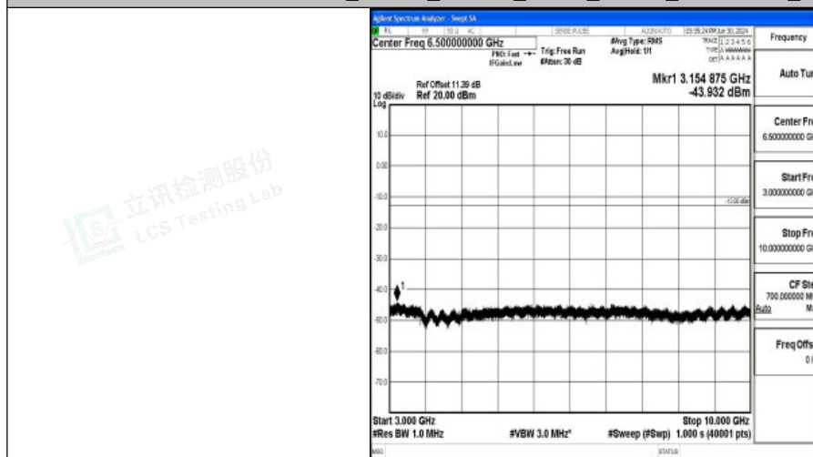
Band5_10MHz_16QAM_20525_1RB#0_3000~10000_3000~10000
