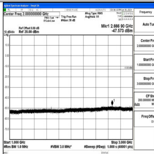
Band5_10MHz_16QAM_20600_1RB#0_1000~3000_1000~3000
