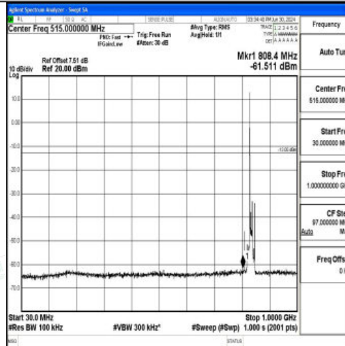
Band5_10MHz_QPSK_20525_1RB#0_30~1000_30~1000
