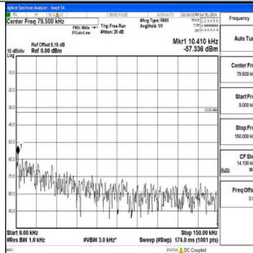
Band5_1.4MHz_16QAM_20643_1RB#0_0.009~0.15_0.009~0.15
