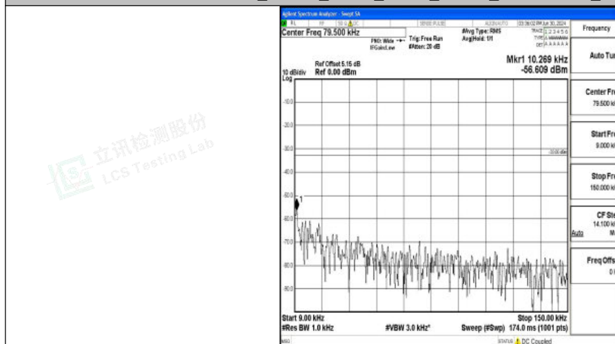
Band5_10MHz_16QAM_20600_1RB#0_0.009~0.15_0.009~0.15
