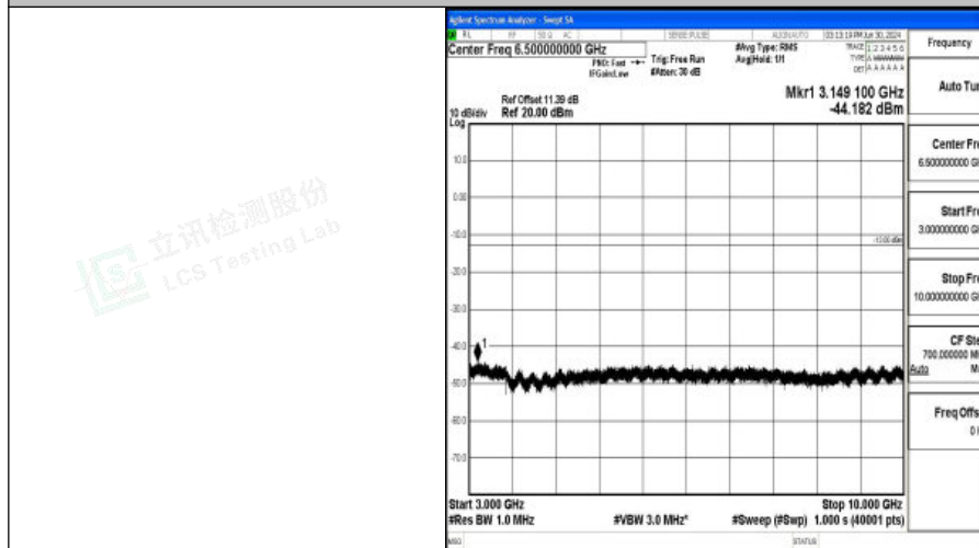
Band5_5MHz_QPSK_20425_1RB#0_3000~10000_3000~10000
