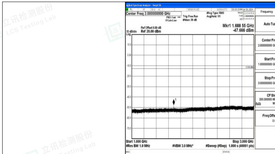
Band5_5MHz_QPSK_20625_1RB#0_1000~3000_1000~3000
