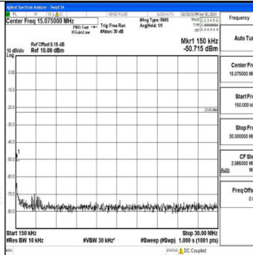
Band5_3MHz_16QAM_20415_1RB#0_0.15~30_0.15~30
