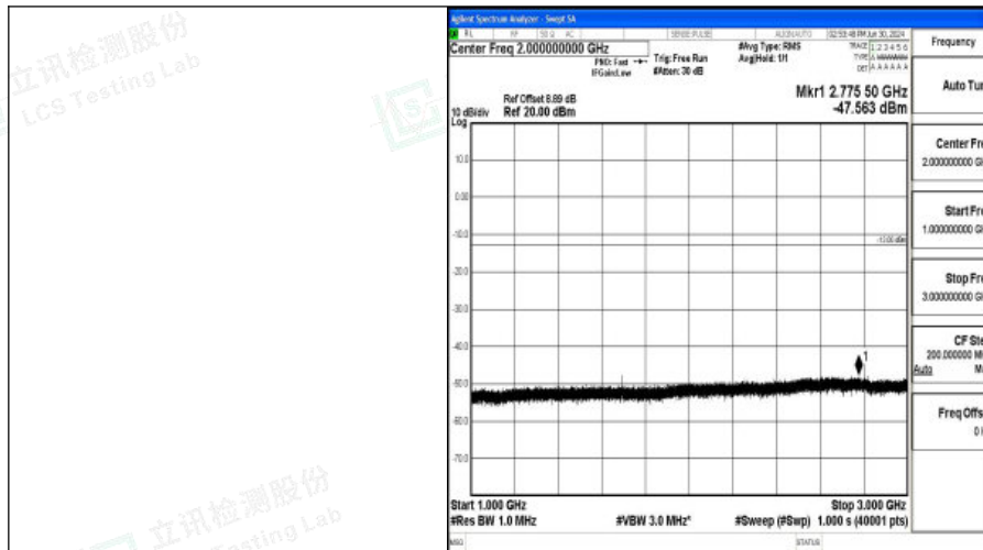
Band5_3MHz_QPSK_20635_1RB#0_1000~3000_1000~3000
