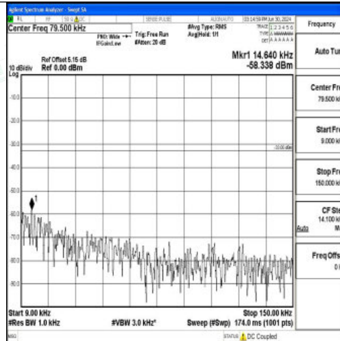
Band5_5MHz_QPSK_20625_1RB#0_0.009~0.15_0.009~0.15
