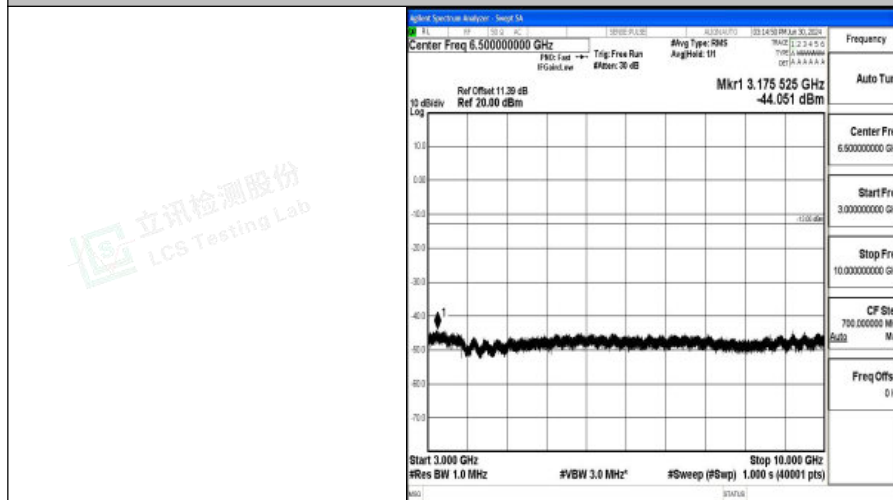
Band5_5MHz_16QAM_20525_1RB#0_3000~10000_3000~10000
