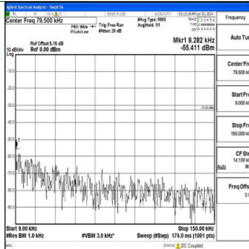
Band5_5MHz_16QAM_20425_1RB#0_0.009~0.15_0.009~0.15
