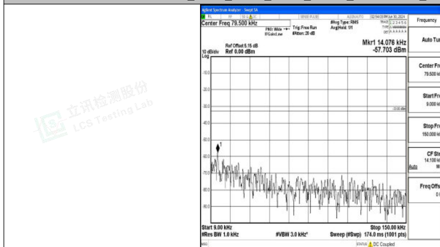
Band5_3MHz_16QAM_20635_1RB#0_0.009~0.15_0.009~0.15
