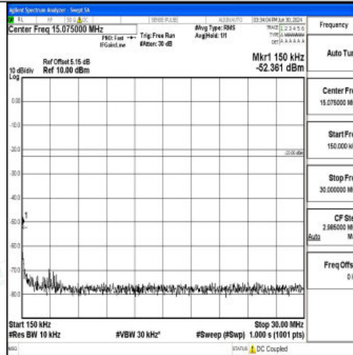
Band5_10MHz_16QAM_20450_1RB#0_0.15~30_0.15~30
