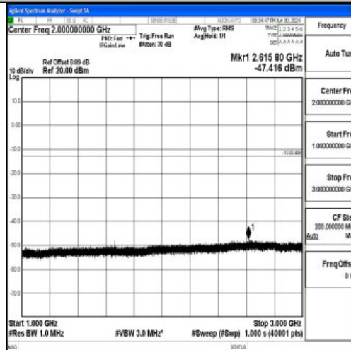
Band5_10MHz_QPSK_20525_1RB#0_1000~3000_1000~3000
