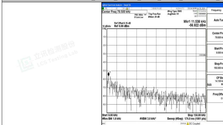
Band5_10MHz_QPSK_20525_1RB#0_0.009~0.15_0.009~0.15
