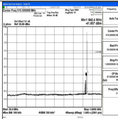
Band5_1.4MHz_16QAM_20643_1RB#0_30~1000_30~1000
