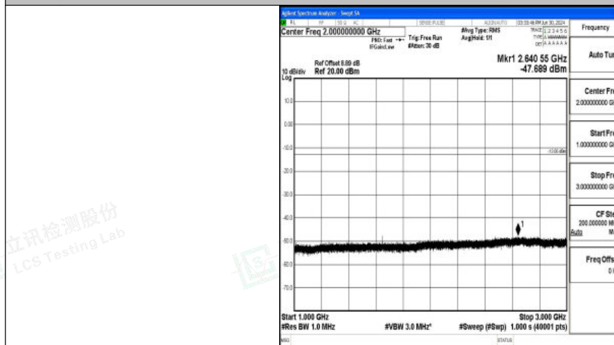
Band5_10MHz_QPSK_20450_1RB#0_1000~3000_1000~3000
