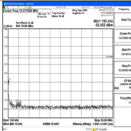
Band5_5MHz_16QAM_20625_1RB#0_0.15~30_0.15~30
