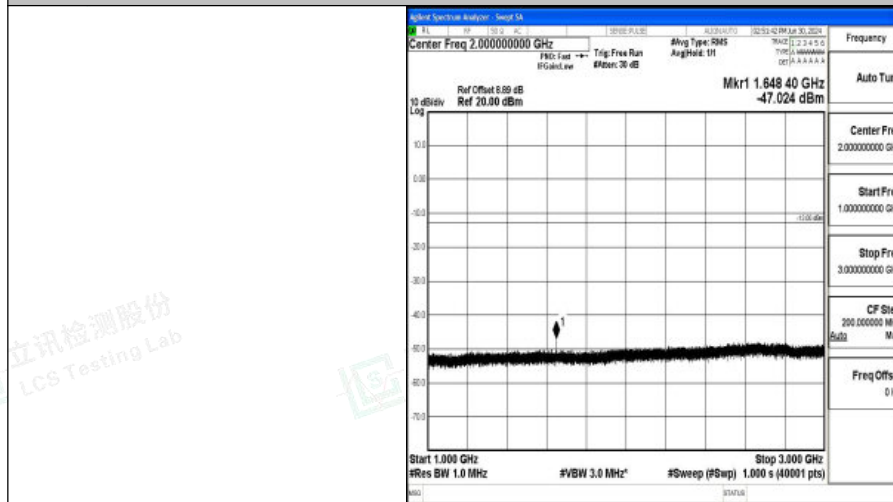
Band5_3MHz_QPSK_20415_1RB#0_1000~3000_1000~3000
