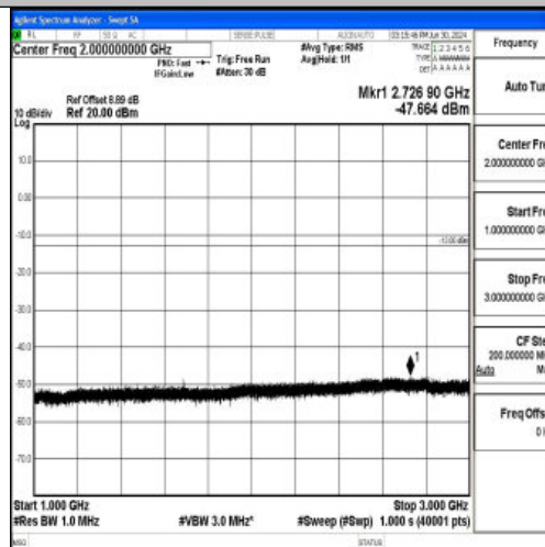
Band5_5MHz_16QAM_20625_1RB#0_1000~3000_1000~3000
