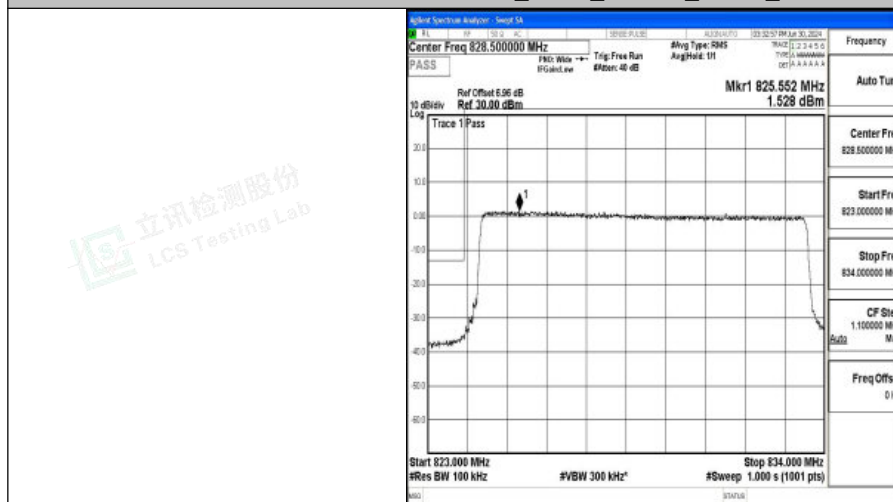
Band5_10MHz_QPSK_20450_50RB#0
