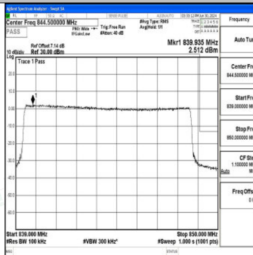
Band5_10MHz_QPSK_20600_50RB#0
