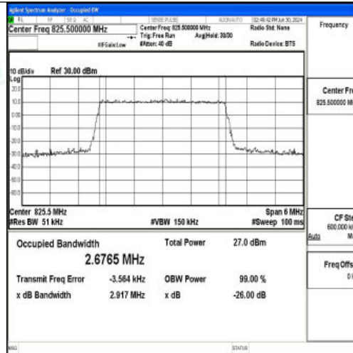
Band5-3MHz-QPSK-20415-15RB#0-PASS
