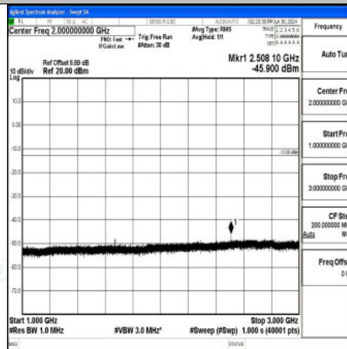
Band5_1.4MHz_16QAM_20525_1RB#0_1000~3000_1000~3000
