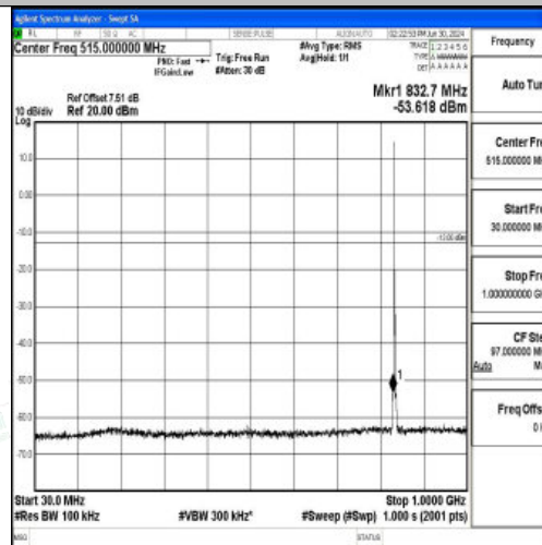
Band5_1.4MHz_QPSK_20525_1RB#0_30~1000_30~1000
