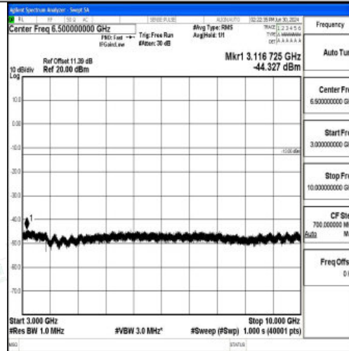
Band5_1.4MHz_16QAM_20407_1RB#0_3000~10000_3000~10000
