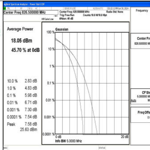
Band5-5MHz-16QAM-20425-25RB#0-PASS
