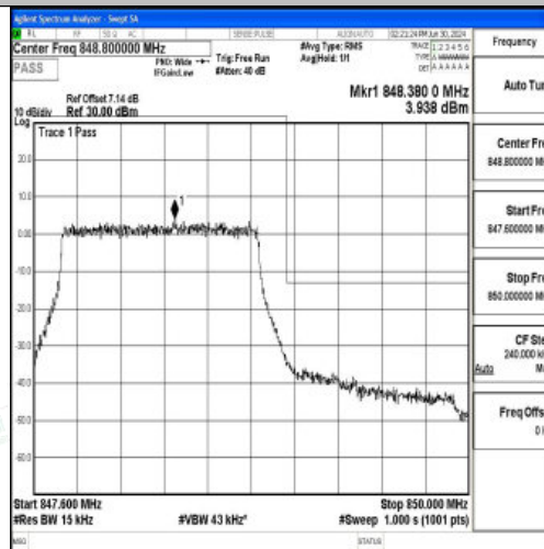
Band5_1.4MHz_QPSK_20643_6RB#0
