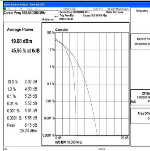
Band5-10MHz-16QAM-20525-1RB#0-PASS
