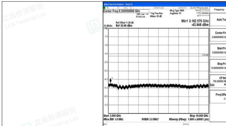
Band5_1.4MHz_QPSK_20525_1RB#0_3000~10000_3000~10000
