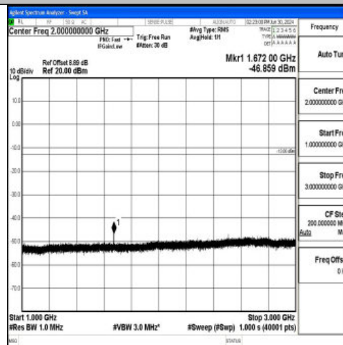
Band5_1.4MHz_QPSK_20525_1RB#0_1000~3000_1000~3000
