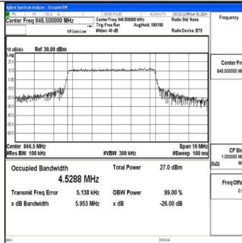
Band5-5MHz-16QAM-20625-25RB#0-PASS
