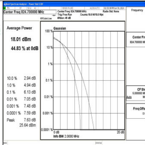
Band5-1.4MHz-16QAM-20407-6RB#0-PASS
