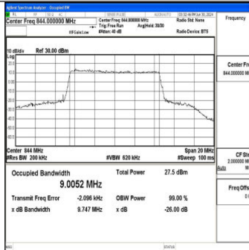
Band5-10MHz-16QAM-20600-50RB#0-PASS
