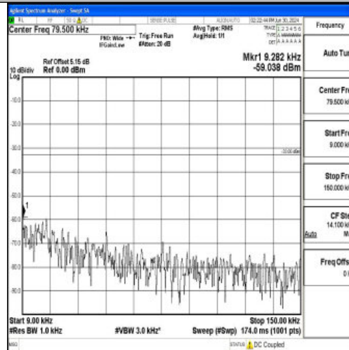
Band5_1.4MHz_QPSK_20525_1RB#0_0.009~0.15_0.009~0.15
