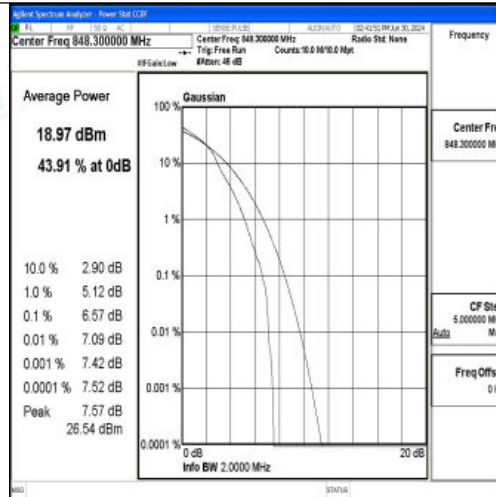
Band5-1.4MHz-16QAM-20643-1RB#0-PASS
