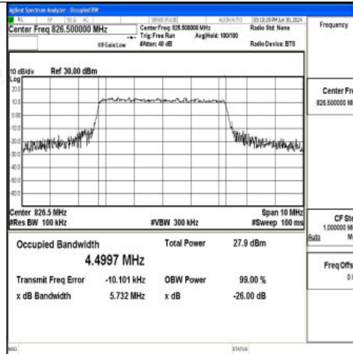
Band5-5MHz-QPSK-20425-25RB#0-PASS
