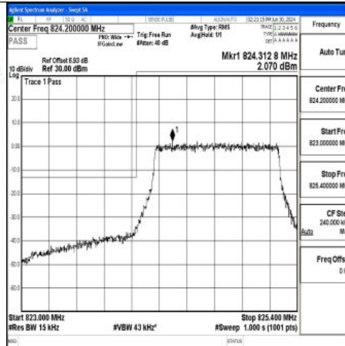
Band5_1.4MHz_16QAM_20407_6RB#0
