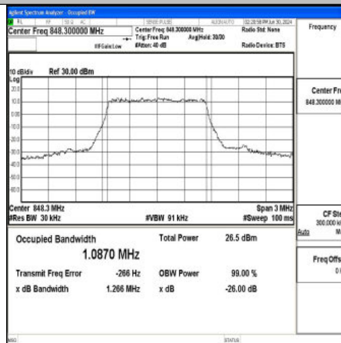
Band5-1.4MHz-16QAM-20643-6RB#0-PASS
