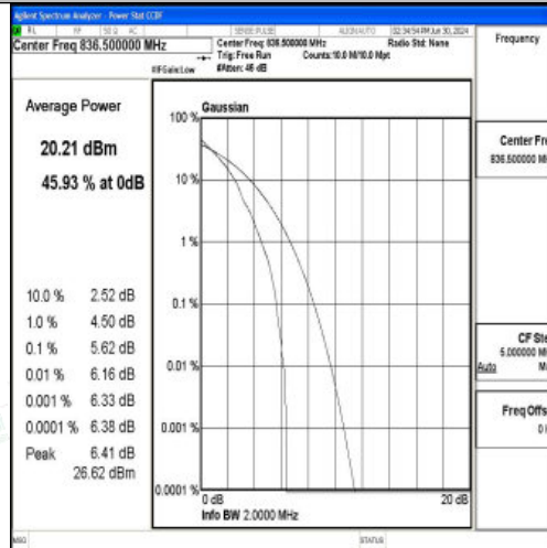
Band5-1.4MHz-QPSK-20525-1RB#0-PASS
