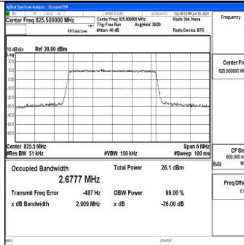
Band5-3MHz-16QAM-20415-15RB#0-PASS
