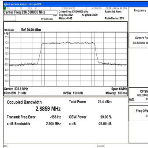
Band5-3MHz-16QAM-20525-15RB#0-PASS
