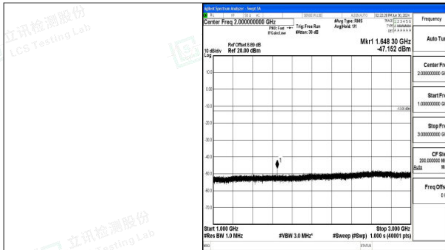
Band5_1.4MHz_16QAM_20407_1RB#0_1000~3000_1000~3000
