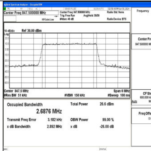
Band5-3MHz-16QAM-20635-15RB#0-PASS
