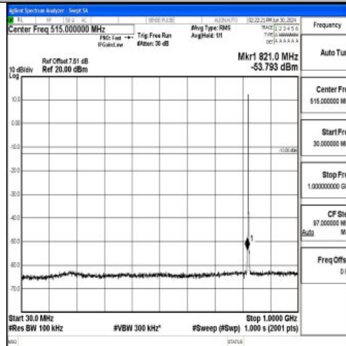
Band5_1.4MHz_16QAM_20407_1RB#0_30~1000_30~1000
