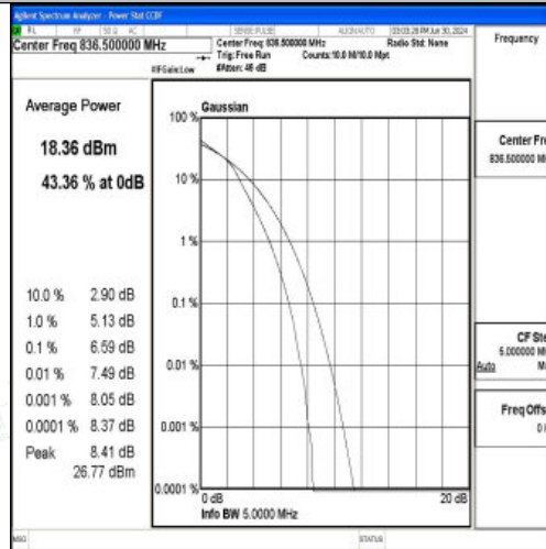
Band5-3MHz-16QAM-20525-15RB#0-PASS
