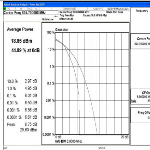
Band5-1.4MHz-16QAM-20407-1RB#0-PASS
