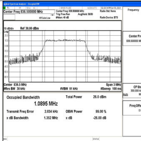
Band5-1.4MHz-16QAM-20525-6RB#0-PASS
