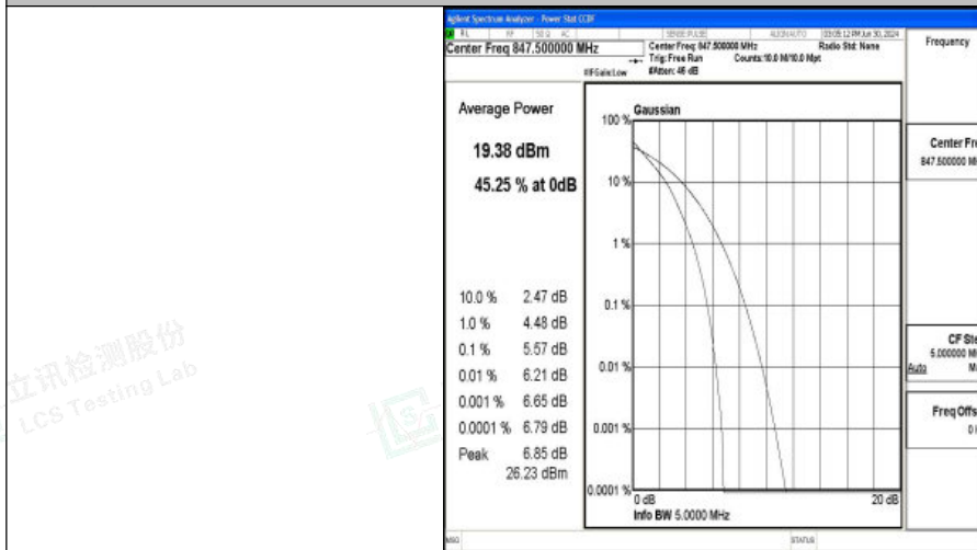
Band5-3MHz-QPSK-20635-15RB#0-PASS
