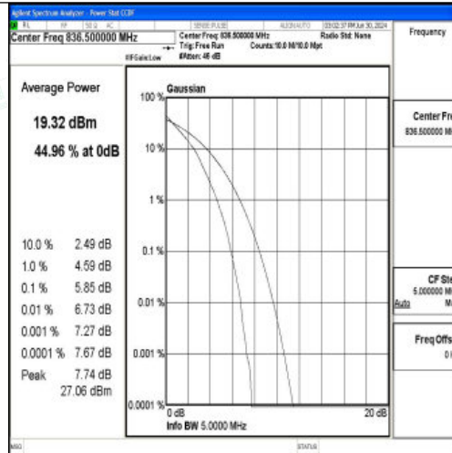
Band5-3MHz-QPSK-20525-15RB#0-PASS
