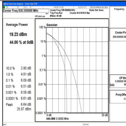
Band5-5MHz-16QAM-20525-1RB#0-PASS
