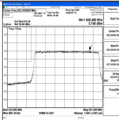
Band5_3MHz_16QAM_20415_15RB#0
