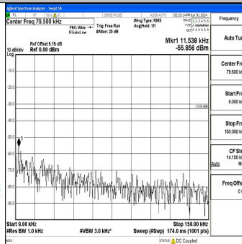
Band5_1.4MHz_16QAM_20525_1RB#0_0.009~0.15_0.009~0.15
