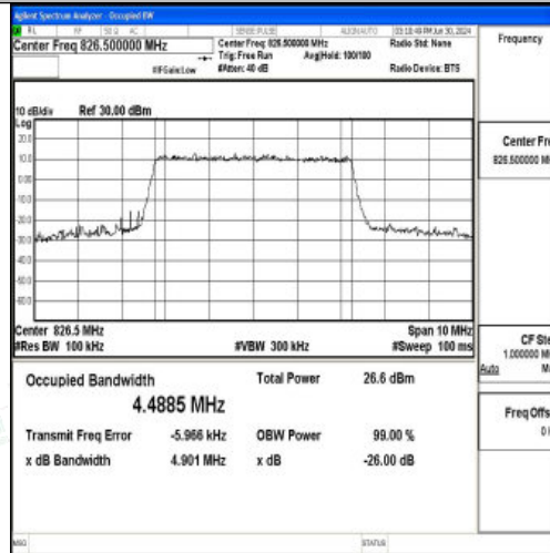
Band5-5MHz-16QAM-20425-25RB#0-PASS
