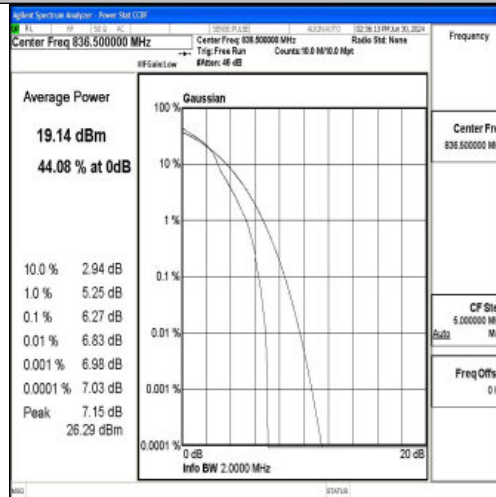
Band5-1.4MHz-16QAM-20525-1RB#0-PASS
