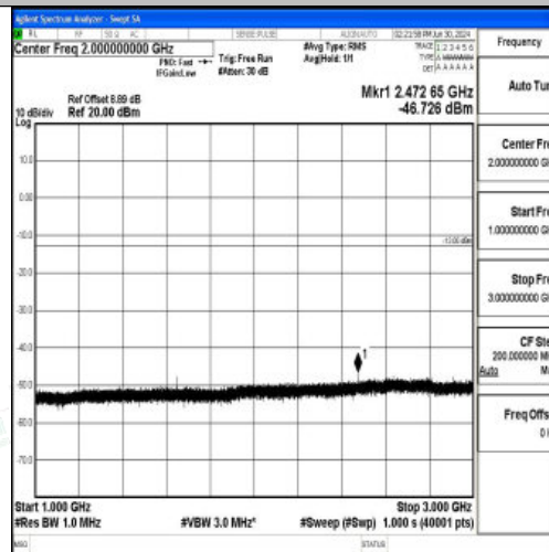
Band5_1.4MHz_QPSK_20407_1RB#0_1000~3000_1000~3000
