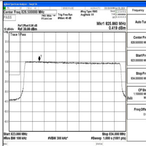
Band5_10MHz_16QAM_20450_50RB#0
