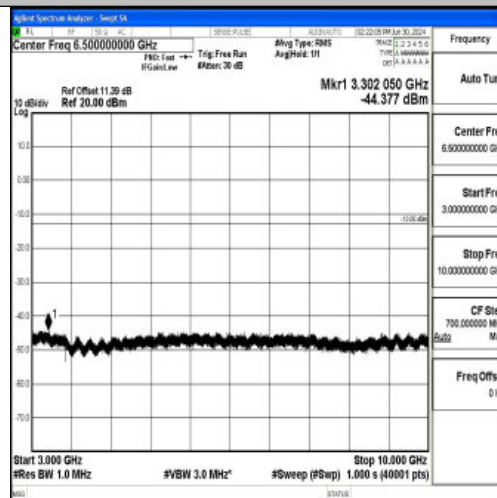
Band5_1.4MHz_QPSK_20407_1RB#0_3000~10000_3000~10000
