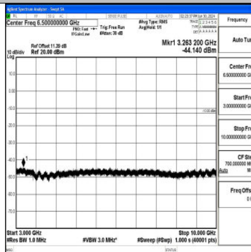
Band5_1.4MHz_16QAM_20525_1RB#0_3000~10000_3000~10000
