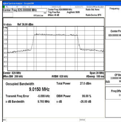
Band5-10MHz-16QAM-20450-50RB#0-PASS
