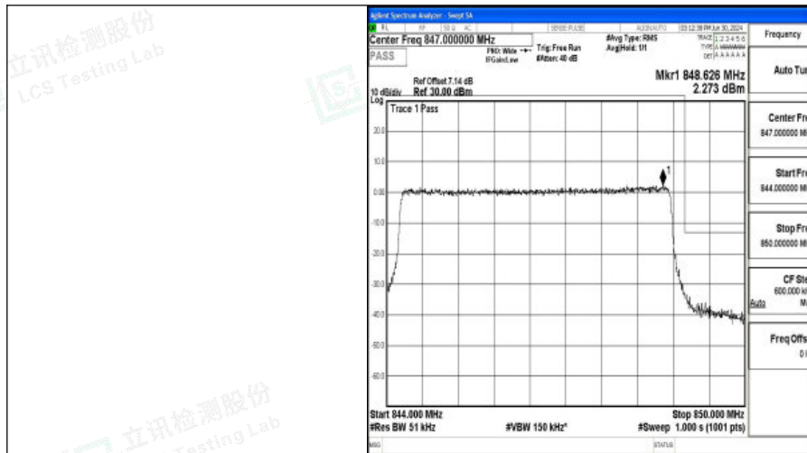
Band5_5MHz_QPSK_20625_25RB#0
