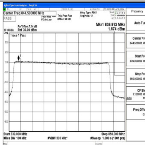
Band5_10MHz_16QAM_20600_50RB#0
