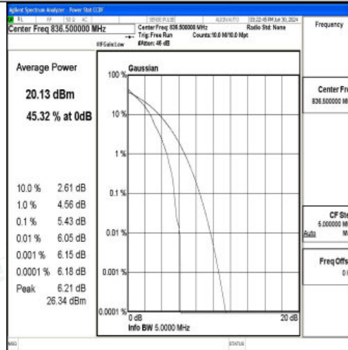
Band5-5MHz-QPSK-20525-1RB#0-PASS
