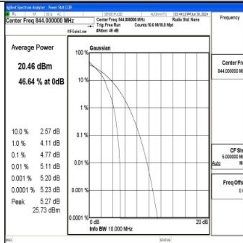
Band5-10MHz-QPSK-20600-1RB#0-PASS
