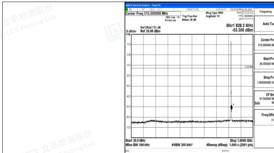
Band5_1.4MHz_QPSK_20407_1RB#0_30~1000_30~1000
