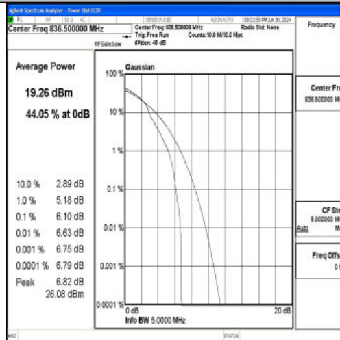
Band5-3MHz-16QAM-20525-1RB#0-PASS
