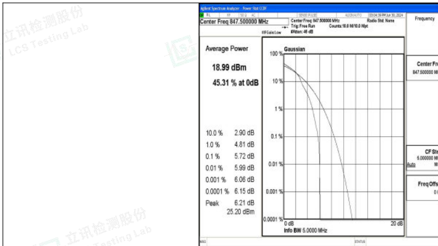
Band5-3MHz-16QAM-20635-1RB#0-PASS
