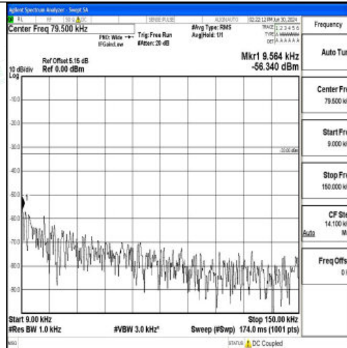
Band5_1.4MHz_16QAM_20407_1RB#0_0.009~0.15_0.009~0.15
