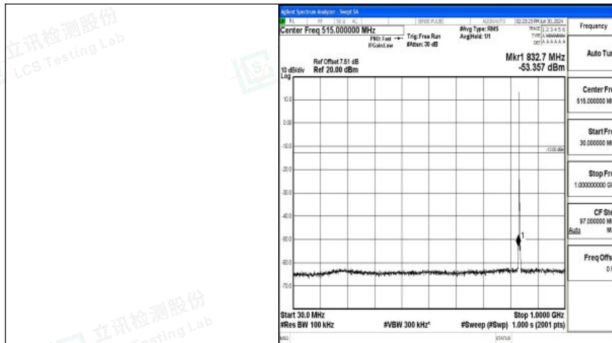
Band5_1.4MHz_16QAM_20525_1RB#0_30~1000_30~1000
