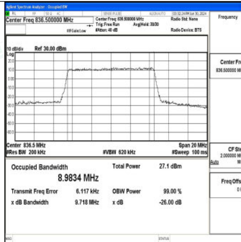
Band5-10MHz-16QAM-20525-50RB#0-PASS
