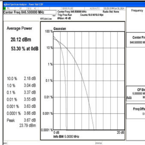
Band5-5MHz-QPSK-20625-1RB#0-PASS
