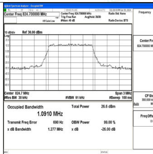
Band5-1.4MHz-QPSK-20407-6RB#0-PASS
