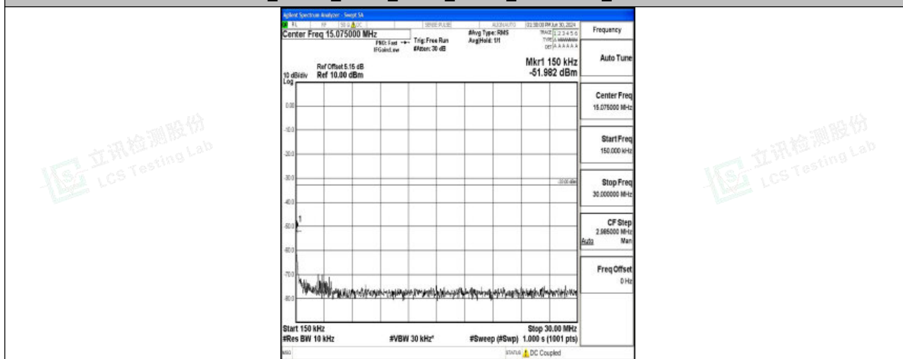
Band4_10MHz_QPSK_20350_1RB#0_0.15~30_0.15~30
