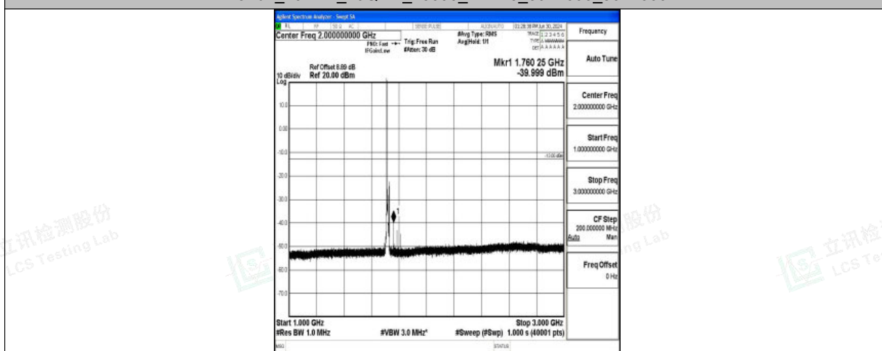
Band4_10MHz_16QAM_20000_1RB#0_1000~3000_1000~3000
