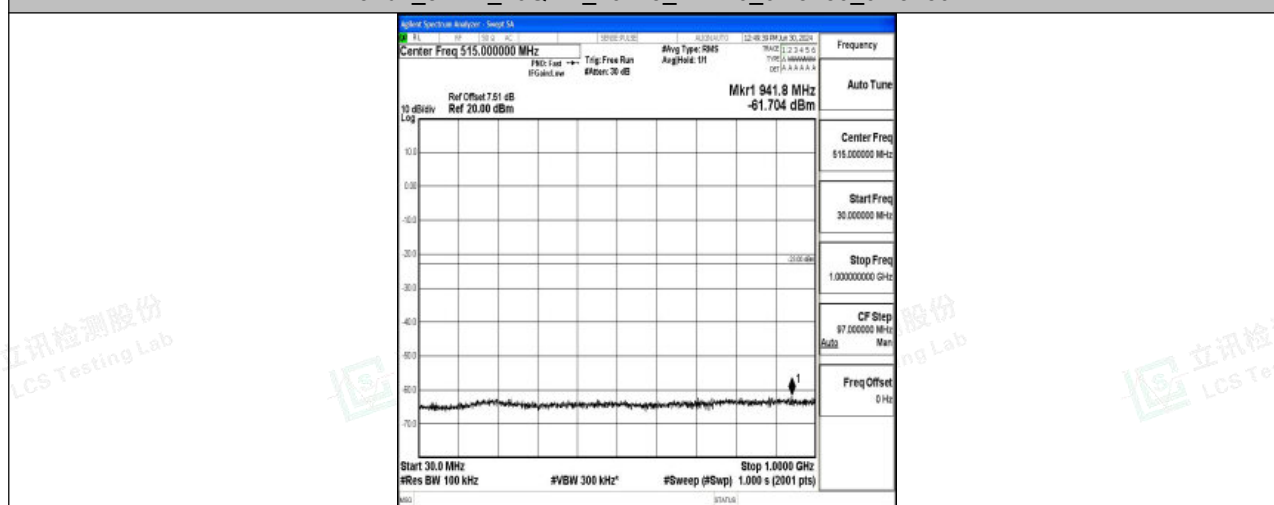
Band4_3MHz_16QAM_20175_1RB#0_30~1000_30~1000
