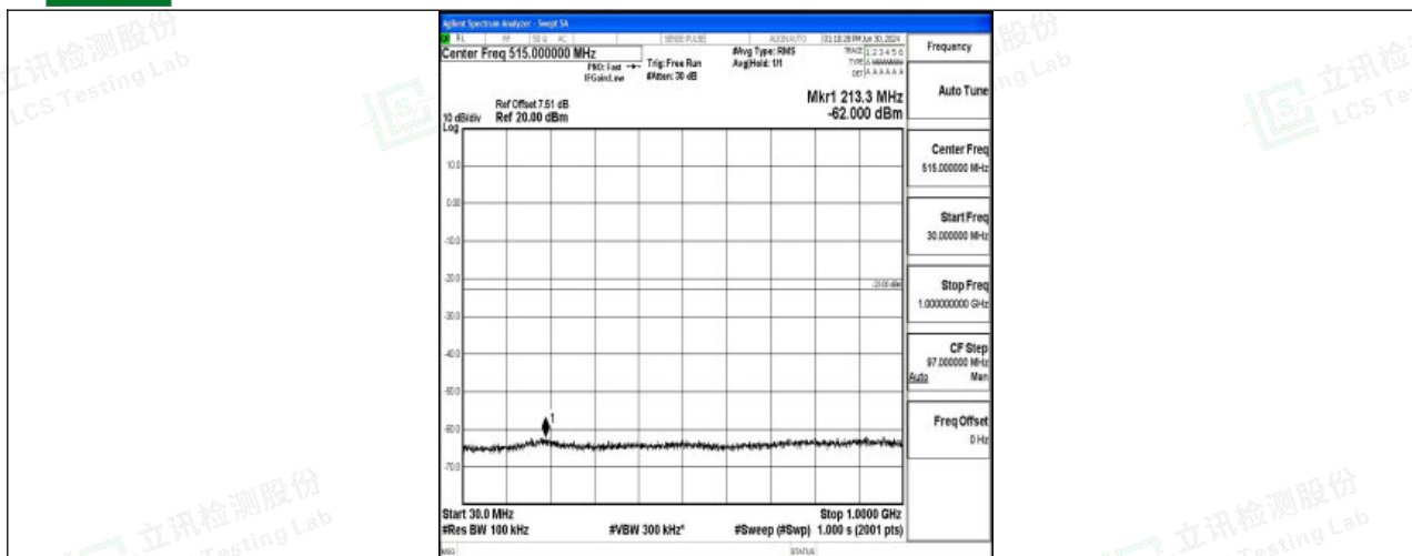
Band4_5MHz_QPSK_20375_1RB#0_30~1000_30~1000
