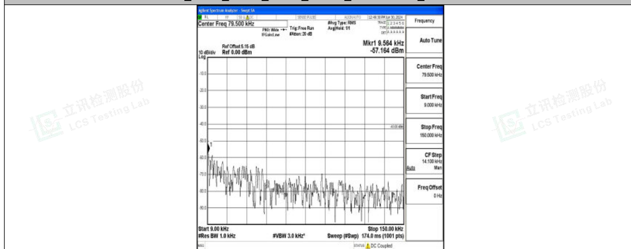
Band4_3MHz_16QAM_20175_1RB#0_0.009~0.15_0.009~0.15
