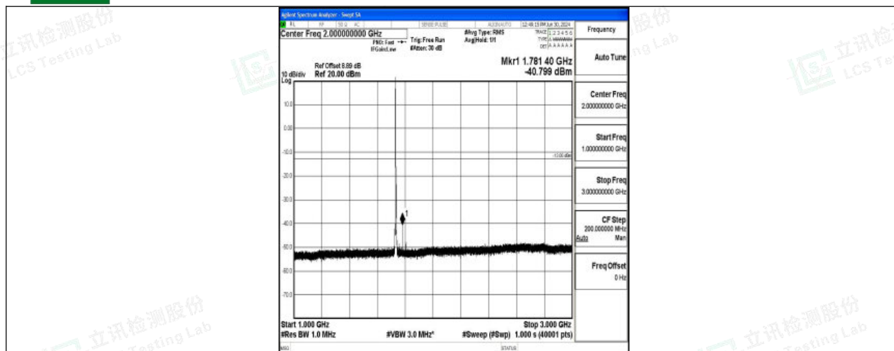
Band4_3MHz_QPSK_20175_1RB#0_1000~3000_1000~3000
