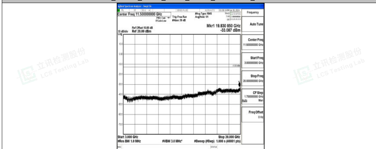
Band4_10MHz_QPSK_20350_1RB#0_3000~20000_3000~20000
