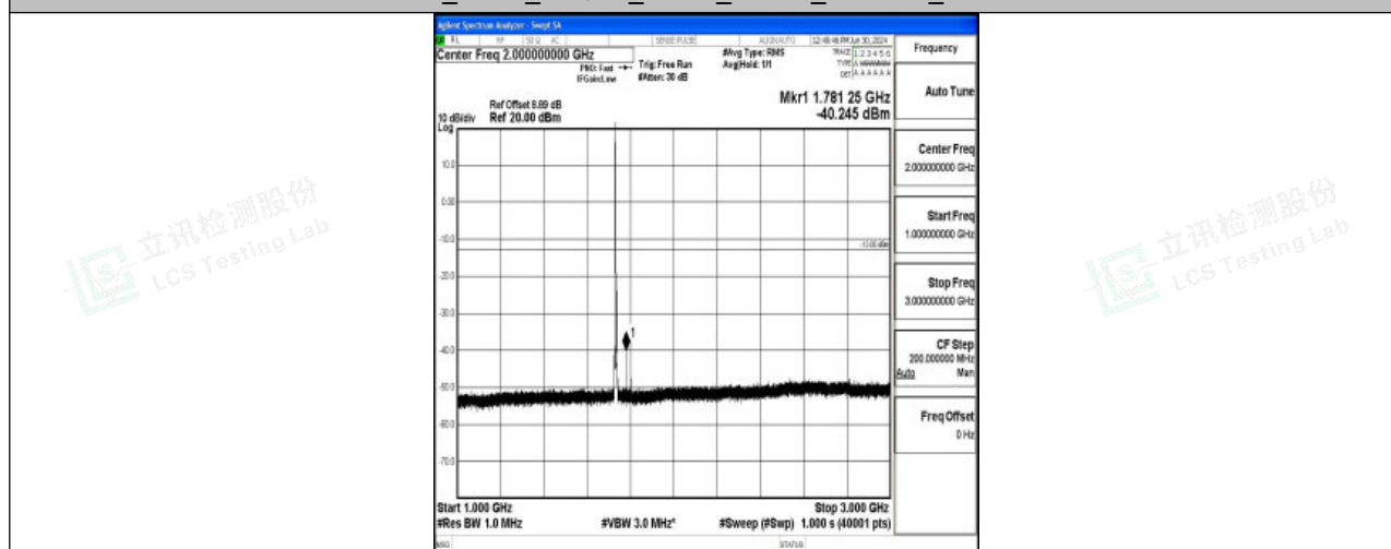
Band4_3MHz_16QAM_20175_1RB#0_1000~3000_1000~3000
