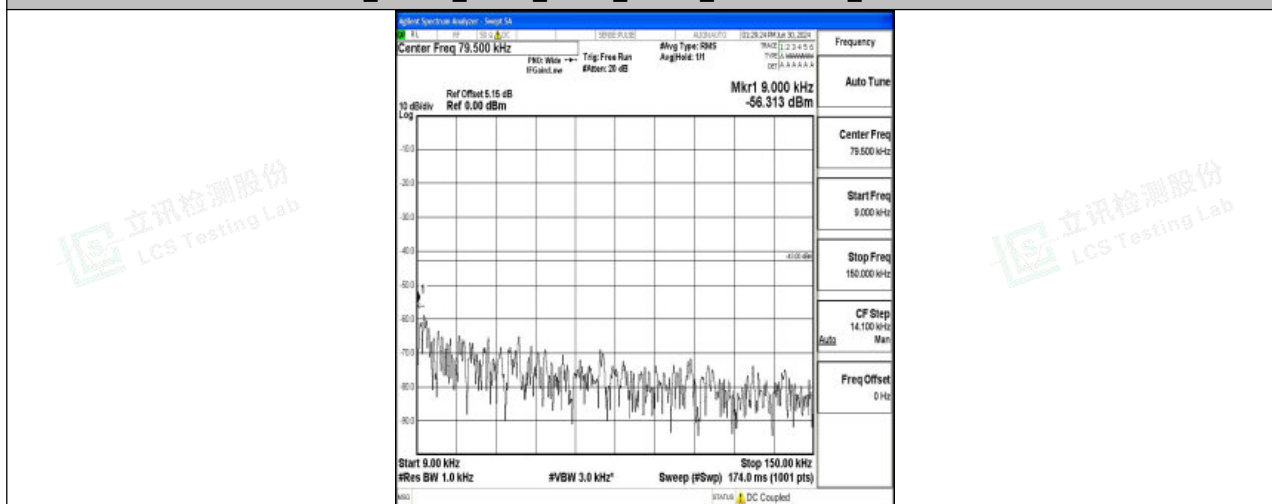
Band4_10MHz_16QAM_20175_1RB#0_0.009~0.15_0.009~0.15
