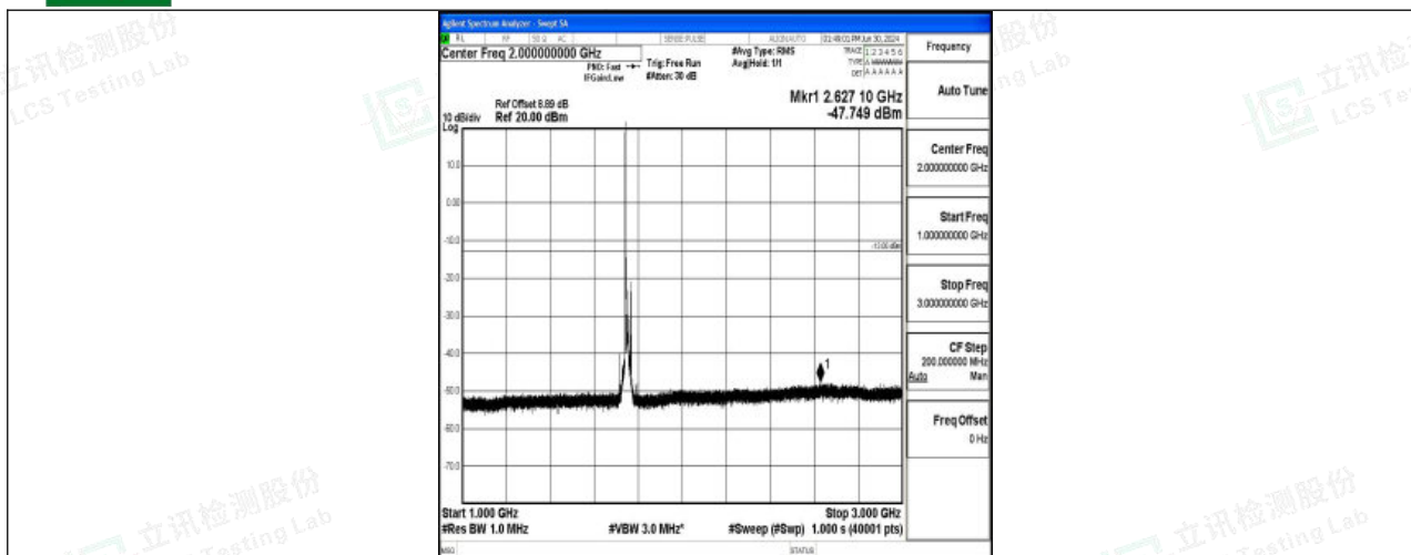
Band4_15MHz_16QAM_20325_1RB#0_1000~3000_1000~3000
