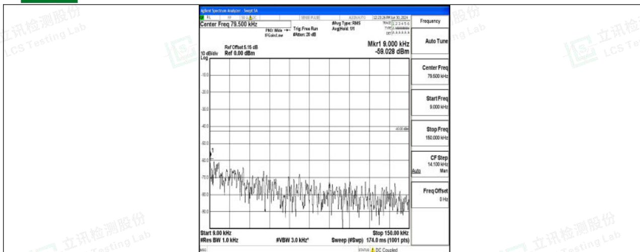
Band4_1.4MHz_16QAM_20393_1RB#0_0.009~0.15_0.009~0.15
