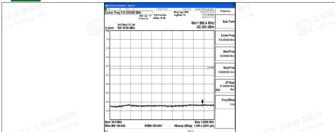
Band4_3MHz_16QAM_19965_1RB#0_30~1000_30~1000
