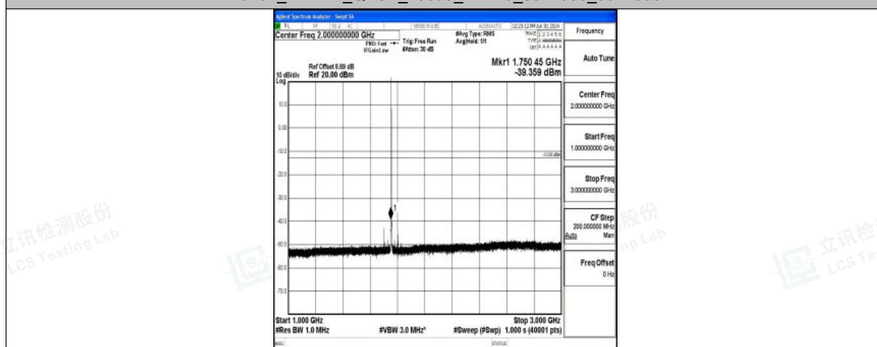
Band4_1.4MHz_QPSK_20393_1RB#0_1000~3000_1000~3000
