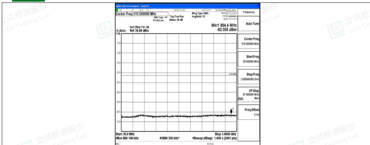
Band4_10MHz_16QAM_20000_1RB#0_30~1000_30~1000
