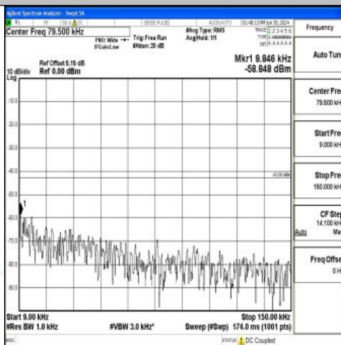
Band4_15MHz_QPSK_20325_1RB#0_0.009~0.15_0.009~0.15
