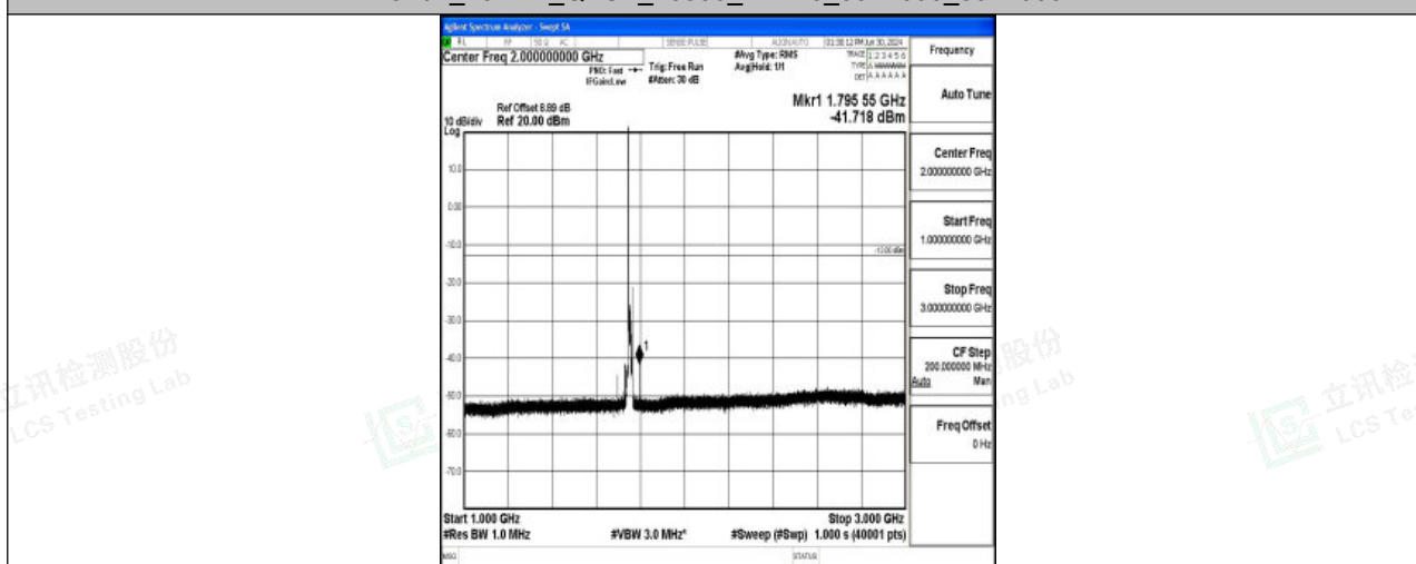
Band4_10MHz_QPSK_20350_1RB#0_1000~3000_1000~3000
