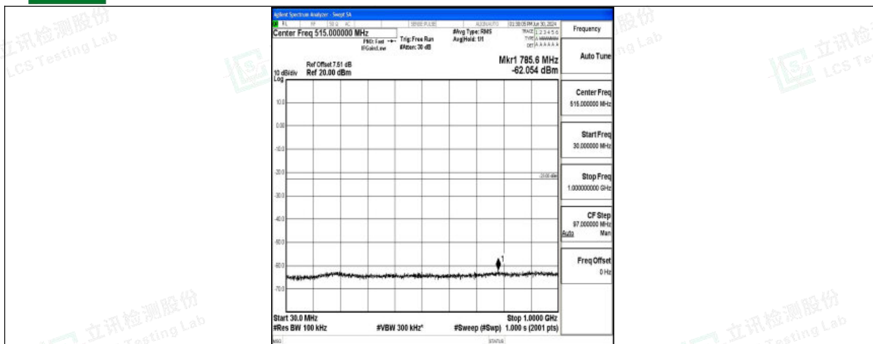
Band4_10MHz_QPSK_20350_1RB#0_30~1000_30~1000
