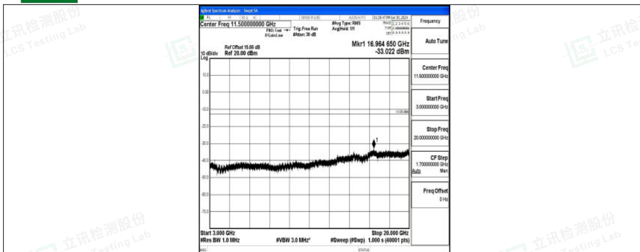
Band4_10MHz_16QAM_20175_1RB#0_3000~20000_3000~20000
