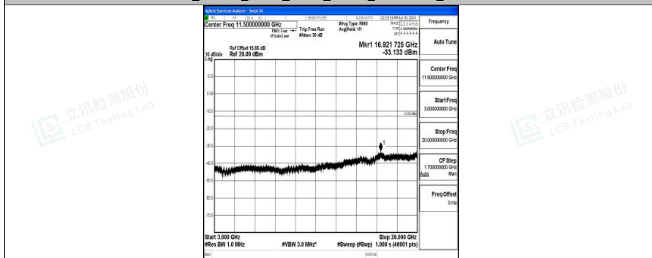
Band4_1.4MHz_QPSK_20393_1RB#0_3000~20000_3000~20000
