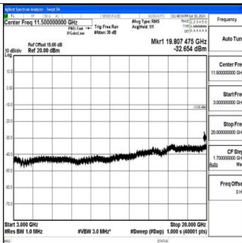
Band4_15MHz_16QAM_20175_1RB#0_3000~20000_3000~20000
