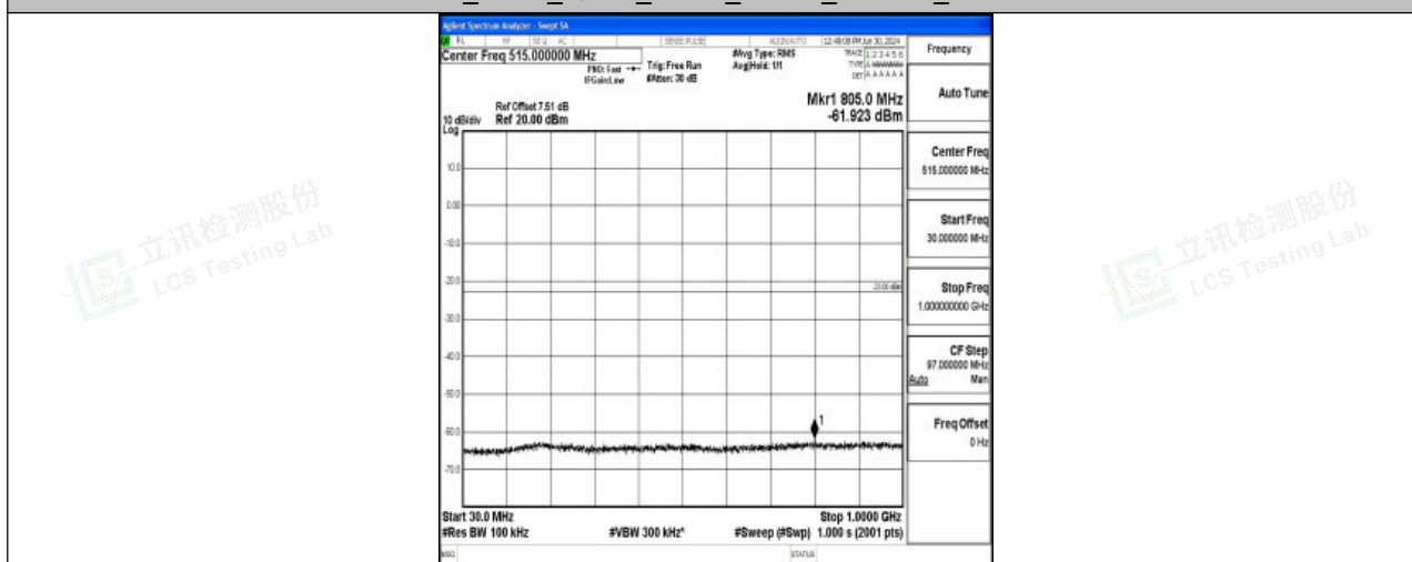
Band4_3MHz_QPSK_20175_1RB#0_30~1000_30~1000
