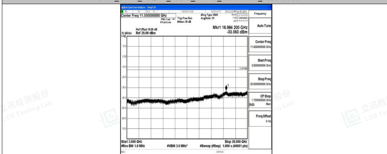
Band4_5MHz_16QAM_20375_1RB#0_3000~20000_3000~20000
