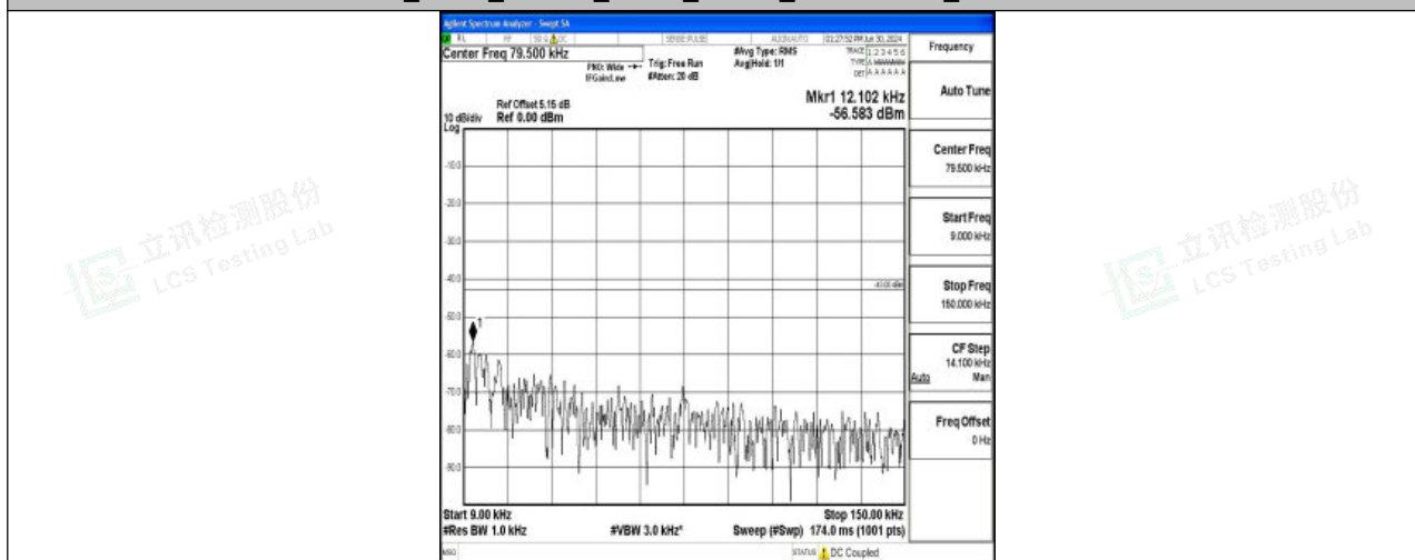
Band4_10MHz_QPSK_20000_1RB#0_0.009~0.15_0.009~0.15
