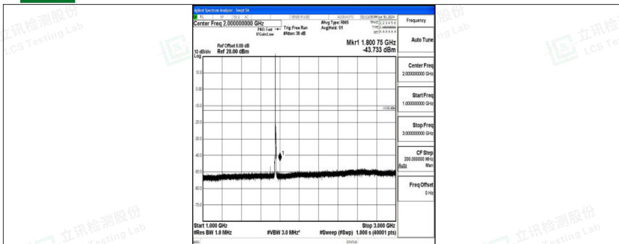
Band4_5MHz_16QAM_20375_1RB#0_1000~3000_1000~3000
