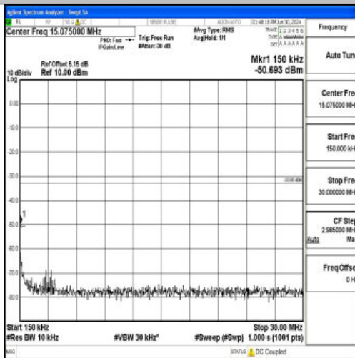
Band4_15MHz_QPSK_20325_1RB#0_0.15~30_0.15~30
