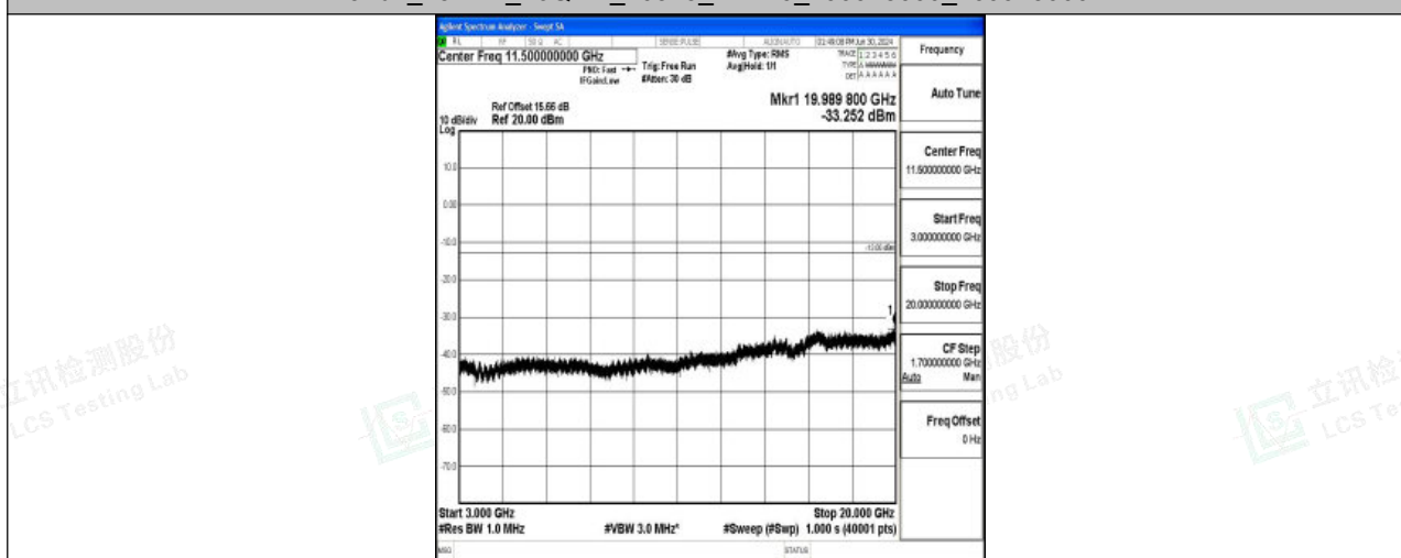
Band4_15MHz_16QAM_20325_1RB#0_3000~20000_3000~20000
