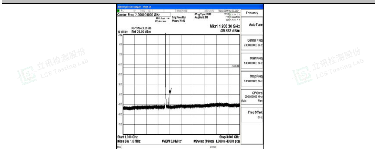
Band4_5MHz_16QAM_20175_1RB#0_1000~3000_1000~3000
