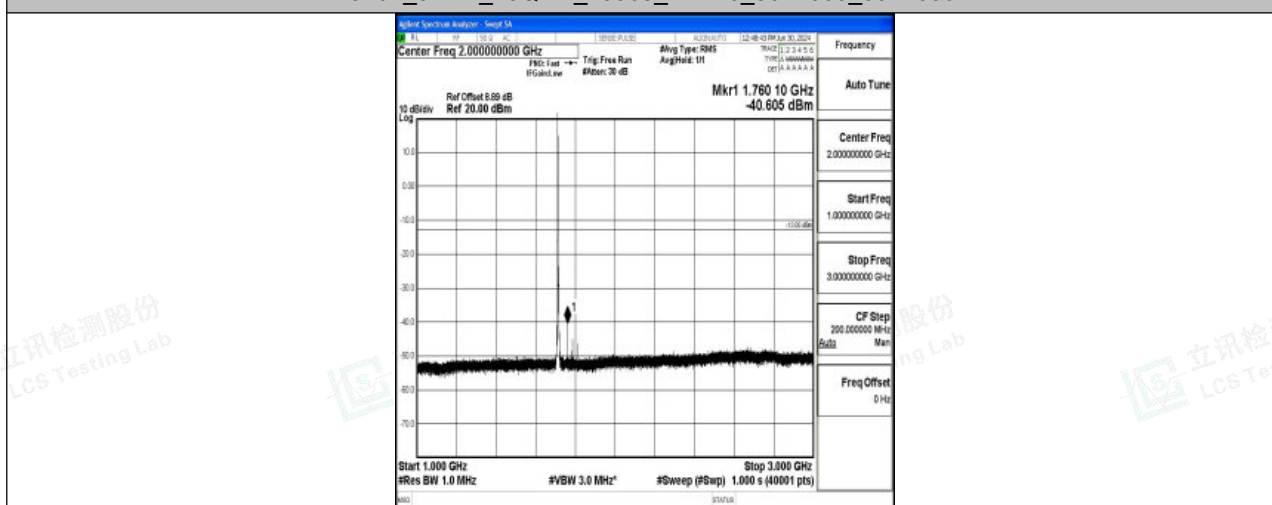
Band4_3MHz_16QAM_19965_1RB#0_1000~3000_1000~3000
