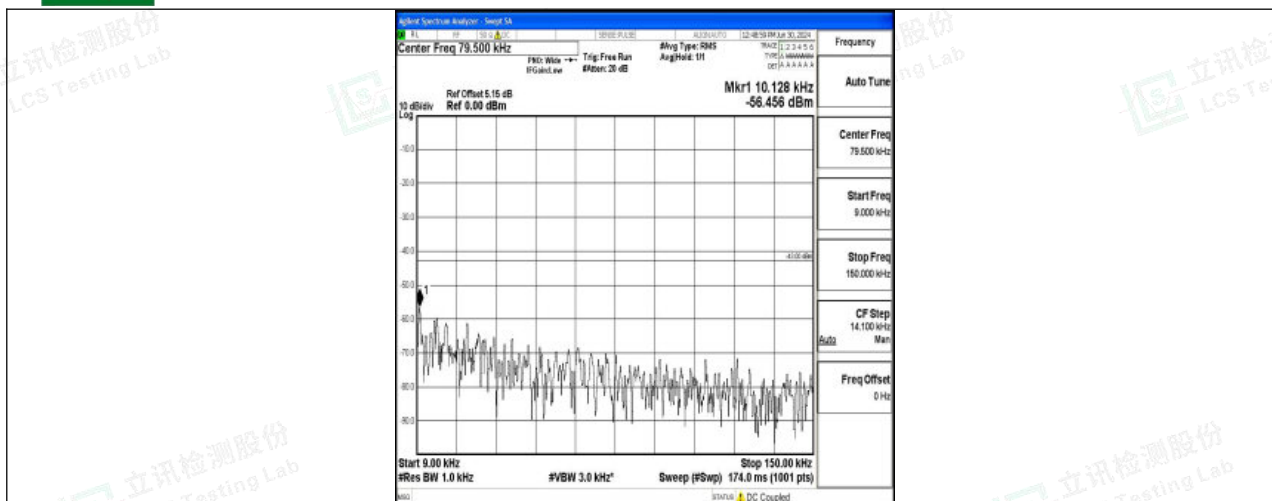
Band4_3MHz_QPSK_20175_1RB#0_0.009~0.15_0.009~0.15
