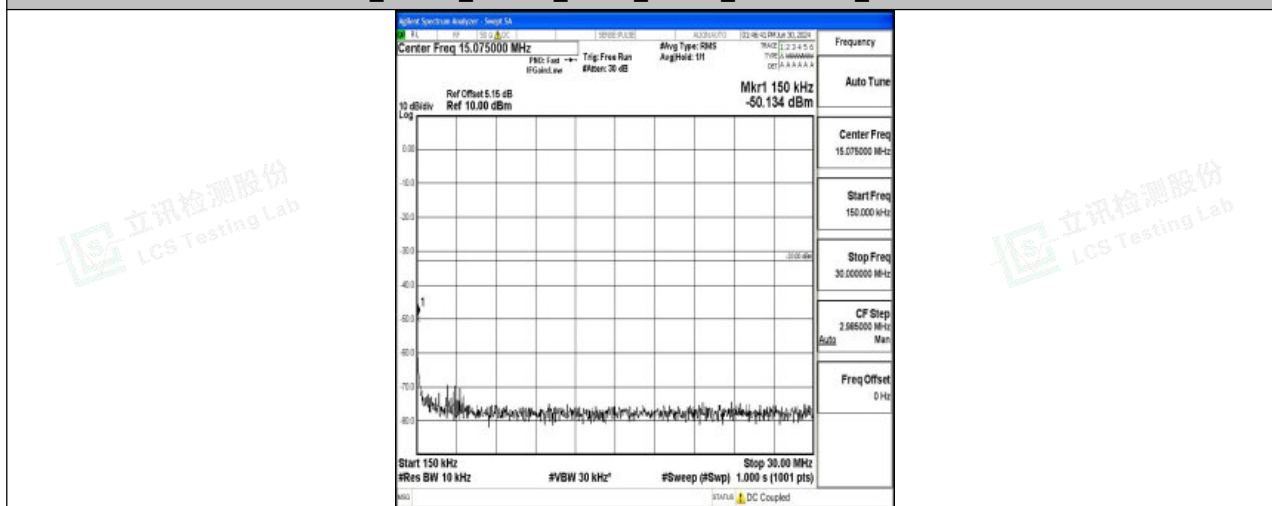
Band4_15MHz_16QAM_20025_1RB#0_0.15~30_0.15~30
