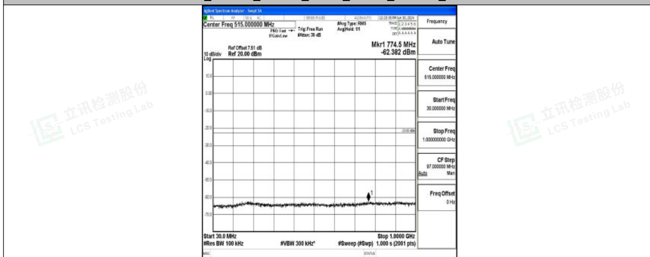
Band4_1.4MHz_16QAM_20393_1RB#0_30~1000_30~1000
