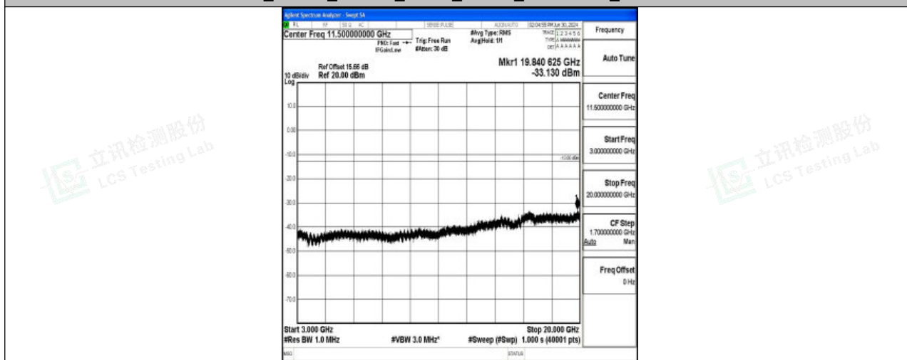
Band4_20MHz_16QAM_20050_1RB#0_3000~20000_3000~20000
