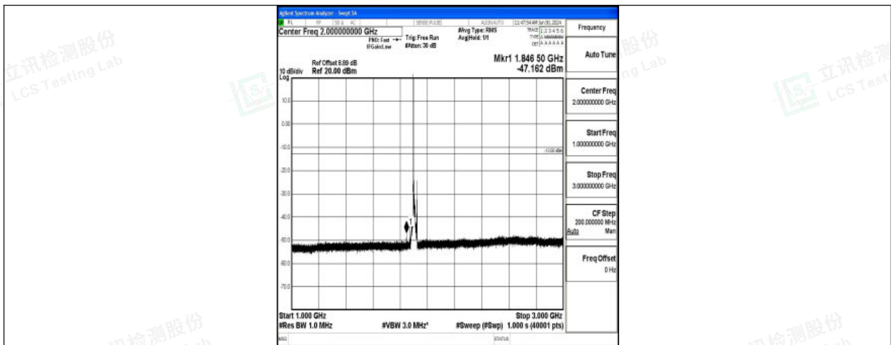
Band2_15MHz_QPSK_19125_1RB#0_1000~3000_1000~3000
