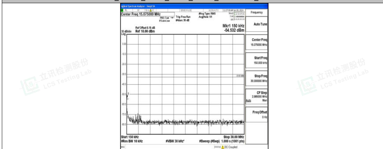
Band2_10MHz_QPSK_18650_1RB#0_0.15~30_0.15~30
