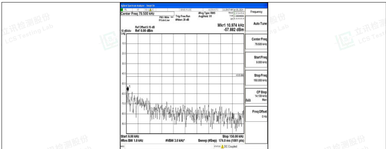
Band2_10MHz_QPSK_19150_1RB#0_0.009~0.15_0.009~0.15
