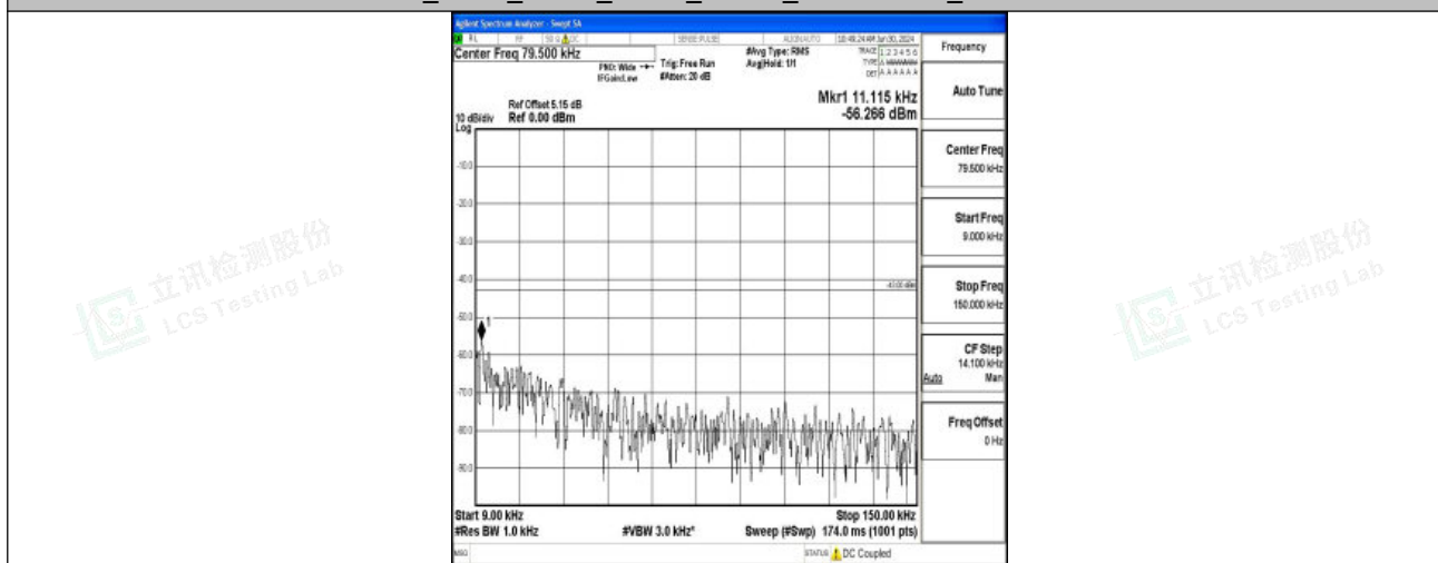
Band2_3MHz_16QAM_19185_1RB#0_0.009~0.15_0.009~0.15
