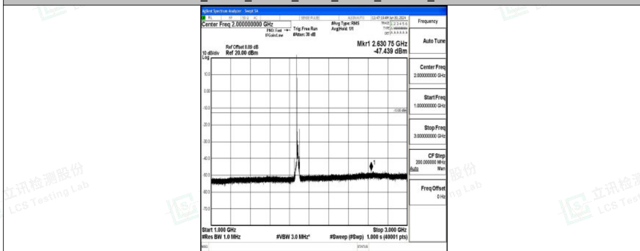
Band2_15MHz_16QAM_18900_1RB#0_1000~3000_1000~3000
