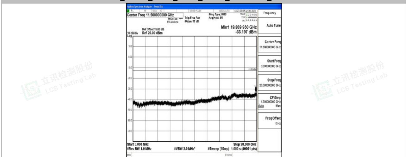
Band2_10MHz_QPSK_18650_1RB#0_3000~20000_3000~20000
