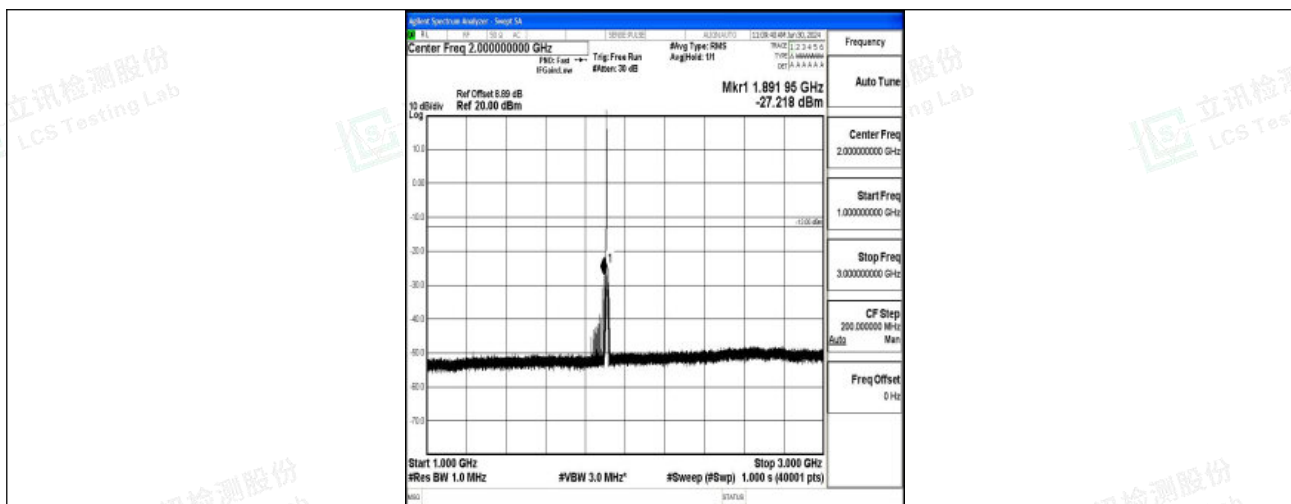
Band2_5MHz_QPSK_19175_1RB#0_1000~3000_1000~3000
