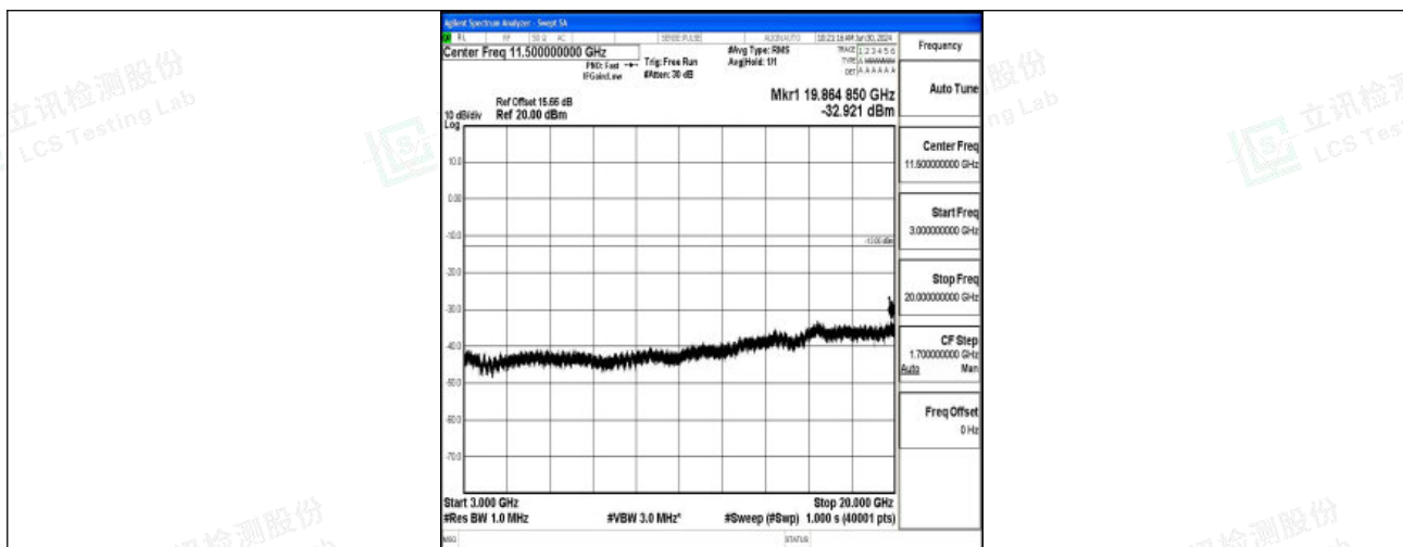
Band2_1.4MHz_16QAM_19193_1RB#0_3000~20000_3000~20000
