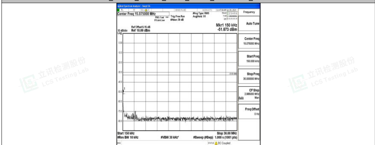
Band2_15MHz_16QAM_18900_1RB#0_0.15~30_0.15~30
