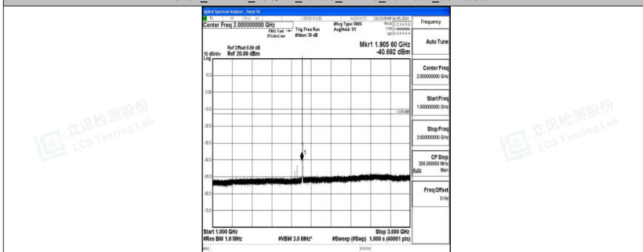
Band2_1.4MHz_16QAM_19193_1RB#0_1000~3000_1000~3000
