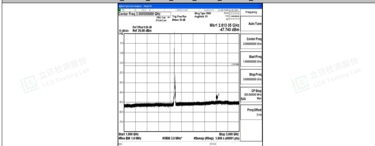
Band2_10MHz_QPSK_18900_1RB#0_1000~3000_1000~3000
