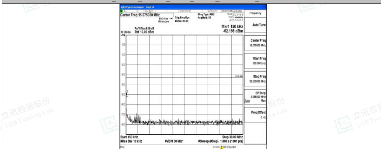
Band2_20MHz_16QAM_18700_1RB#0_0.15~30_0.15~30
