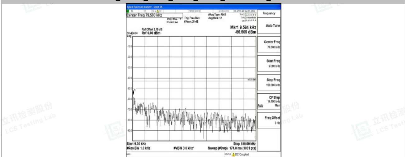
Band2_15MHz_16QAM_18900_1RB#0_0.009~0.15_0.009~0.15
