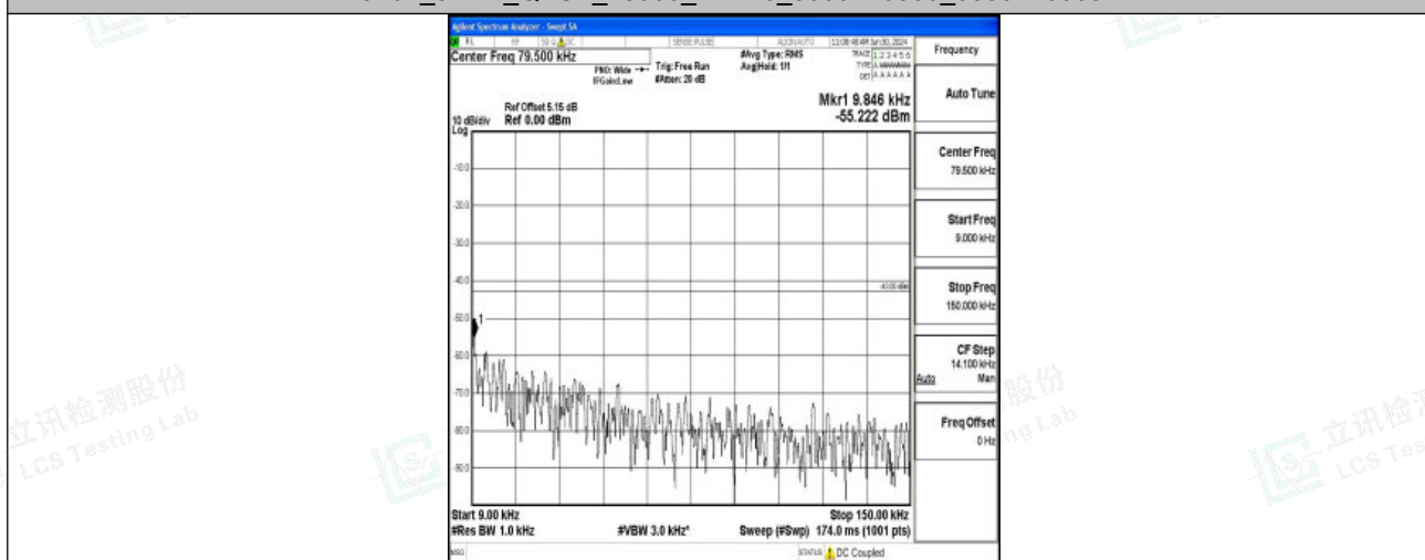
Band2_5MHz_16QAM_18900_1RB#0_0.009~0.15_0.009~0.15
