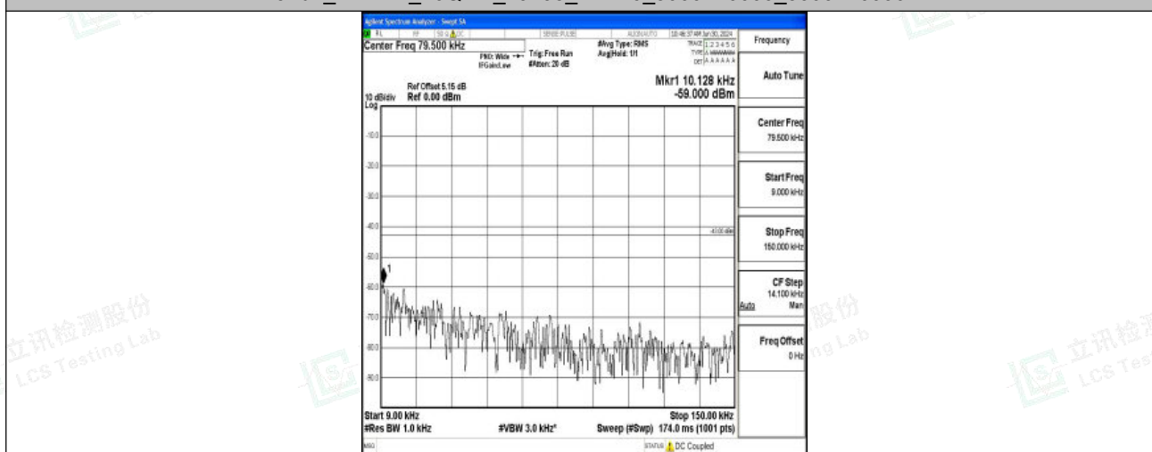
Band2_3MHz_QPSK_18615_1RB#0_0.009~0.15_0.009~0.15
