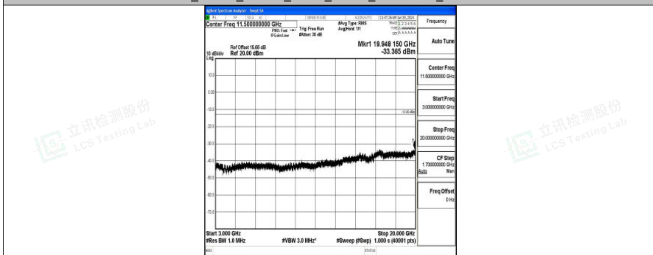
Band2_15MHz_16QAM_18900_1RB#0_3000~20000_3000~20000
