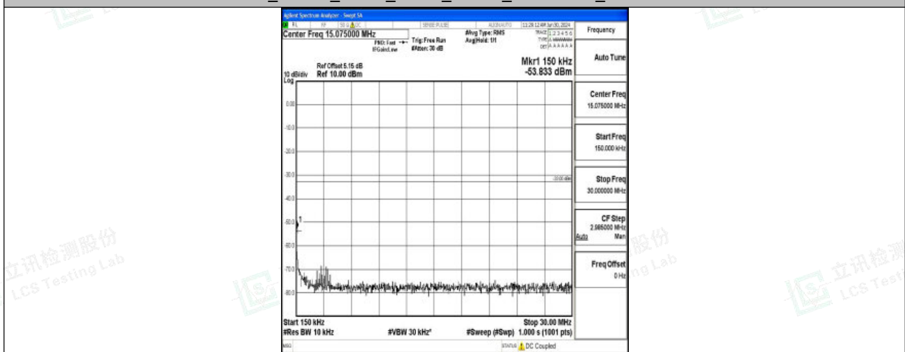
Band2_10MHz_QPSK_19150_1RB#0_0.15~30_0.15~30
