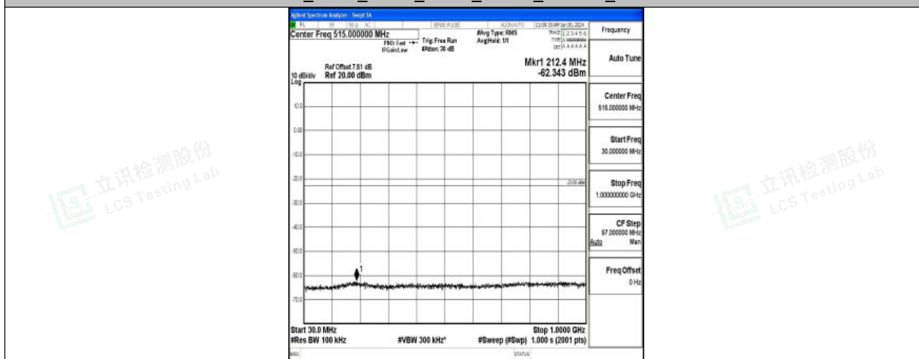
Band2_5MHz_QPSK_19175_1RB#0_30~1000_30~1000
