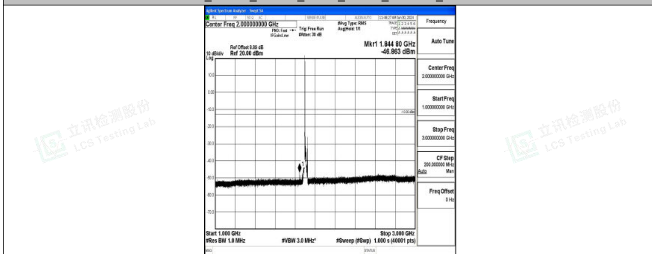
Band2_15MHz_16QAM_19125_1RB#0_1000~3000_1000~3000
