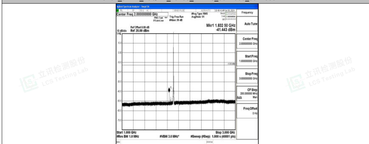
Band2_3MHz_16QAM_19185_1RB#0_1000~3000_1000~3000
