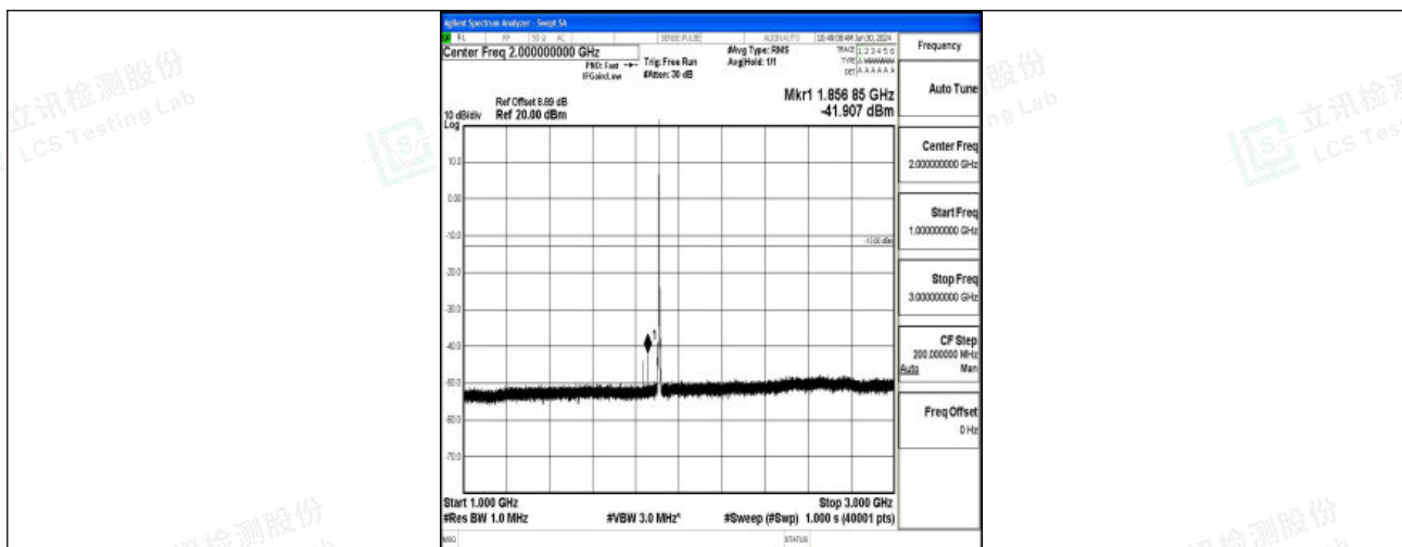
Band2_3MHz_QPSK_19185_1RB#0_1000~3000_1000~3000
