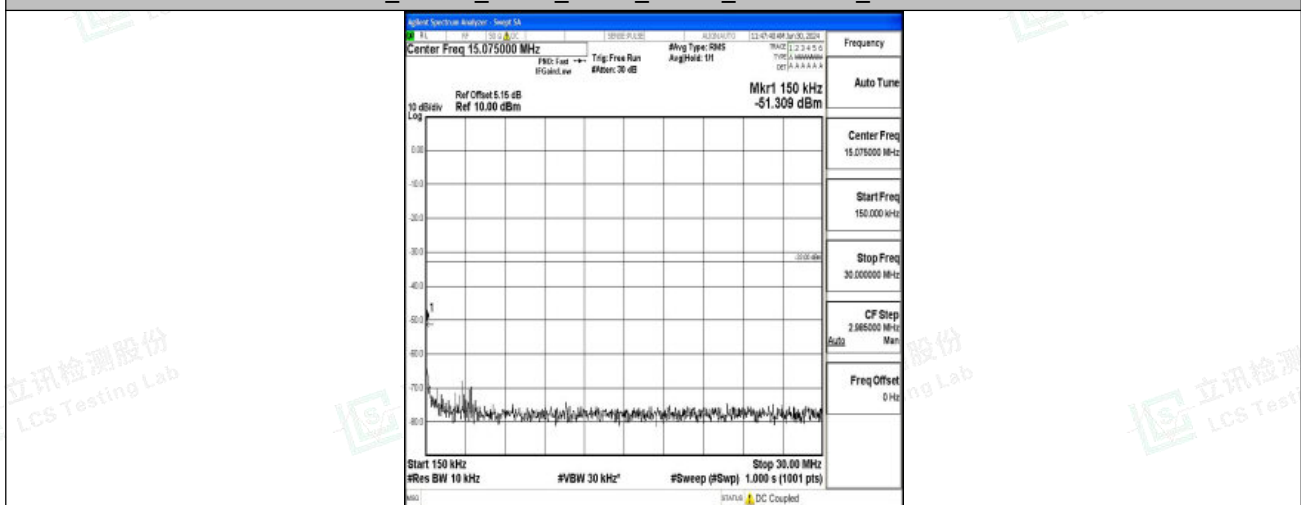
Band2_15MHz_QPSK_19125_1RB#0_0.15~30_0.15~30
