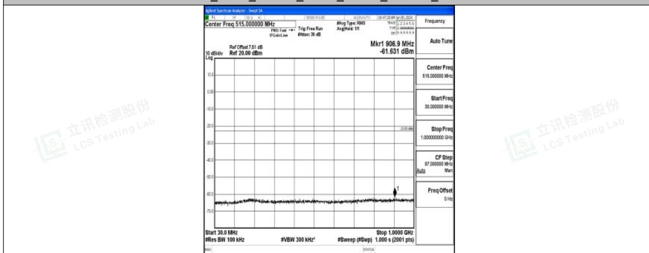
Band2_3MHz_16QAM_18615_1RB#0_30~1000_30~1000
