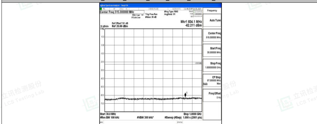
Band2_15MHz_16QAM_19125_1RB#0_30~1000_30~1000
