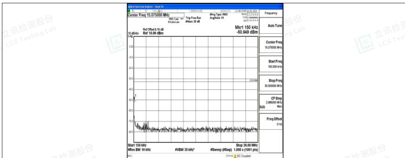
Band2_15MHz_16QAM_19125_1RB#0_0.15~30_0.15~30
