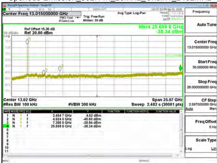
Spurious Emission_802.11n_20MHz_Chain1_2462MHz
