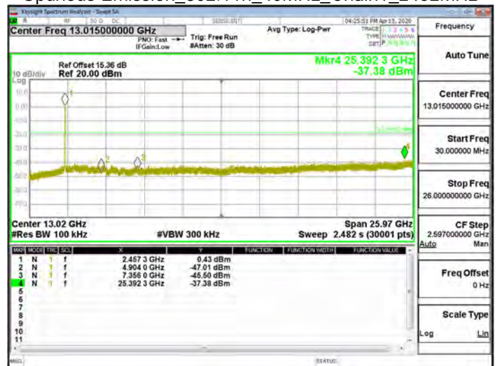
Spurious Emission_802.11n_40MHz_Chain1_2452MHz
