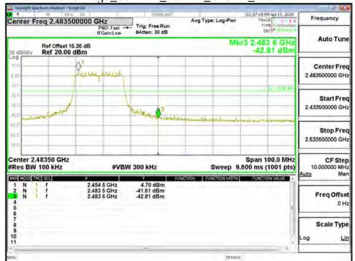
Band Edge_802.11n_20MHz_Chain1_2462MHz
