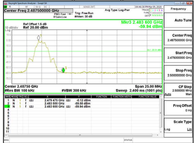
2Mband Edge_BLE_2M_HighCH39-2480
