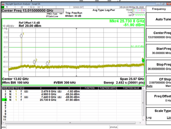
1M\Spurious Emission_BLE_1M_HighCH39-2480
