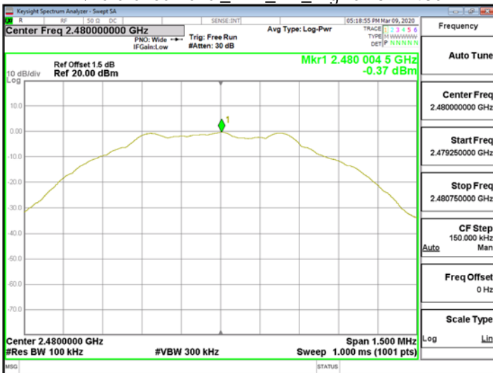
1MReference Level_BLE_1M_HighCH39-2480
