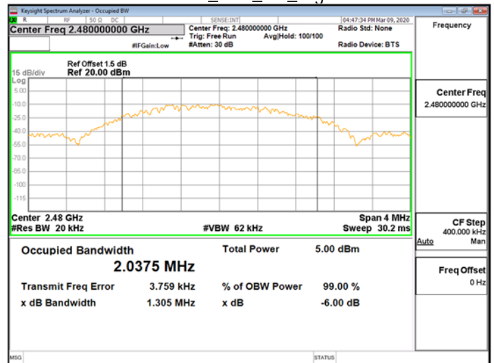
2MNIC OBW 99%_BLE_2M_HighCH39-2480
