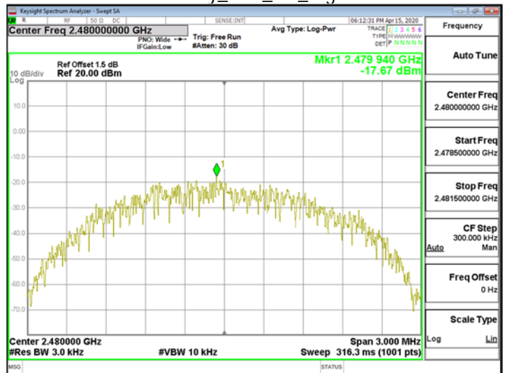
2M Power Density_BLE_2M_HighCH39-2480
