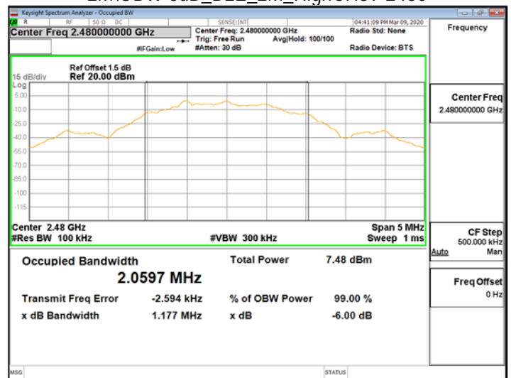
2MOBW 6dB_BLE_2M_HighCH39-2480
