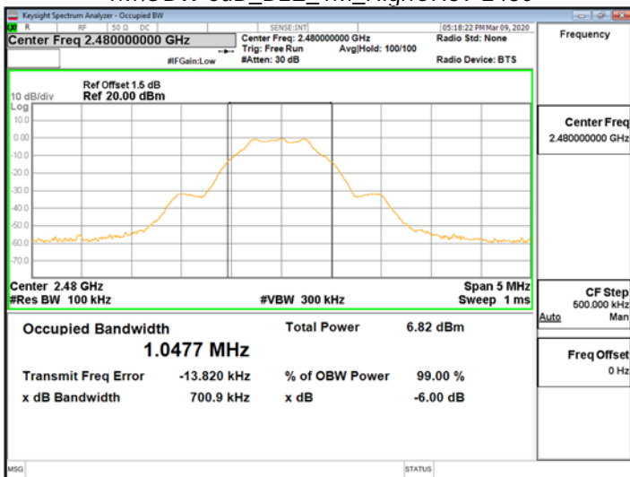
1MOBW 6dB_BLE_1M_HighCH39-2480
