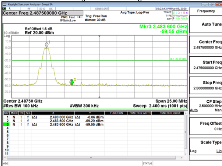
1Mband Edge_BLE_1M_HighCH39-2480
