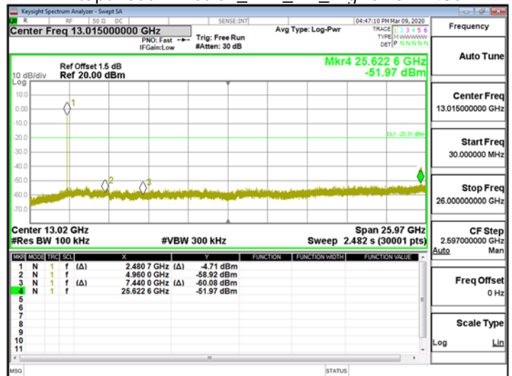
2M\Spurious Emission_BLE_2M_HighCH39-2480
