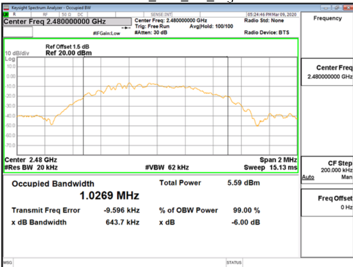
1MNIC OBW 99%_BLE_1M_HighCH39-2480
