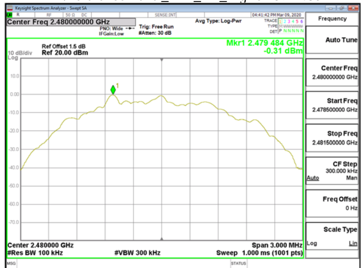
2MReference Level_BLE_2M_HighCH39-2480
