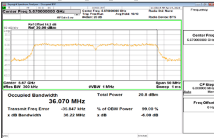
IC_802.11n_40MHz_Chain1_5670MHz
