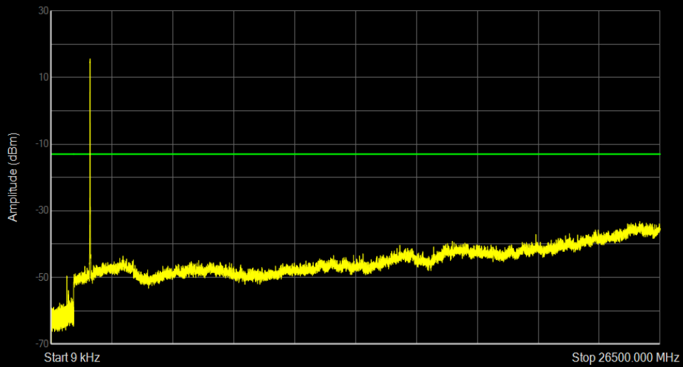
Band66 QPSK BW=10MHz Channel=132022 RB Size=50 Position=#0
