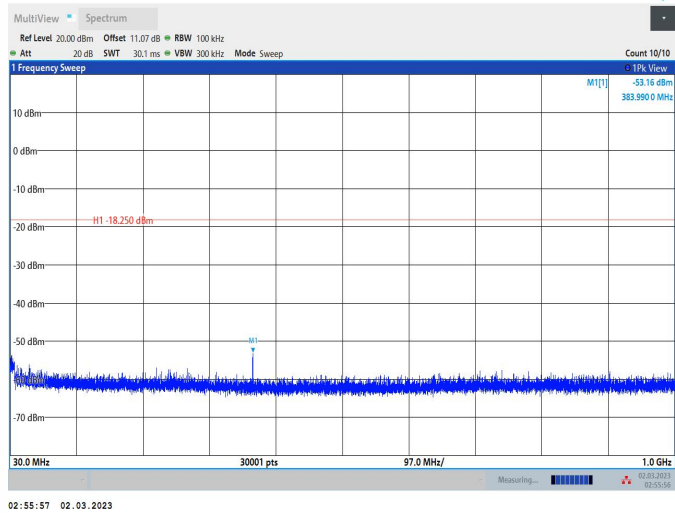
BLE_1M_Ant1_2440_30~1000
