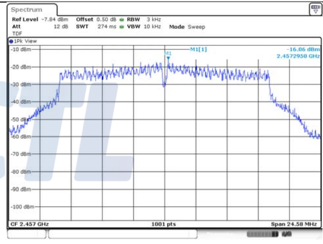
802.11g / 2 457 MHz
