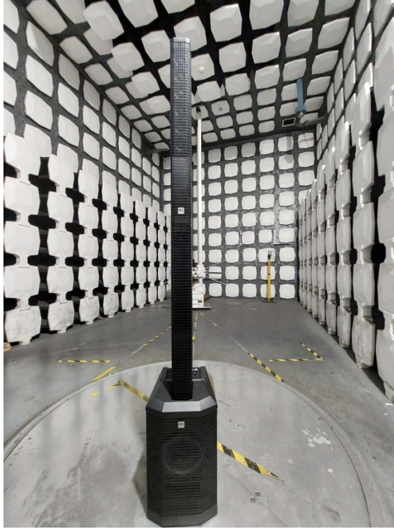
Radiated Emission (Below 1G)
