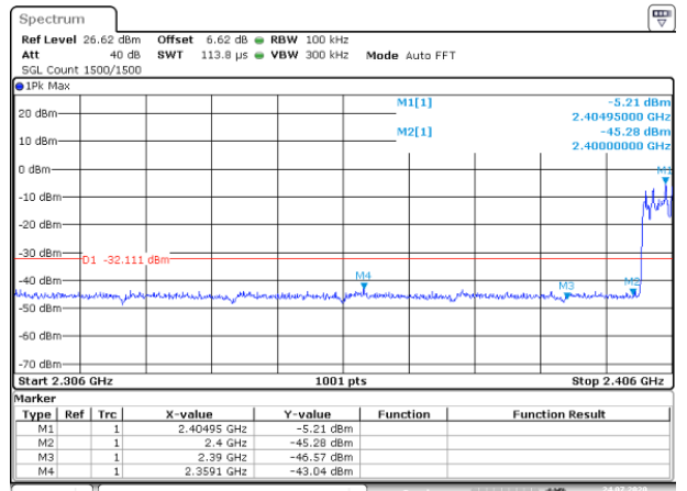
Hopping mode
