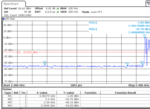
Hopping mode
