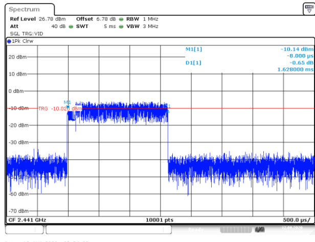
Channel 39 / 2441 MHz - 2DH3
