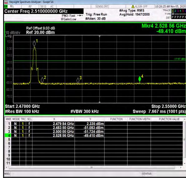
Channel 78 / 2480 MHz – Non-Hopping
