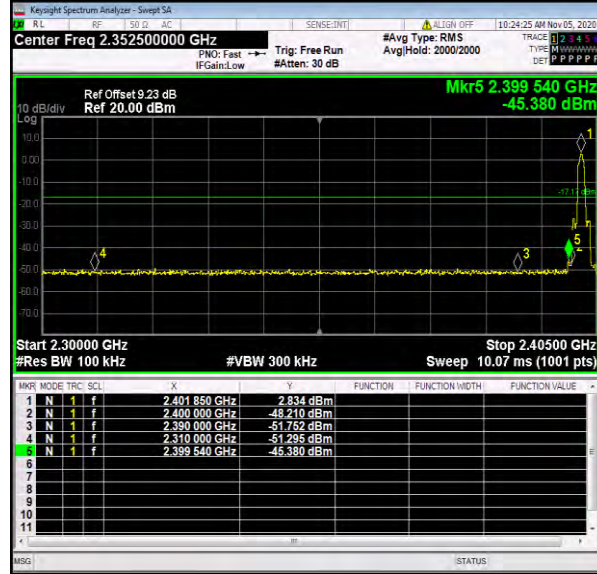
Channel 0 / 2402 MHz – Non-Hopping
