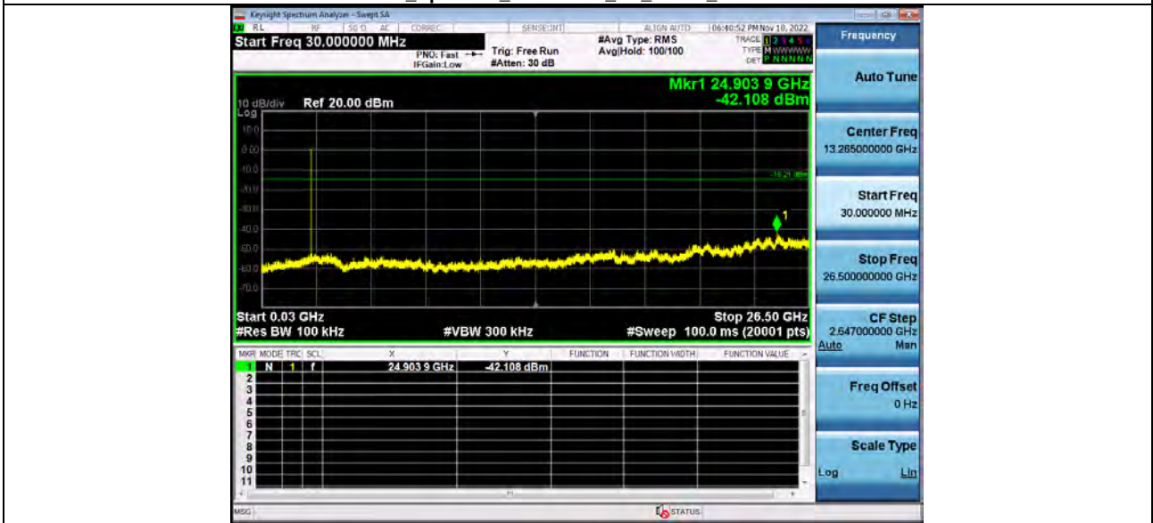
1_Reference_Level_BT_1-DH5_2480
