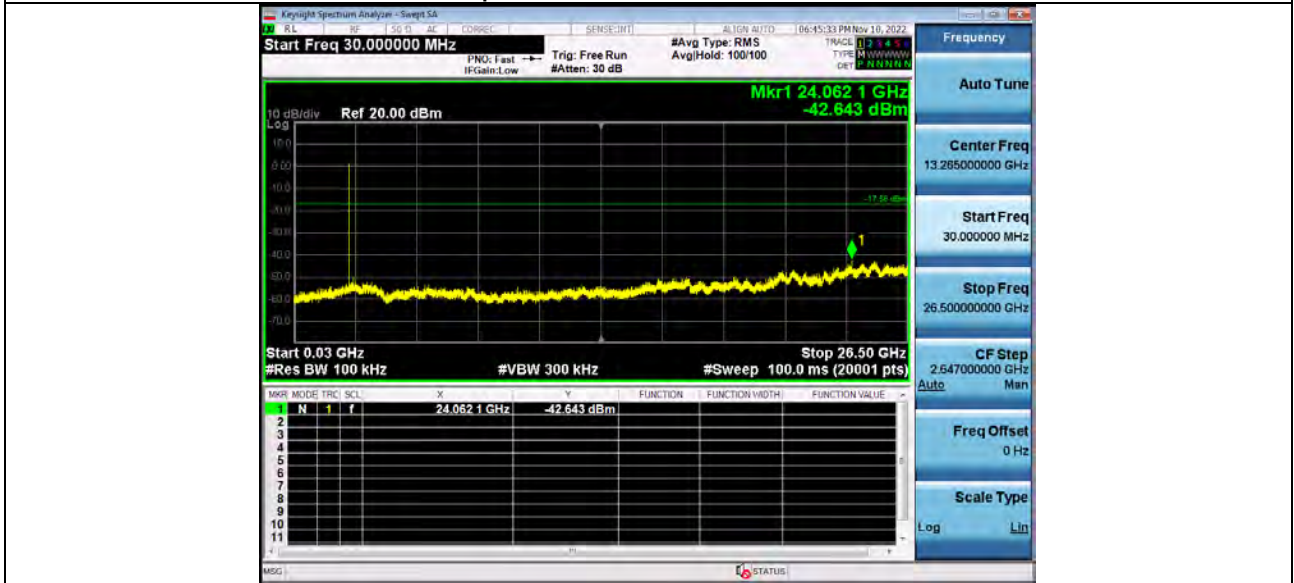
2_Spurious_Emissions_BT_2-DH5_2402
