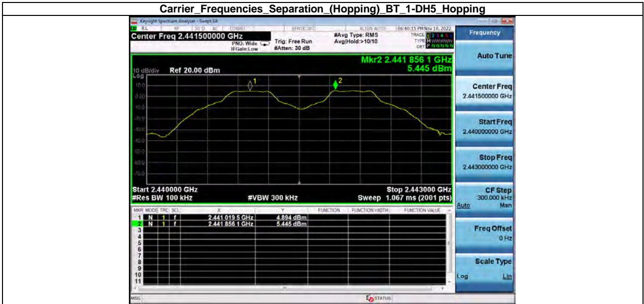
Carrier_Frequencies_Separation_(Hopping)_BT_1-DH5_Hopping
