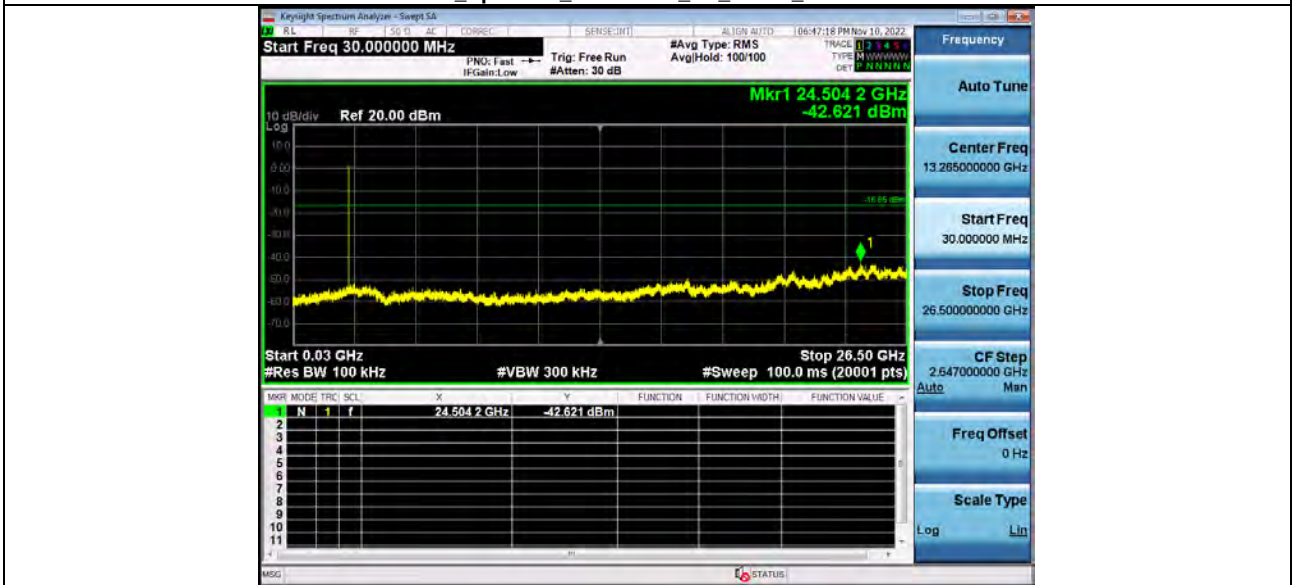
1_Reference_Level_BT_2-DH5_2480
