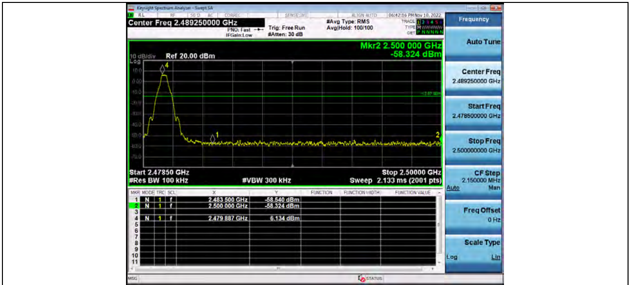
Band_Edge_(Hopping)_BT_1-DH5_Hopping
