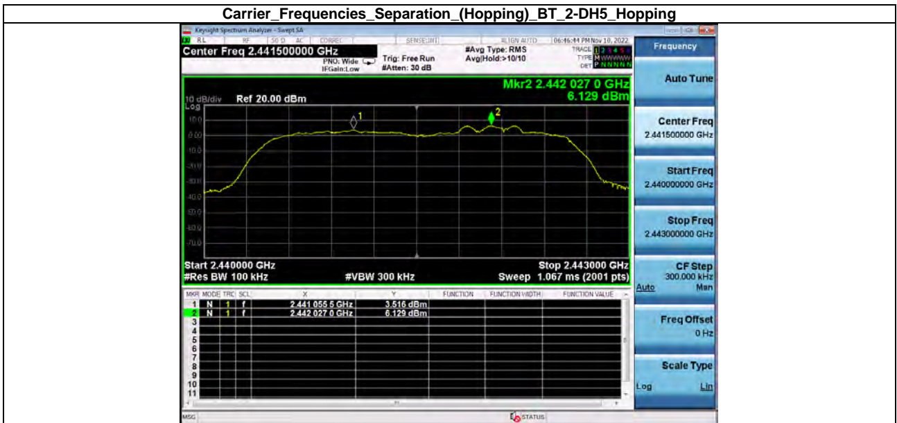
Carrier_Frequencies_Separation_(Hopping)_BT_2-DH5_Hopping
