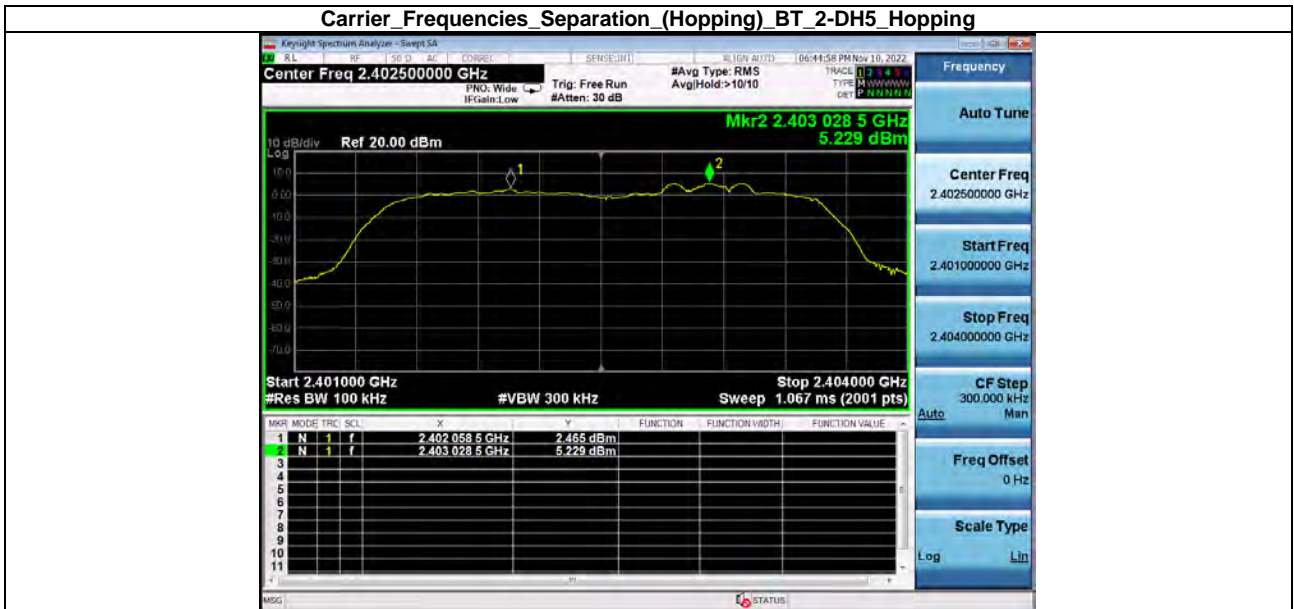
Carrier_Frequencies_Separation_(Hopping)_BT_2-DH5_Hopping
