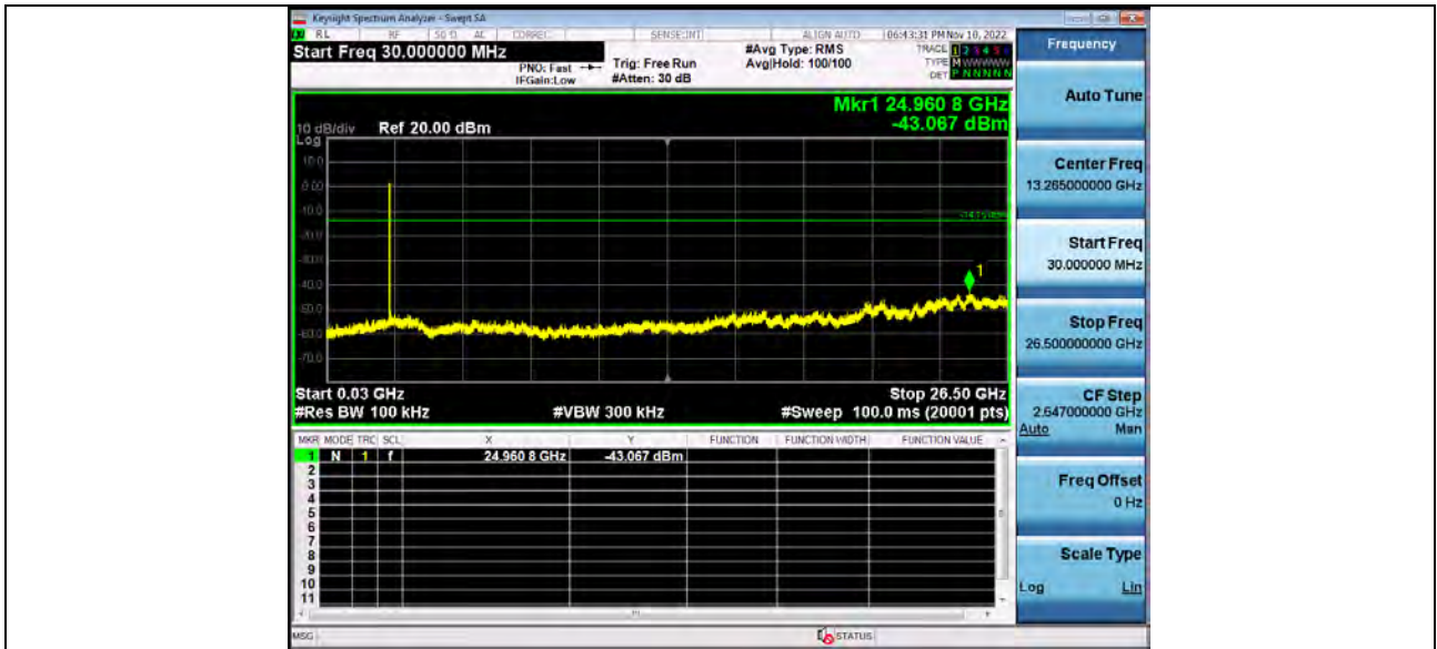
1_Reference_Level_BT_2-DH5_2402
