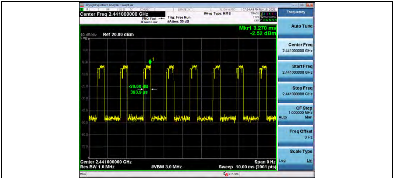
Dwell Time (Hopping) BT 3-DH5_2441_One Burst Time
