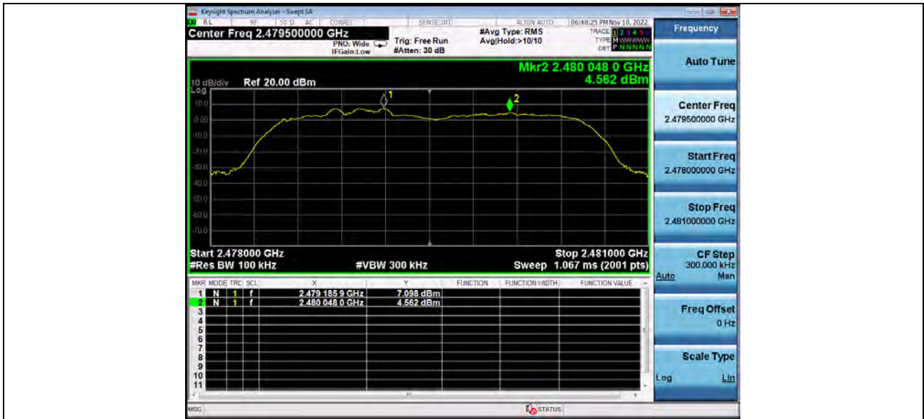
Carrier_Frequencies_Separation_(Hopping)_BT_3-DH5_Hopping
