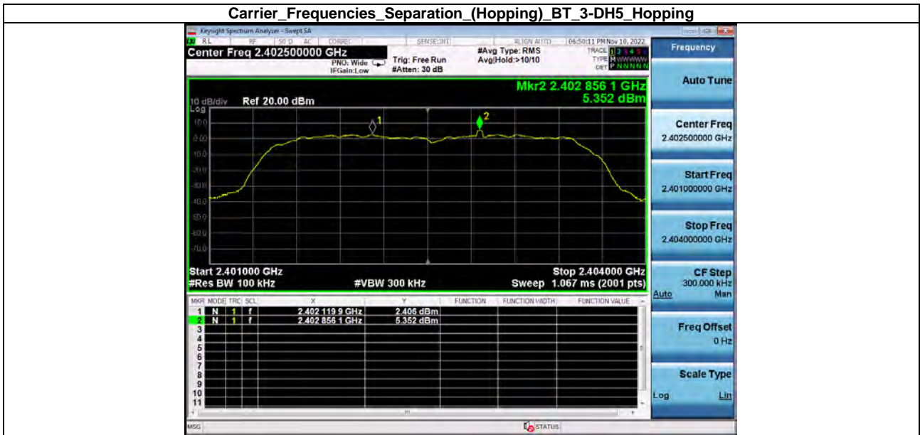
Carrier_Frequencies_Separation_(Hopping)_BT_3-DH5_Hopping
