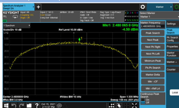
GFSK (BLE 1M) HIGH CHANNEL
