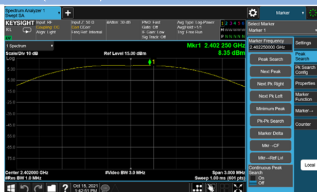
GFSK(BLE 1M ) LOW CHANNEL
