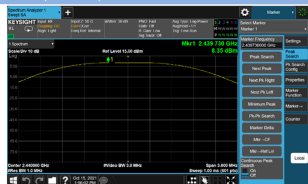
GFSK(BLE 1M ) MIDDLE CHANNEL
