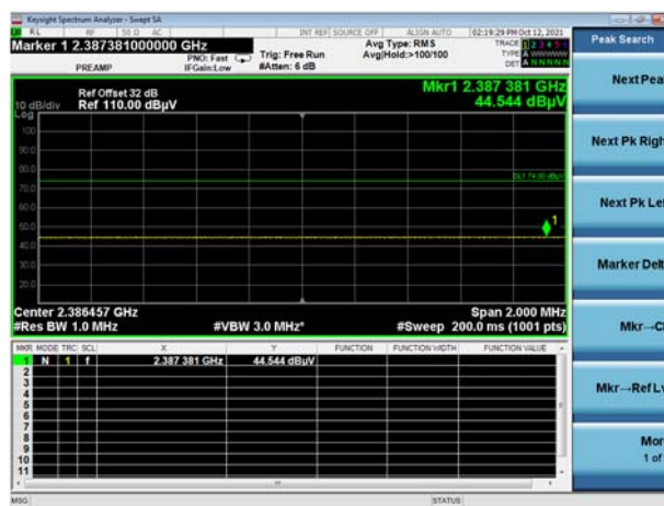
\pi/4 -DQPSK LOW CHANNEL, AVERAGE
