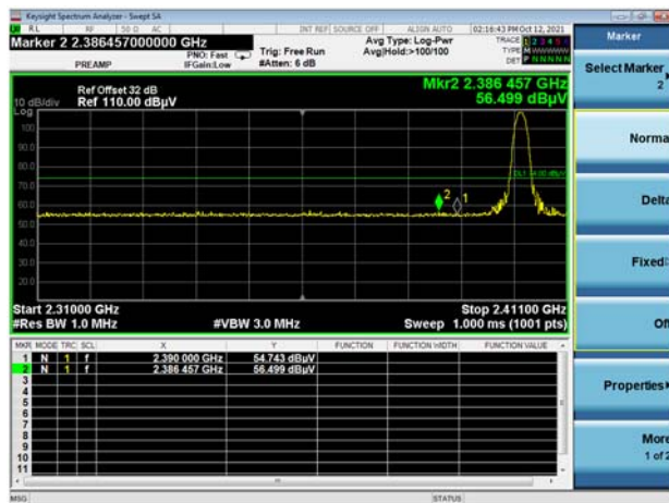
\pi/4 -DQPSK LOW CHANNEL, PEAK
