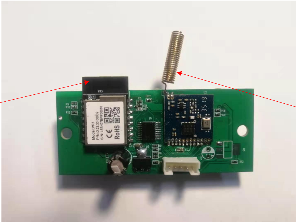
433MHz SRD Antenna
