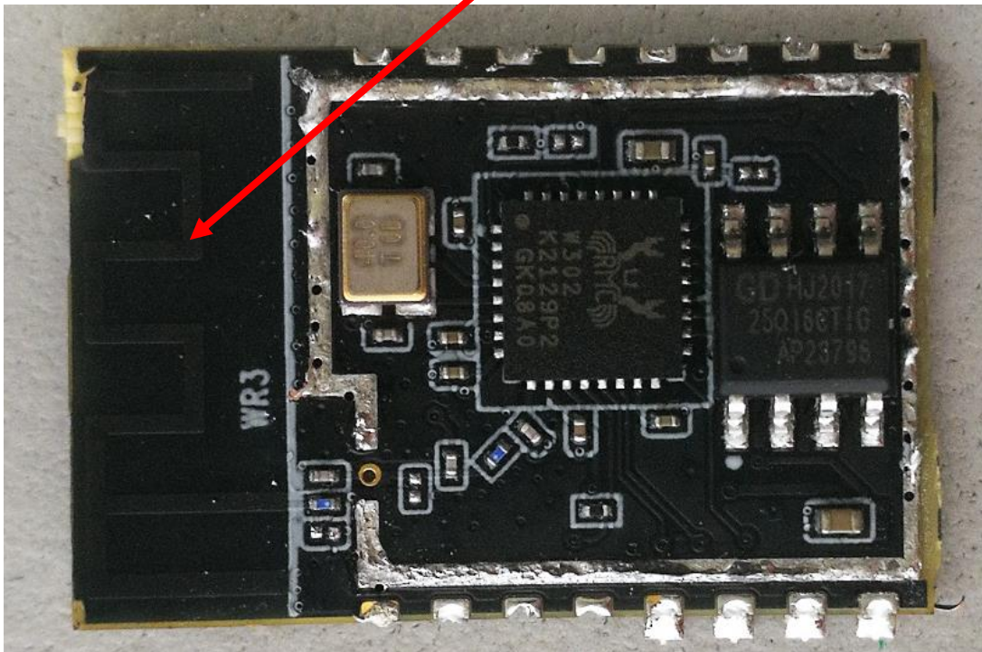
Antenna location
