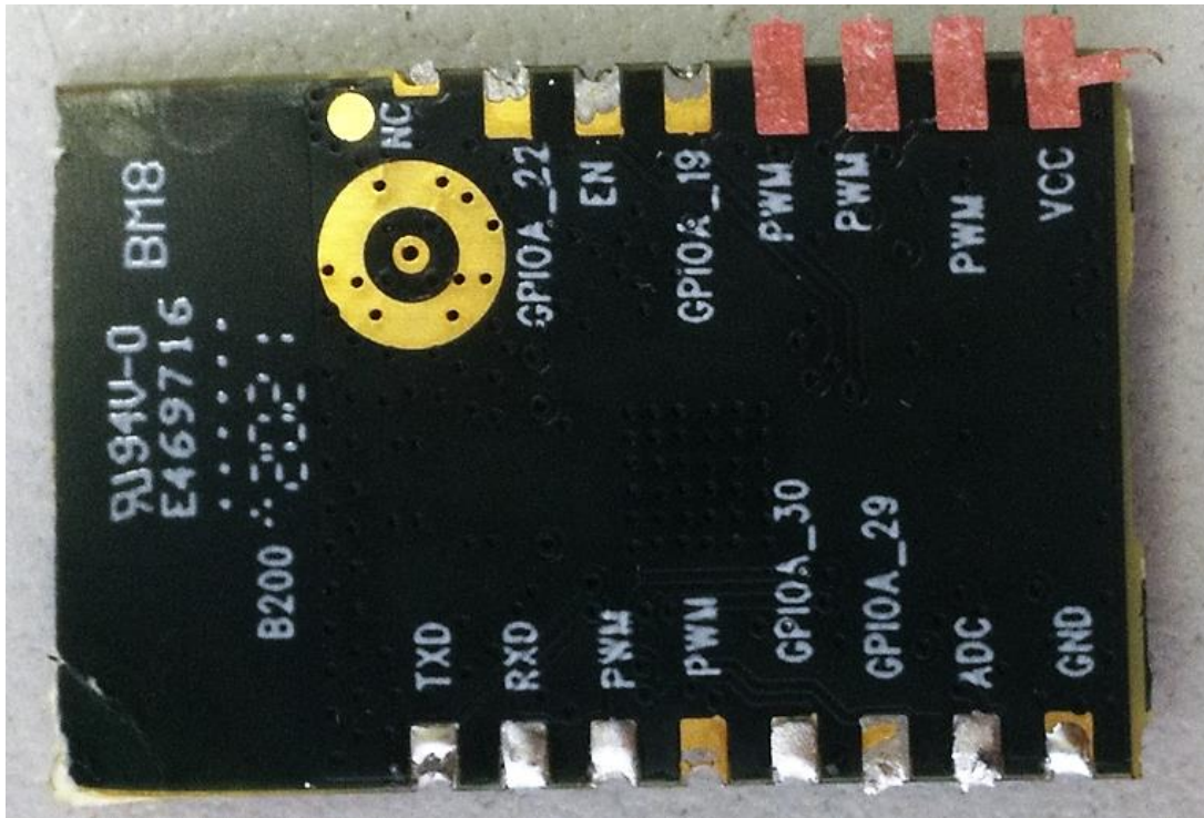
Antenna location
