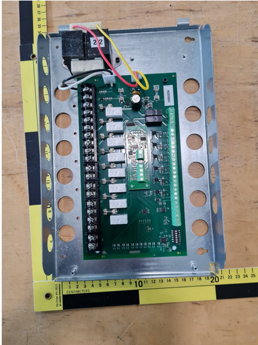
Figure 1 – EUT (SR) Internal Photo
