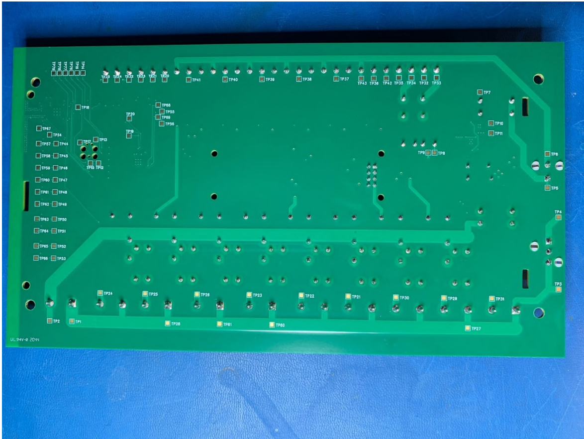
Figure 3 – EUT (SR) Internal Photo PCB Bottom
