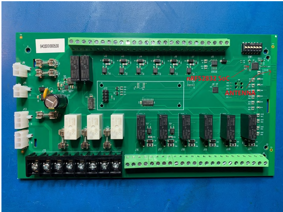
Figure 4 – EUT (ZVC) Internal Photo PCB Top
