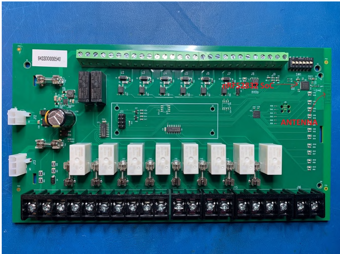
Figure 2 – EUT (SR) Internal Photo PCB Top
