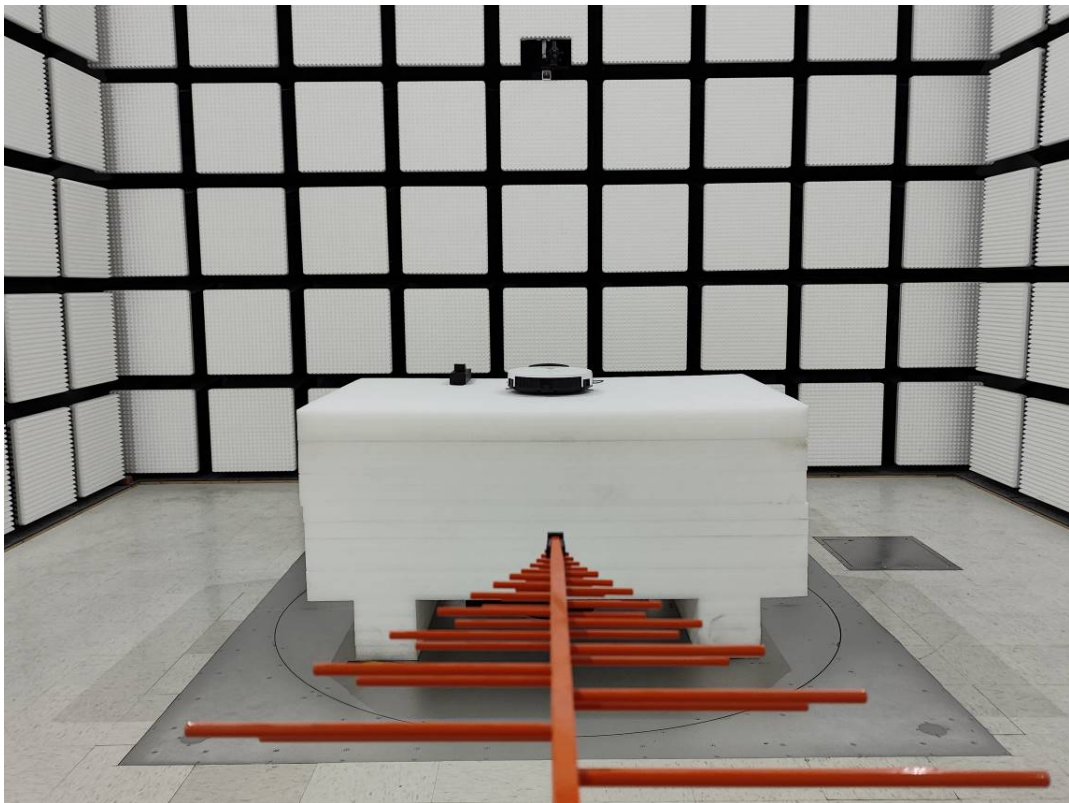
Radiated Emission Below 1GHz View Adapter 2 + Charging Dock
