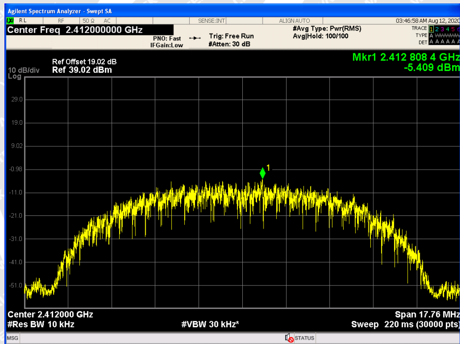
802.11b_Low Channel
