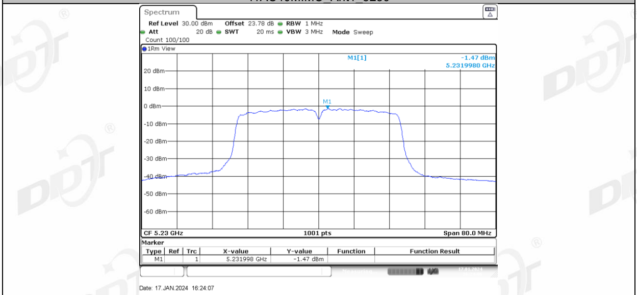
11AC40MIMO Ant2 5230
