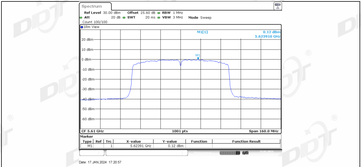
11AC80MIMO Ant2 5610
