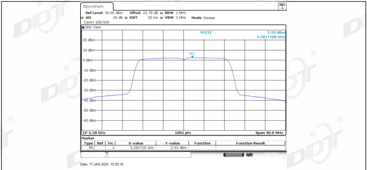
11AC20MIMO Ant2 5280
