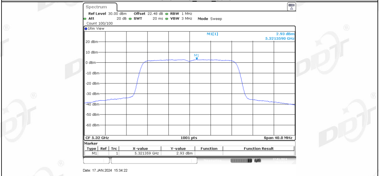
11AC20MIMO Ant2 5320
