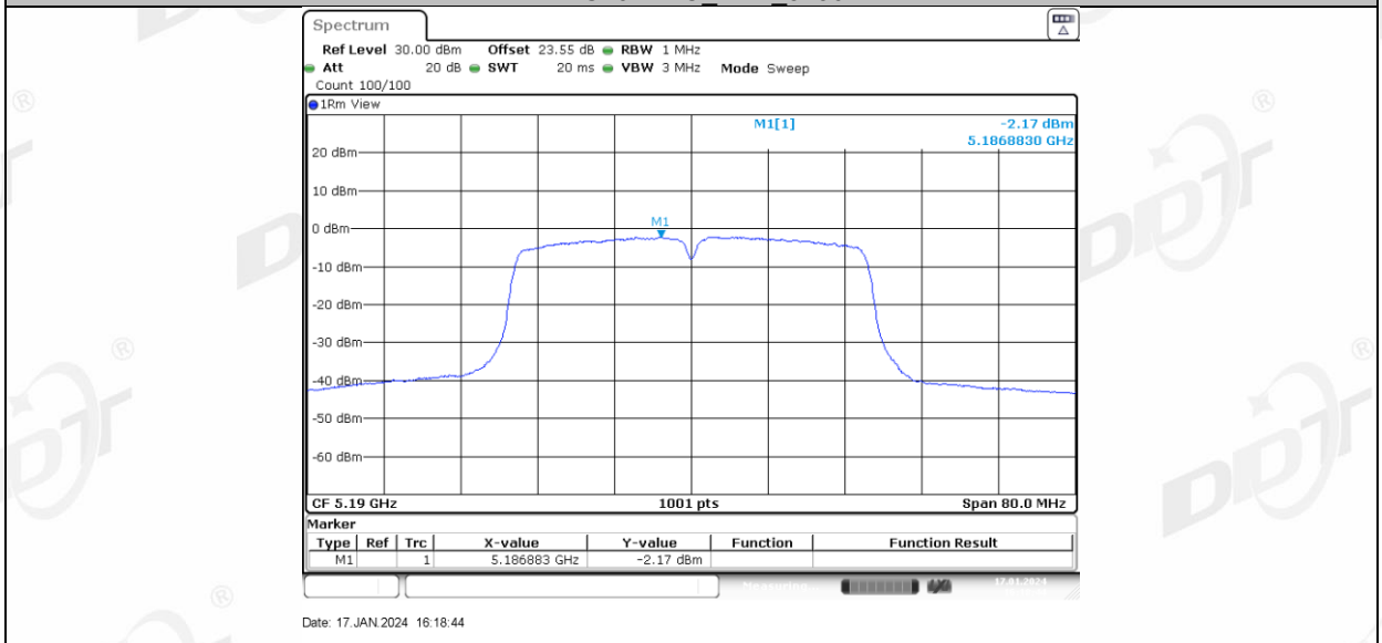
11AC40MIMO Ant2 5190
