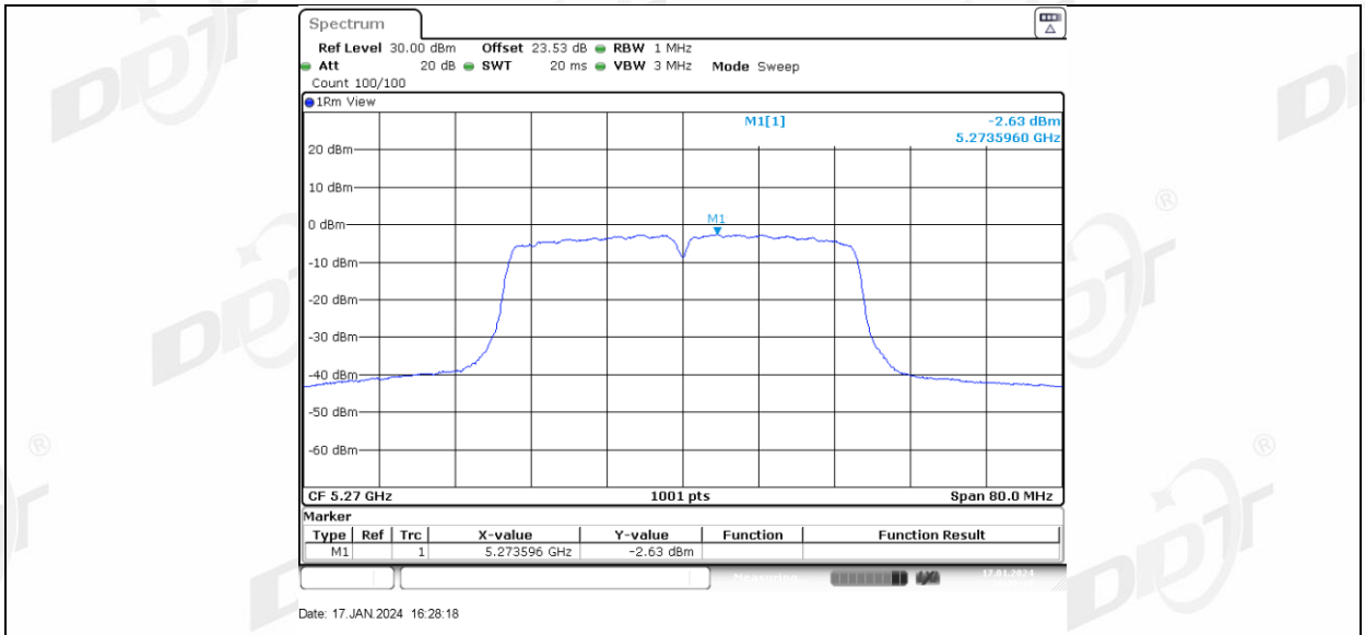
11AC40MIMO Ant2 5270
