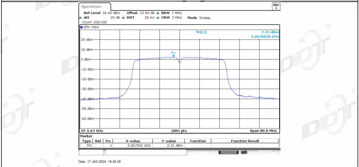
11AC40MIMO Ant2 5670
