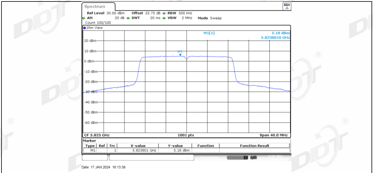
11AC20MIMO Ant2 5825
