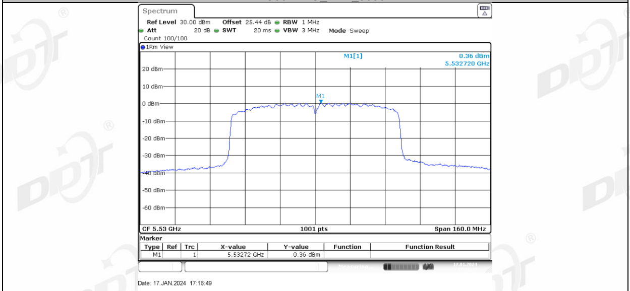
11AC80MIMO Ant2 5530
