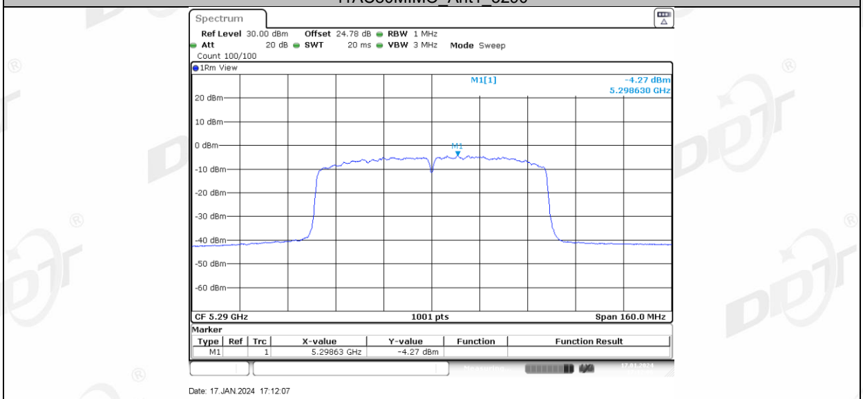
11AC80MIMO Ant2 5290
