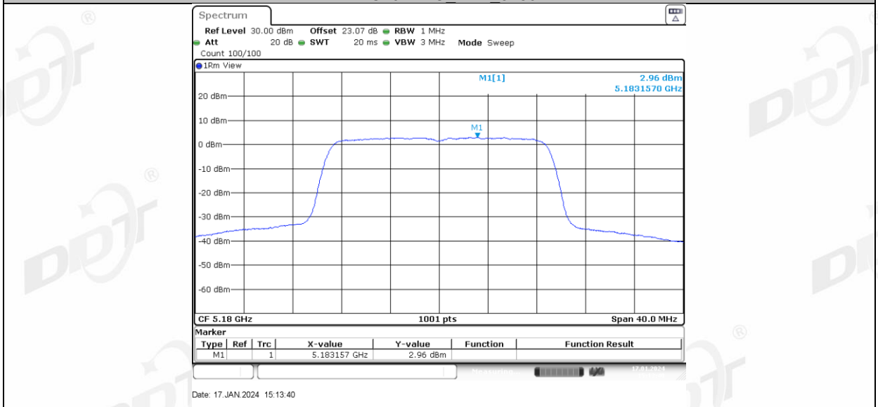
11AC20MIMO Ant2 5180
