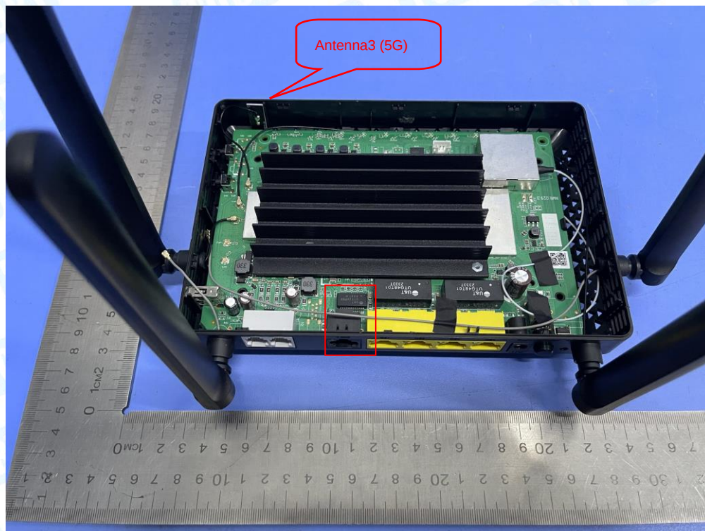
Photo 10 Internal of EUT-NP3081GC
