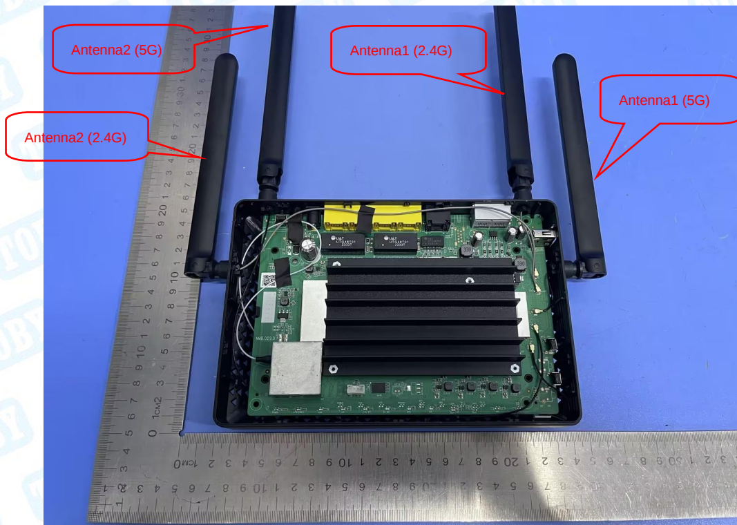
Photo 10 Internal of EUT-NP3081GC
