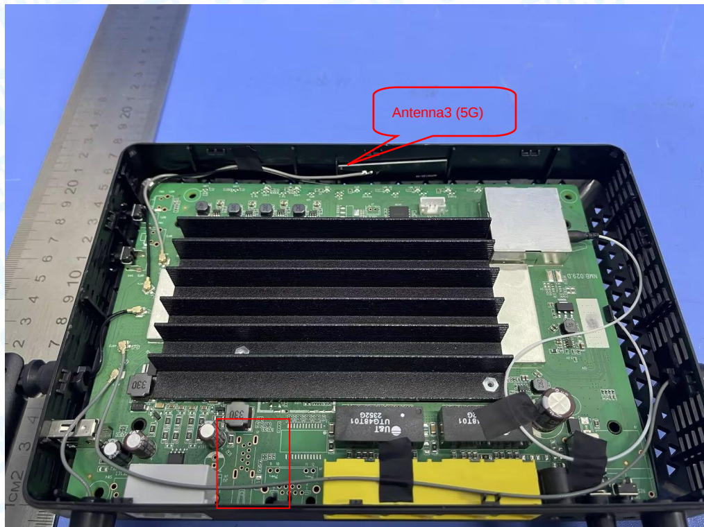
Photo 12 Appearance of Antenna
